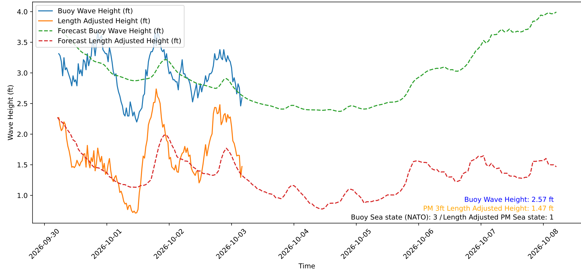
Wave Heights over Time for Green Beach at 2026-10-03 05:01:11
