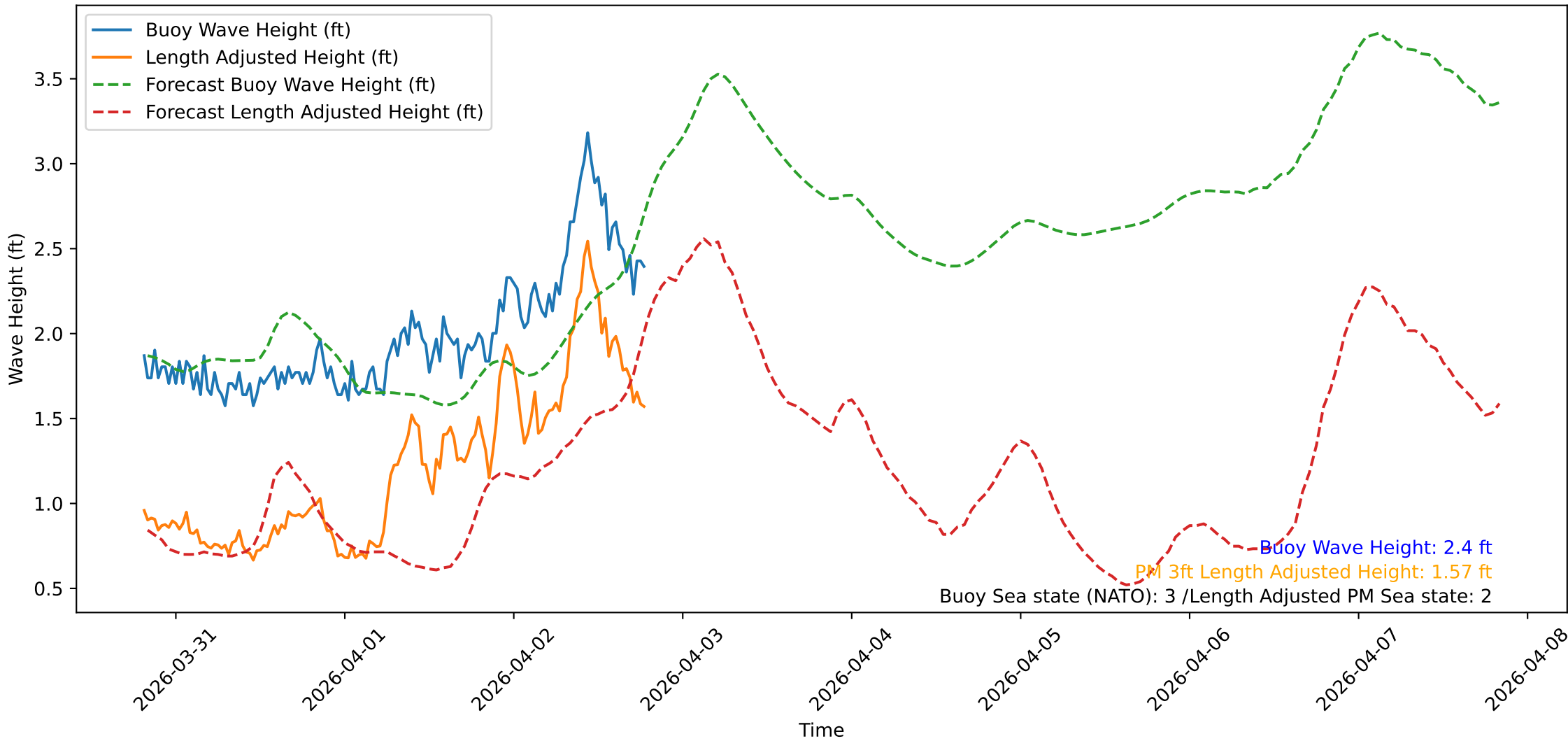
Wave Heights over Time for Oceanside Harbor at 2026-04-02 19:30:31
