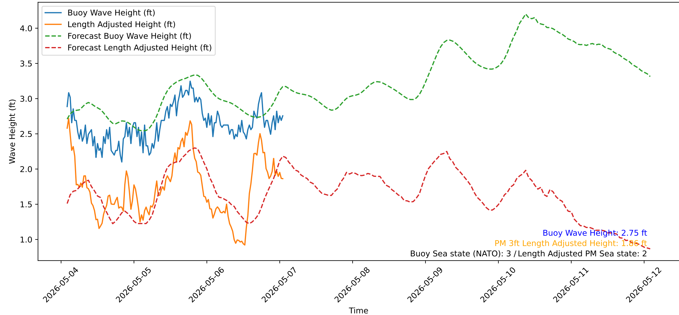
Wave Heights over Time for Oceanside Harbor at 2026-05-07 01:50:31
