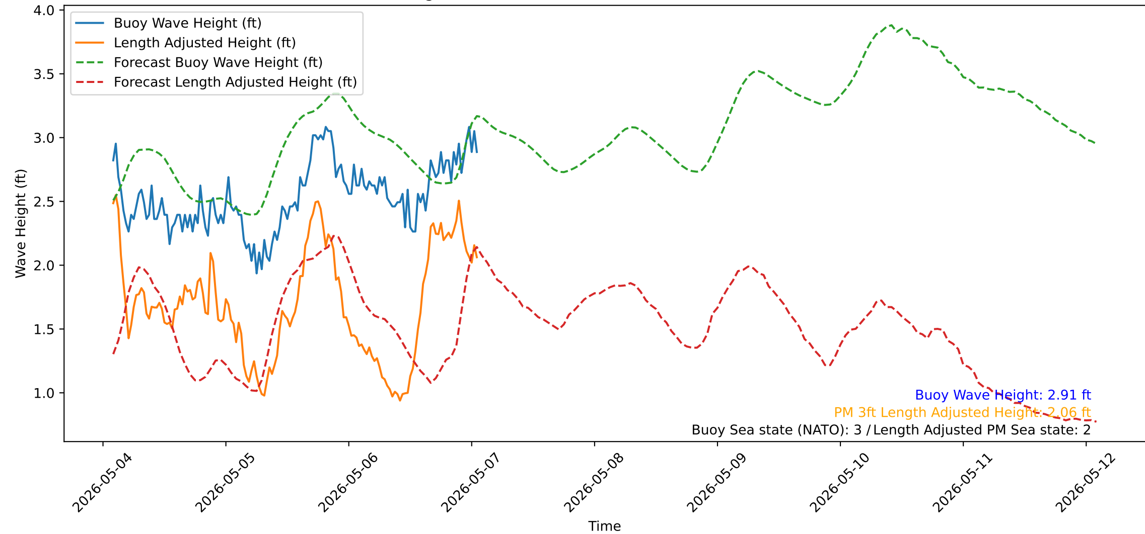
Wave Heights over Time for Red Beach at 2026-05-07 01:50:52
