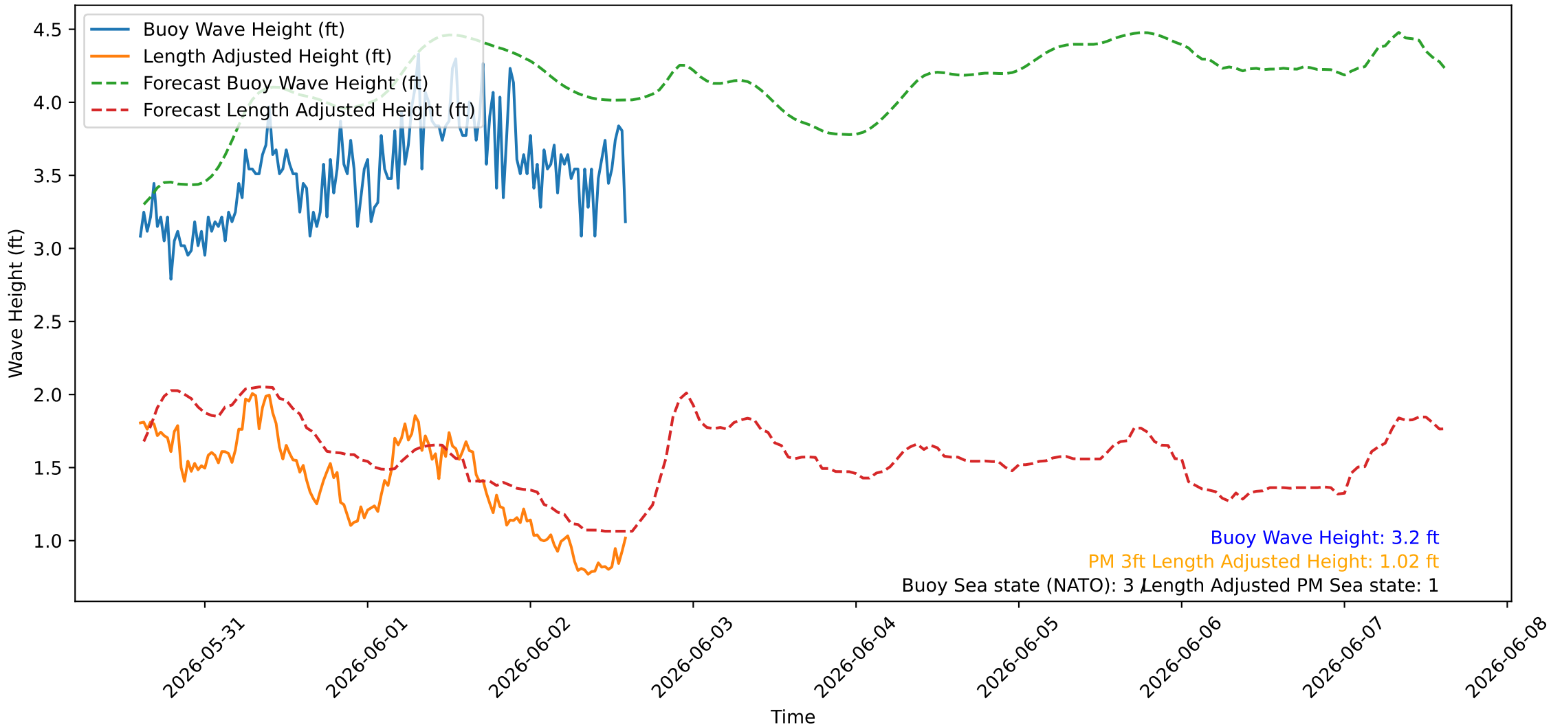
Wave Heights over Time for Green Beach at 2026-06-02 14:41:08
