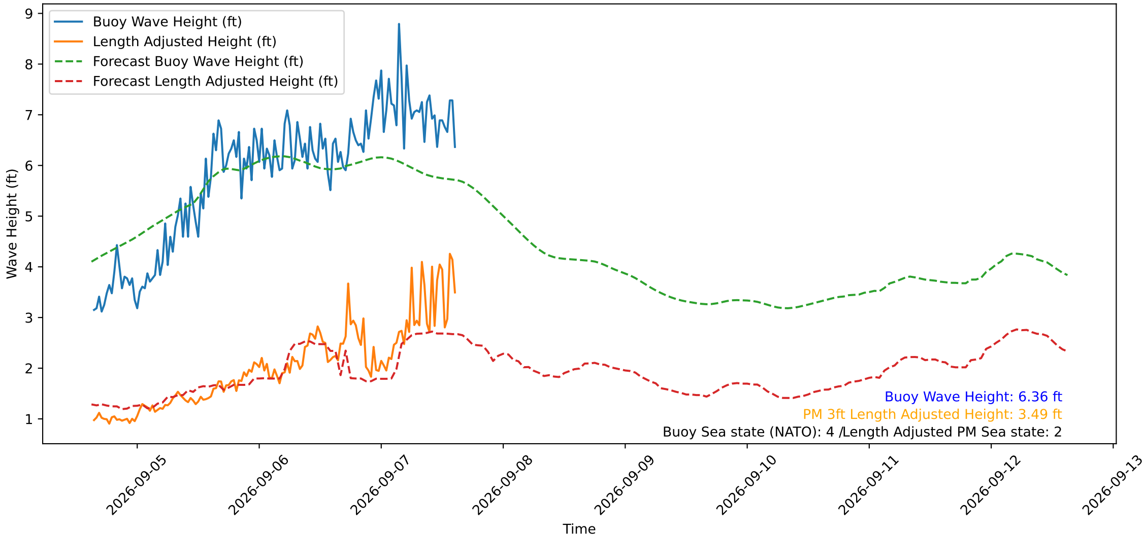
Wave Heights over Time for Green Beach at 2026-09-07 15:11:11
