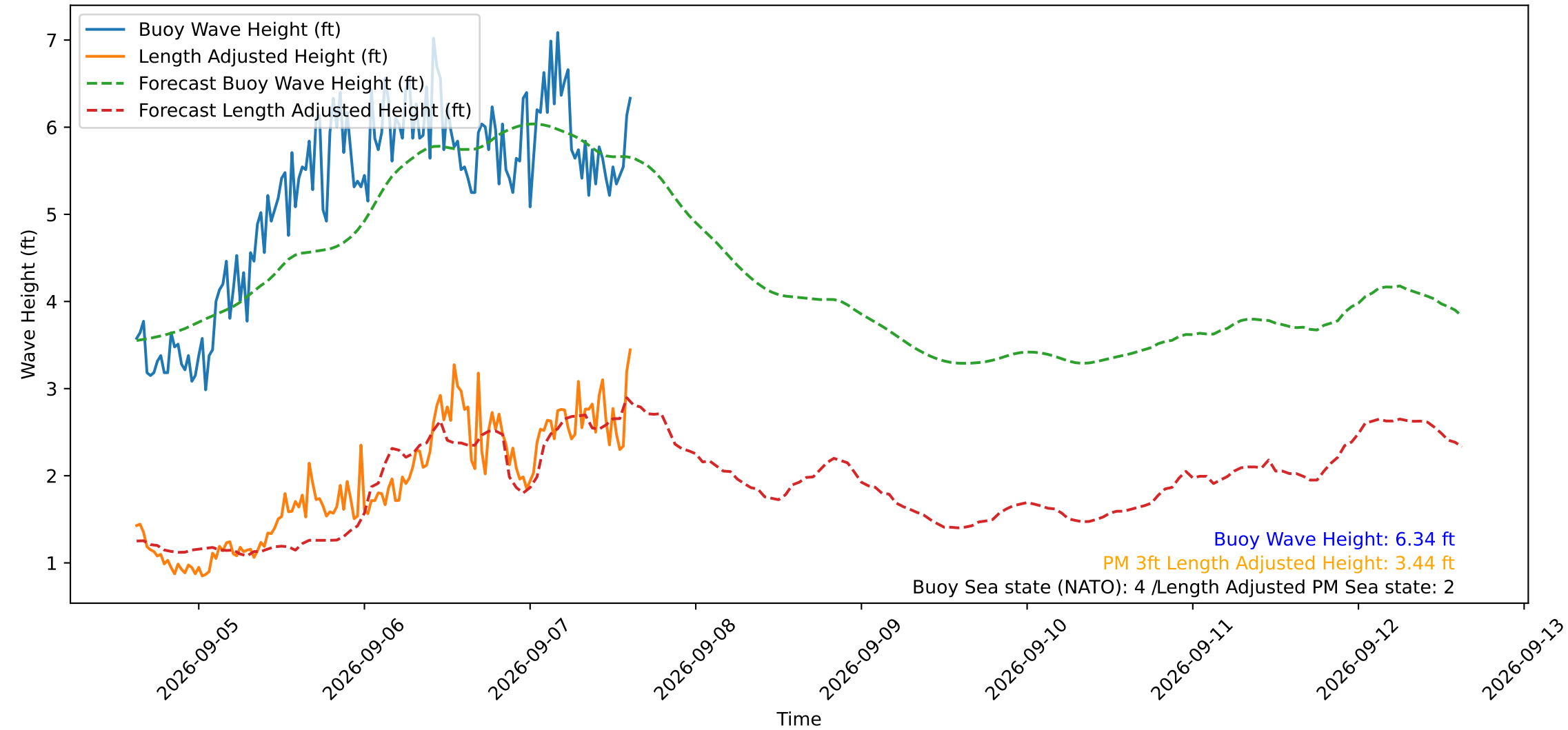
Wave Heights over Time for Oceanside Harbor at 2026-09-07 15:10:30
