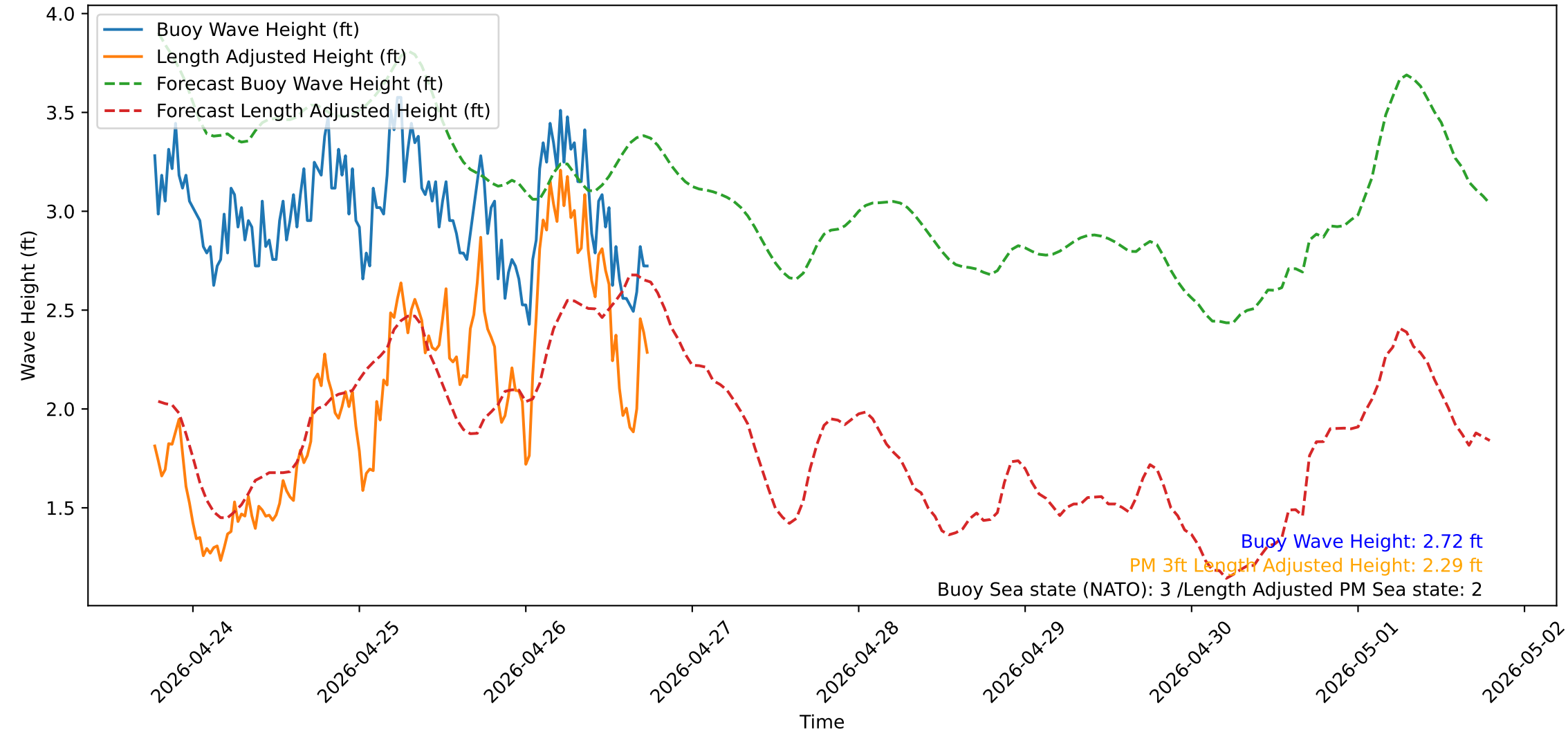
Wave Heights over Time for Green Beach at 2026-04-26 18:31:13
