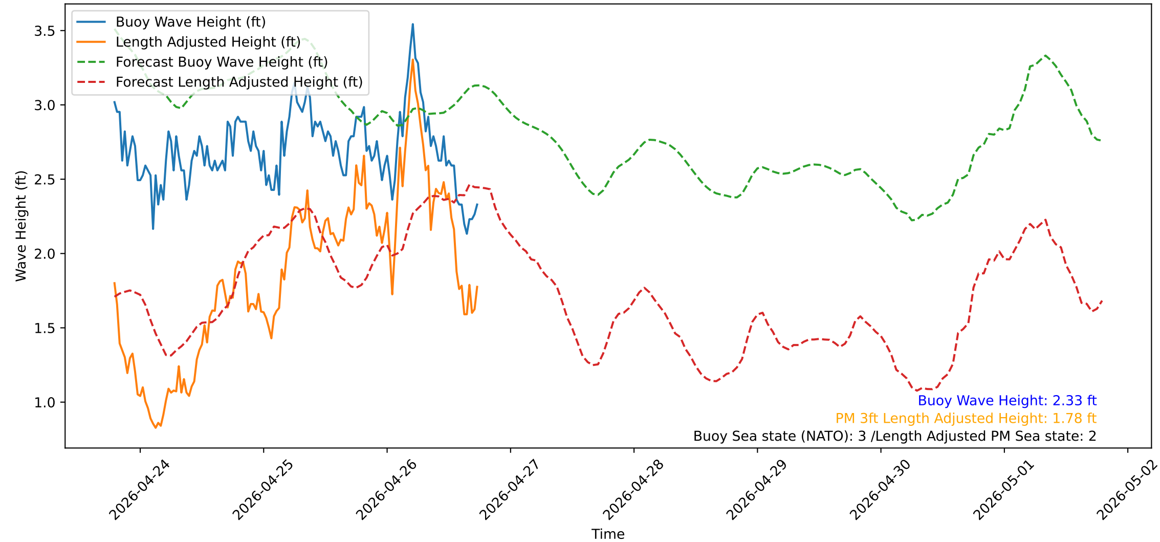
Wave Heights over Time for Red Beach at 2026-04-26 18:30:51
