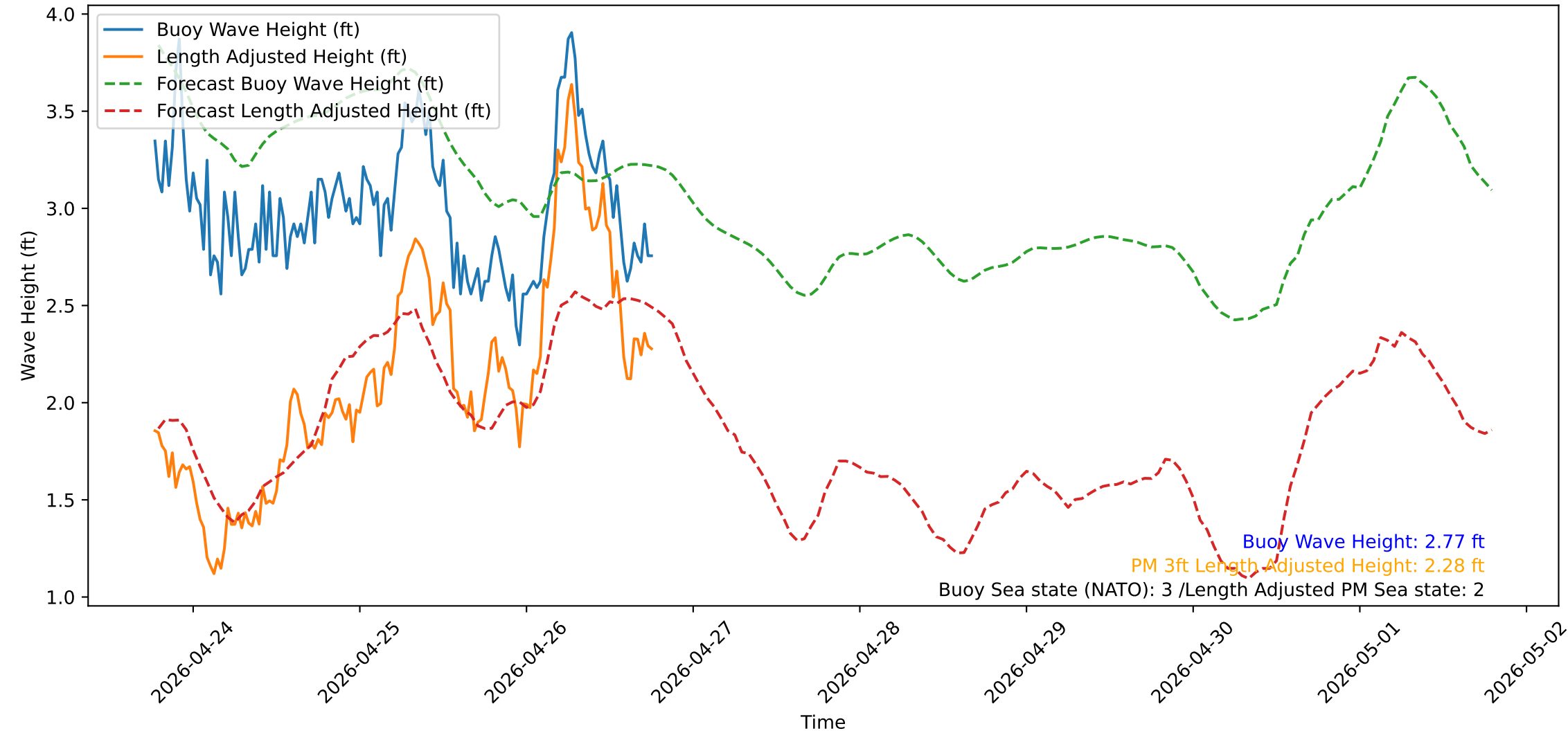
Wave Heights over Time for Oceanside Harbor at 2026-04-26 18:30:31
