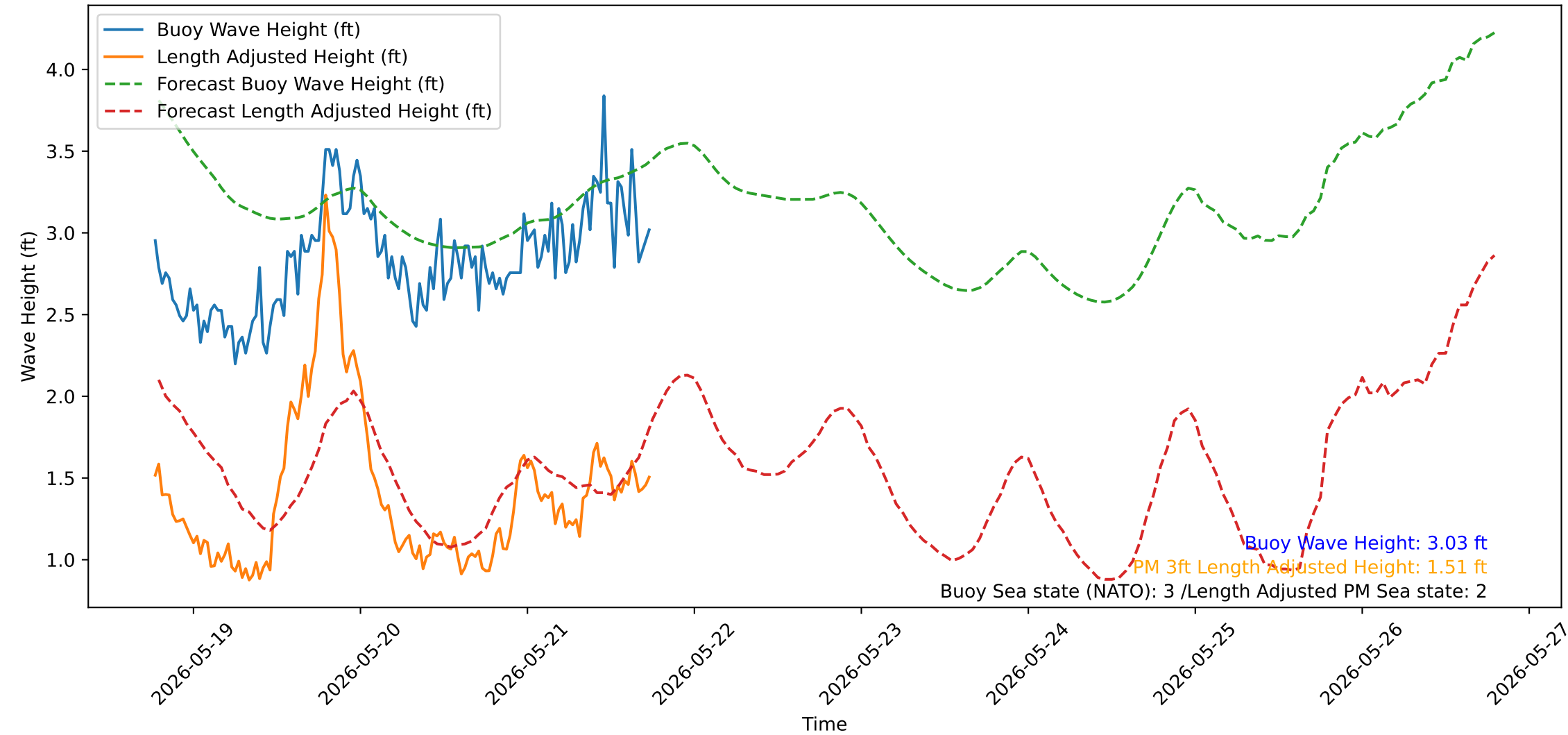
Wave Heights over Time for Oceanside Harbor at 2026-05-21 18:30:31
