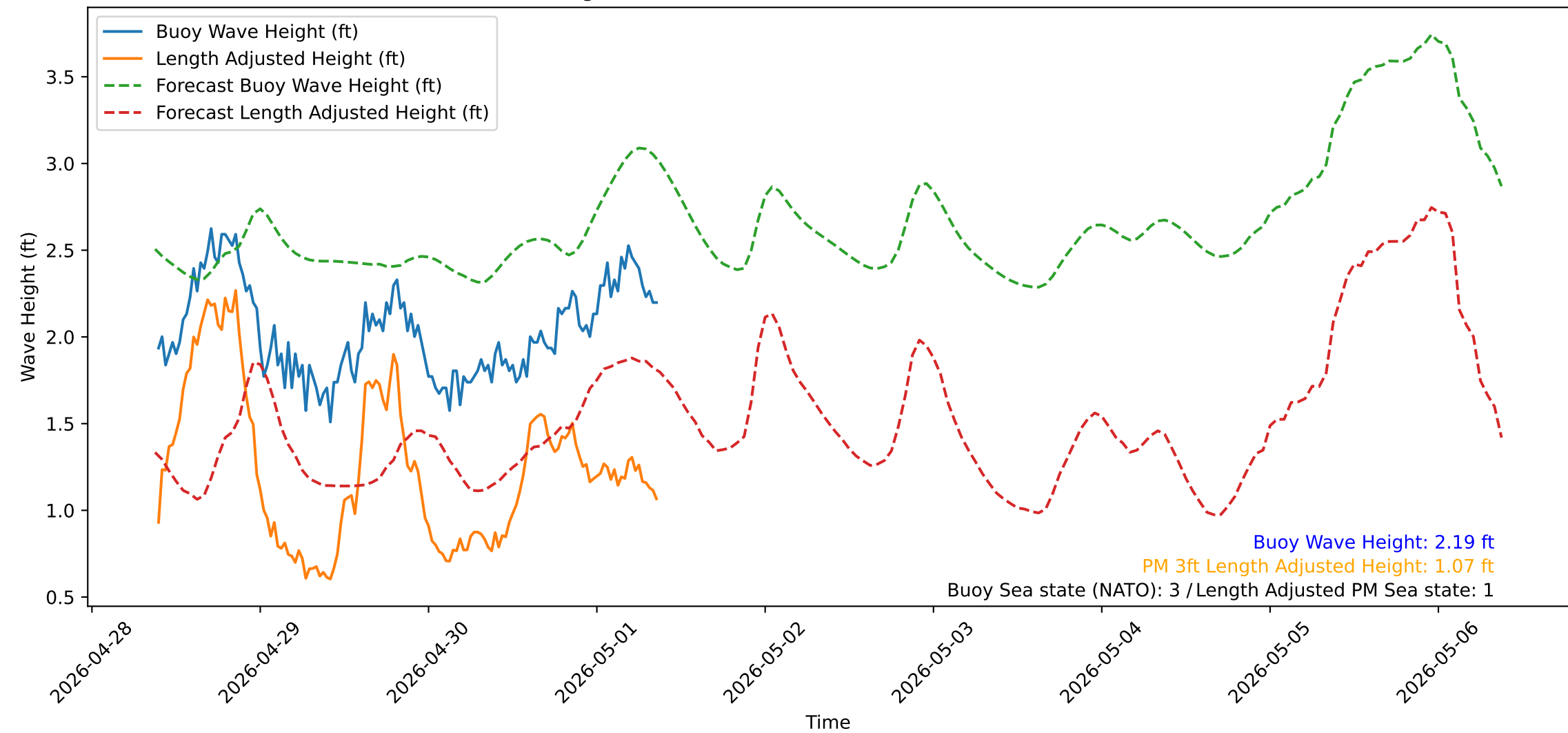
Wave Heights over Time for Red Beach at 2026-05-01 09:10:51
