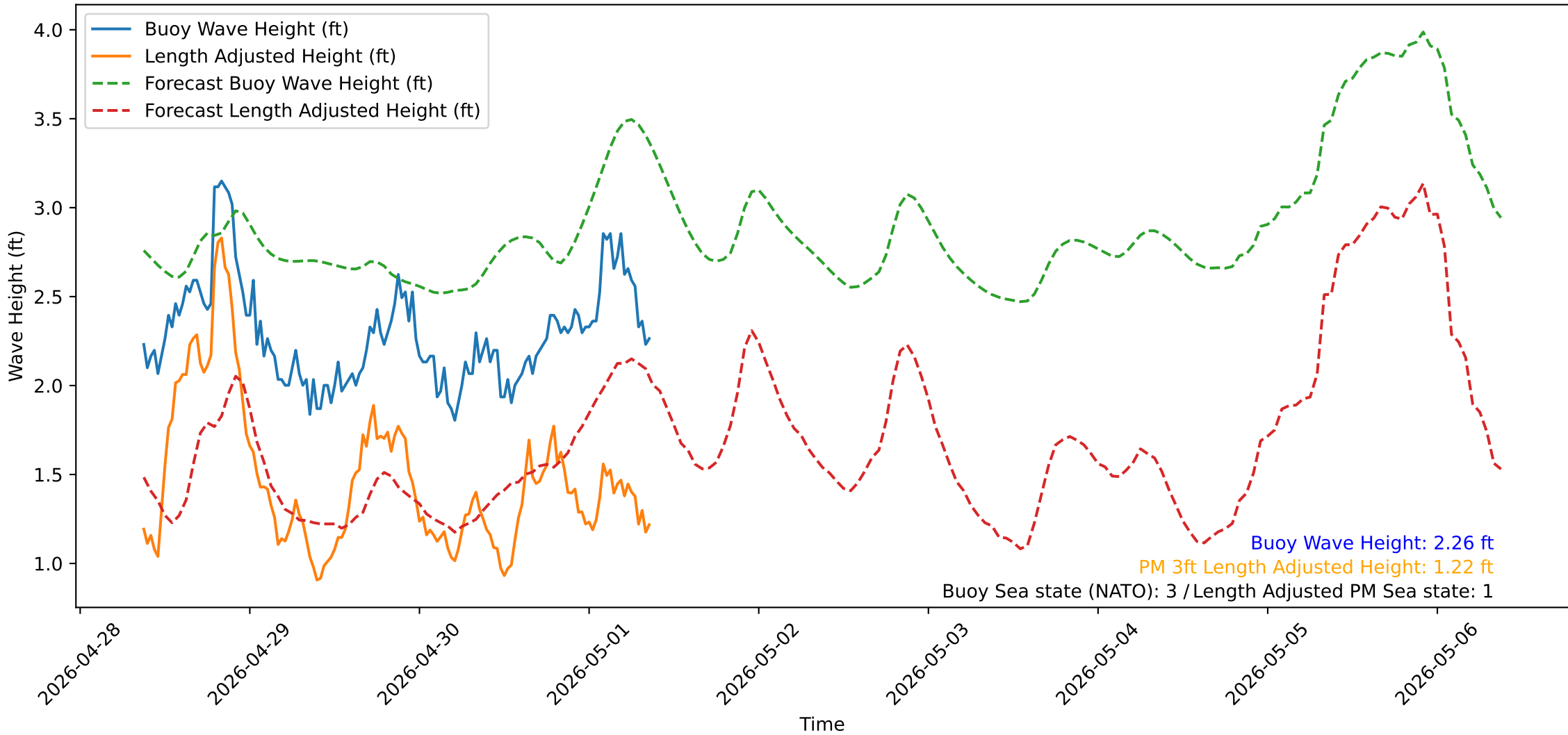
Wave Heights over Time for Green Beach at 2026-05-01 09:11:13
