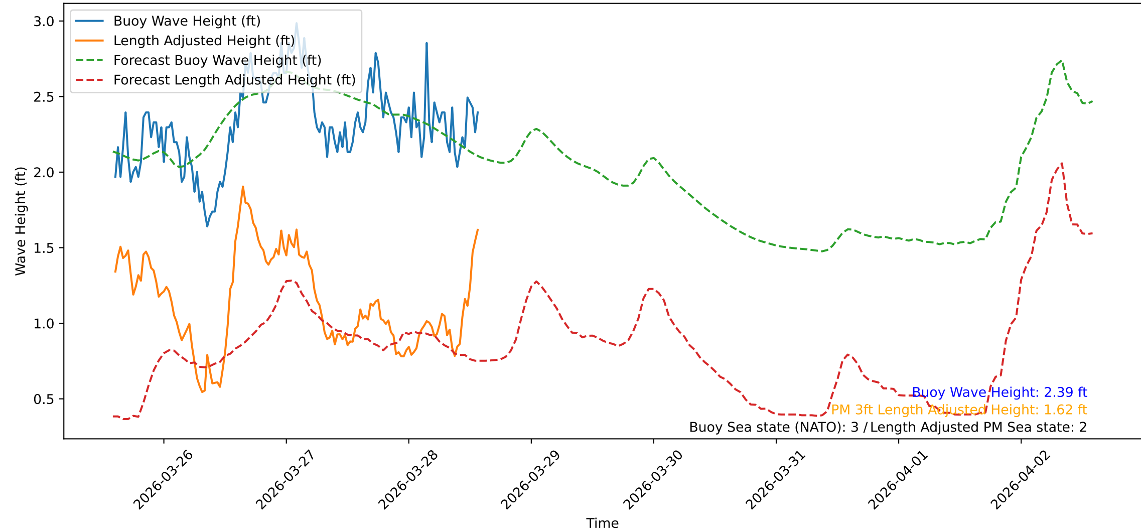
Wave Heights over Time for Red Beach at 2026-03-28 14:10:48
