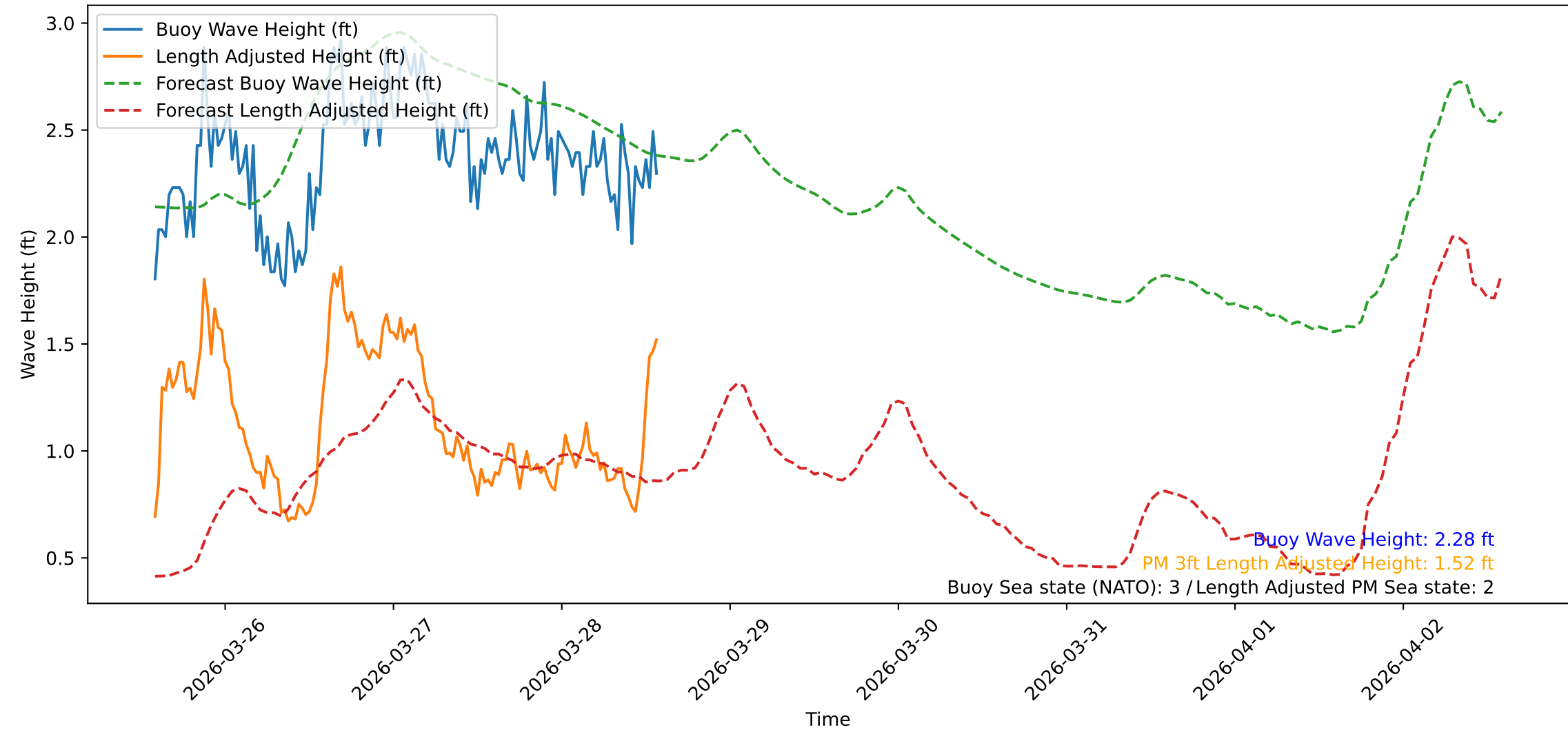
Wave Heights over Time for Oceanside Harbor at 2026-03-28 14:10:32
