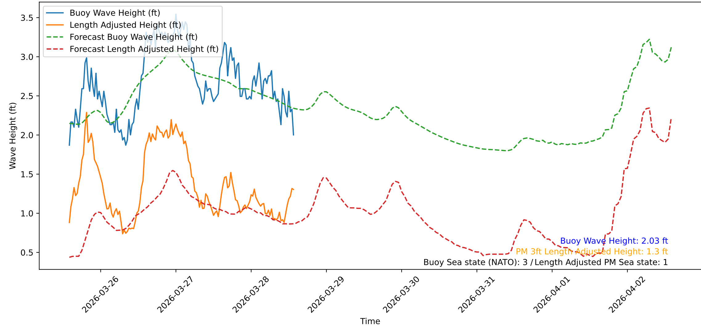
Wave Heights over Time for Green Beach at 2026-03-28 14:11:10
