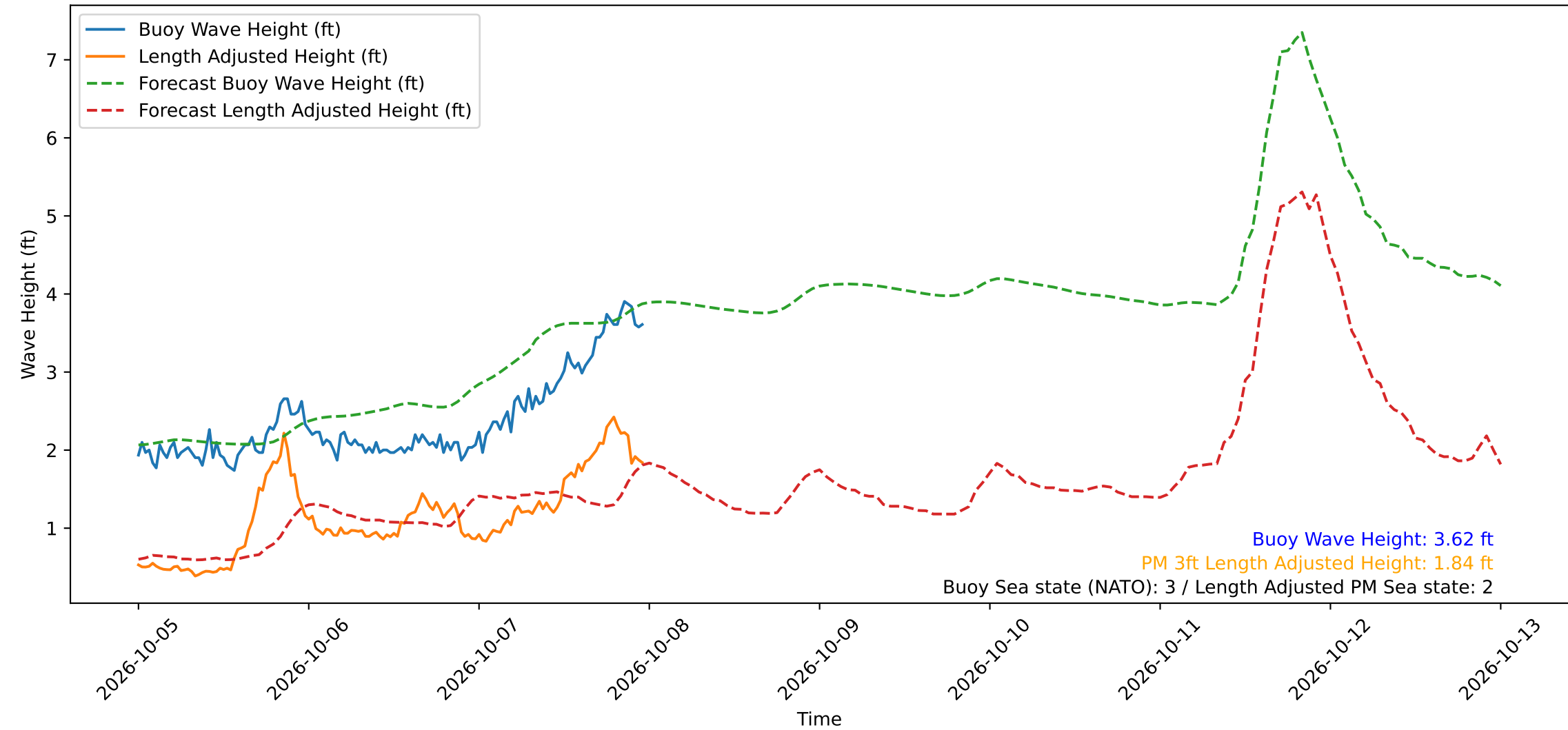
Wave Heights over Time for Red Beach at 2026-10-07 23:40:49
