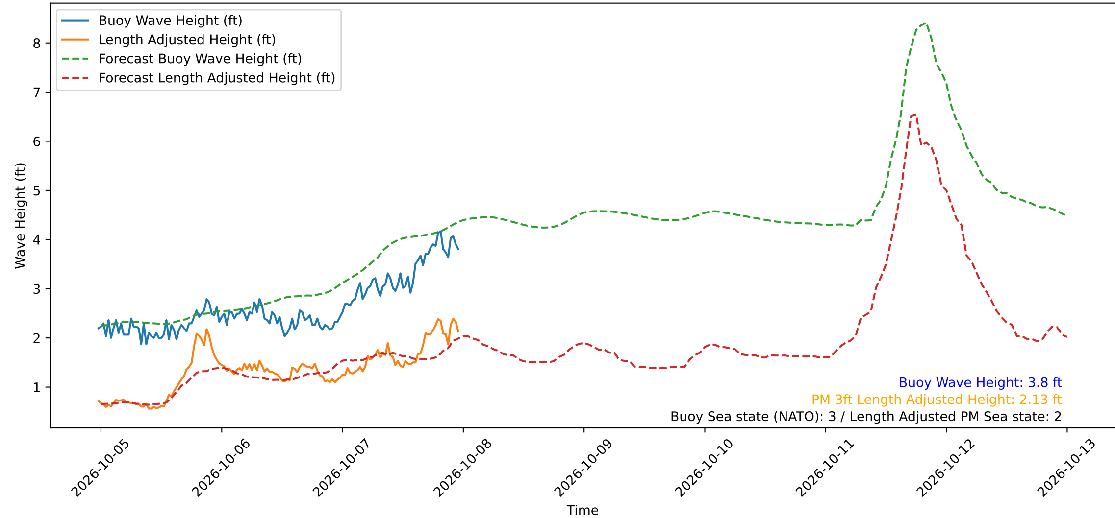
Wave Heights over Time for Oceanside Harbor at 2026-10-07 23:40:29
