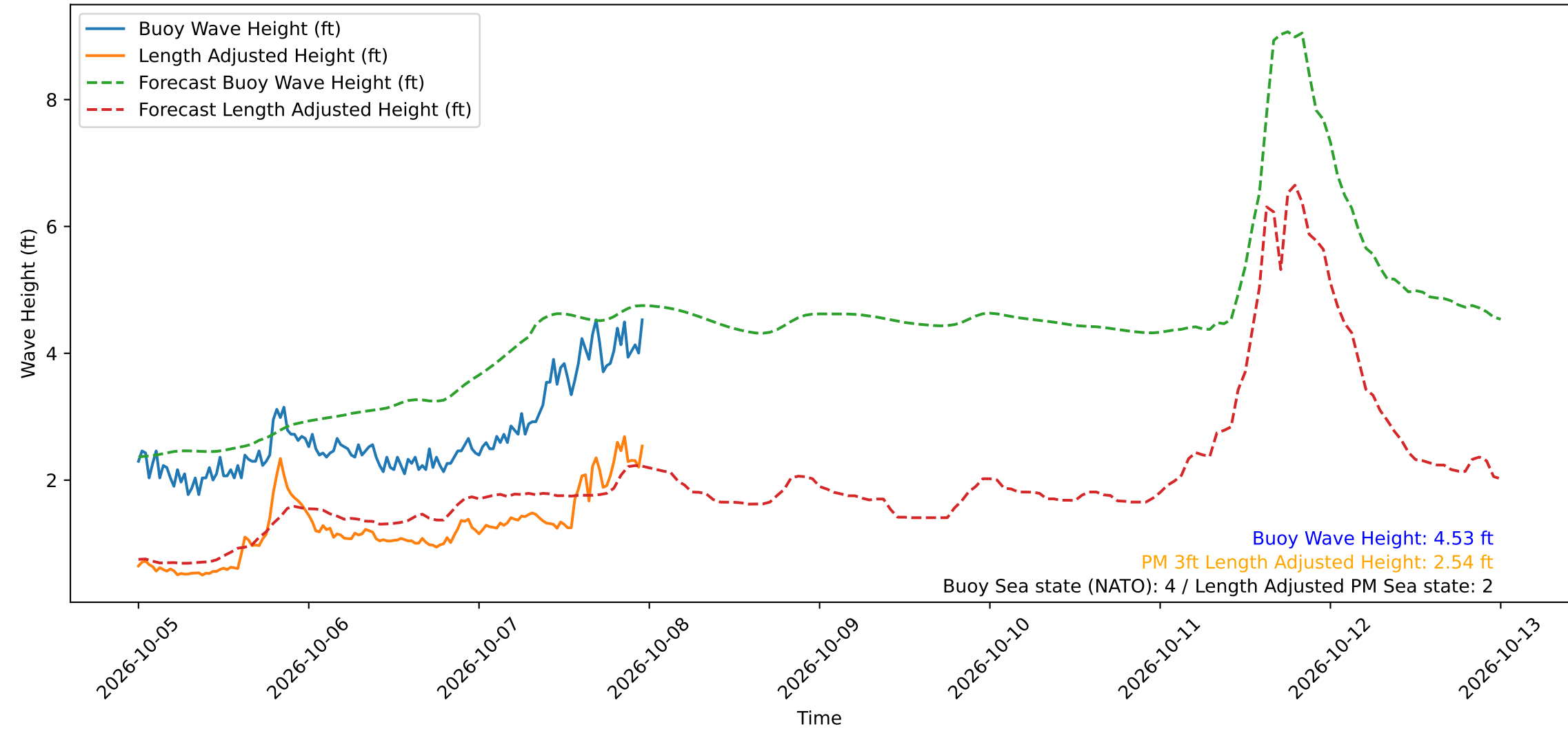
Wave Heights over Time for Green Beach at 2026-10-07 23:41:12
