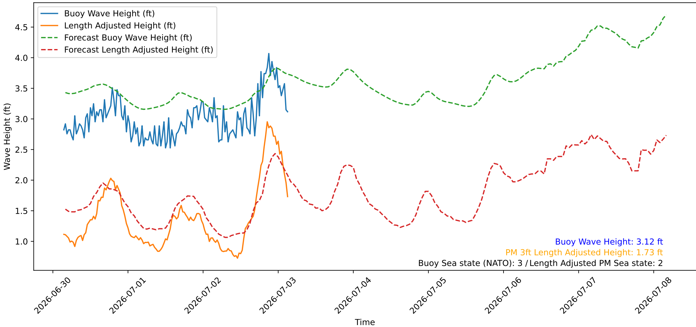
Wave Heights over Time for Green Beach at 2026-07-03 03:41:09
