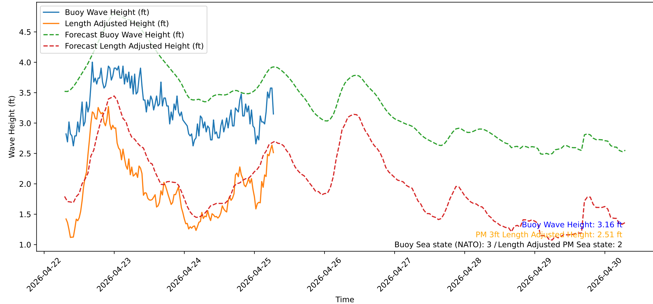
Wave Heights over Time for Green Beach at 2026-04-25 07:21:14
