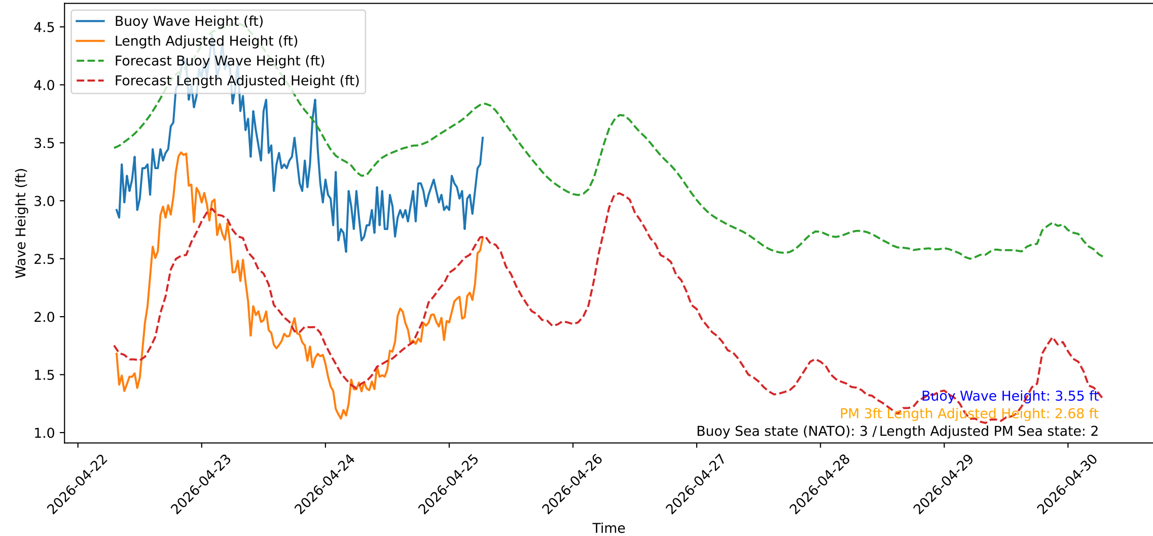
Wave Heights over Time for Oceanside Harbor at 2026-04-25 07:20:32
