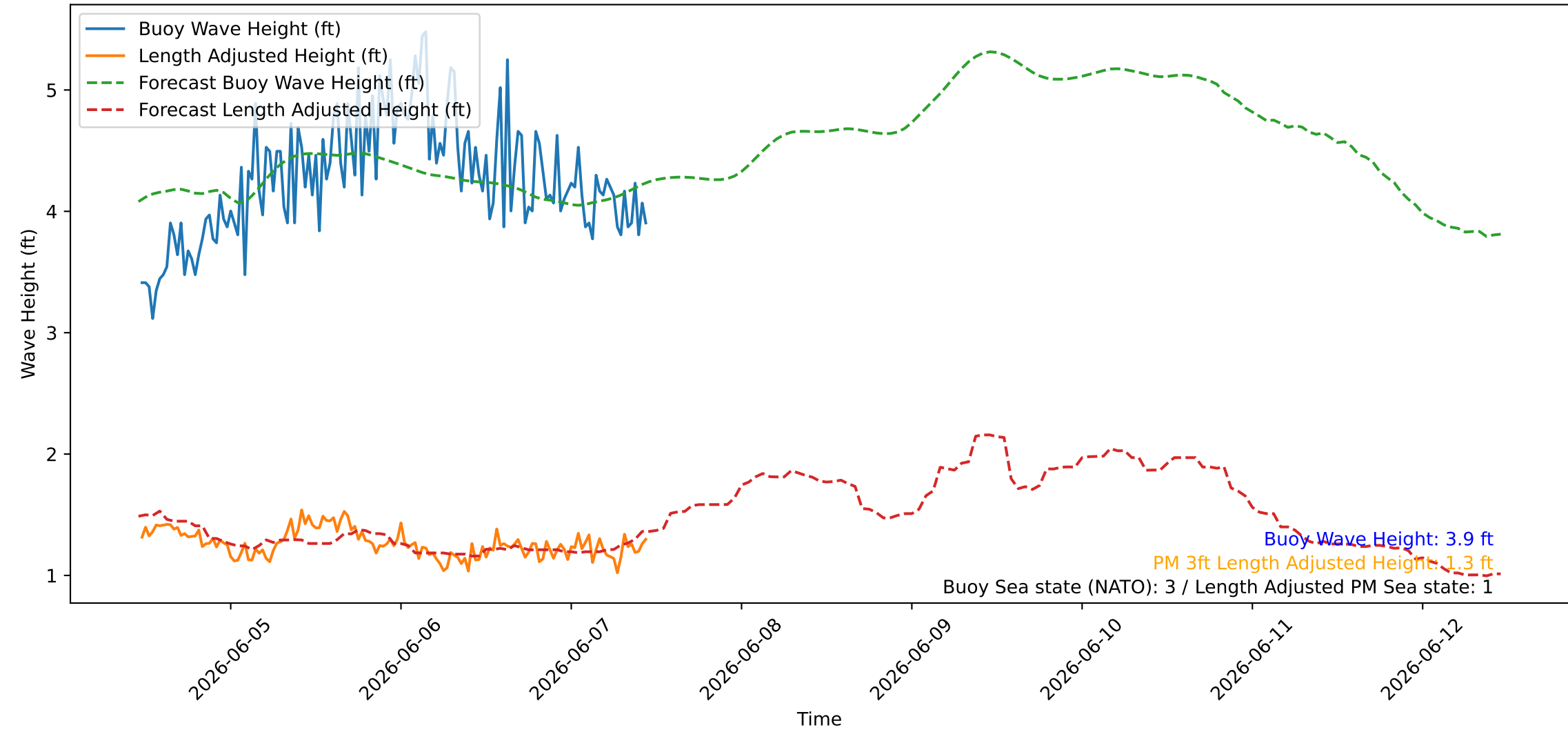
Wave Heights over Time for Oceanside Harbor at 2026-06-07 11:20:26
