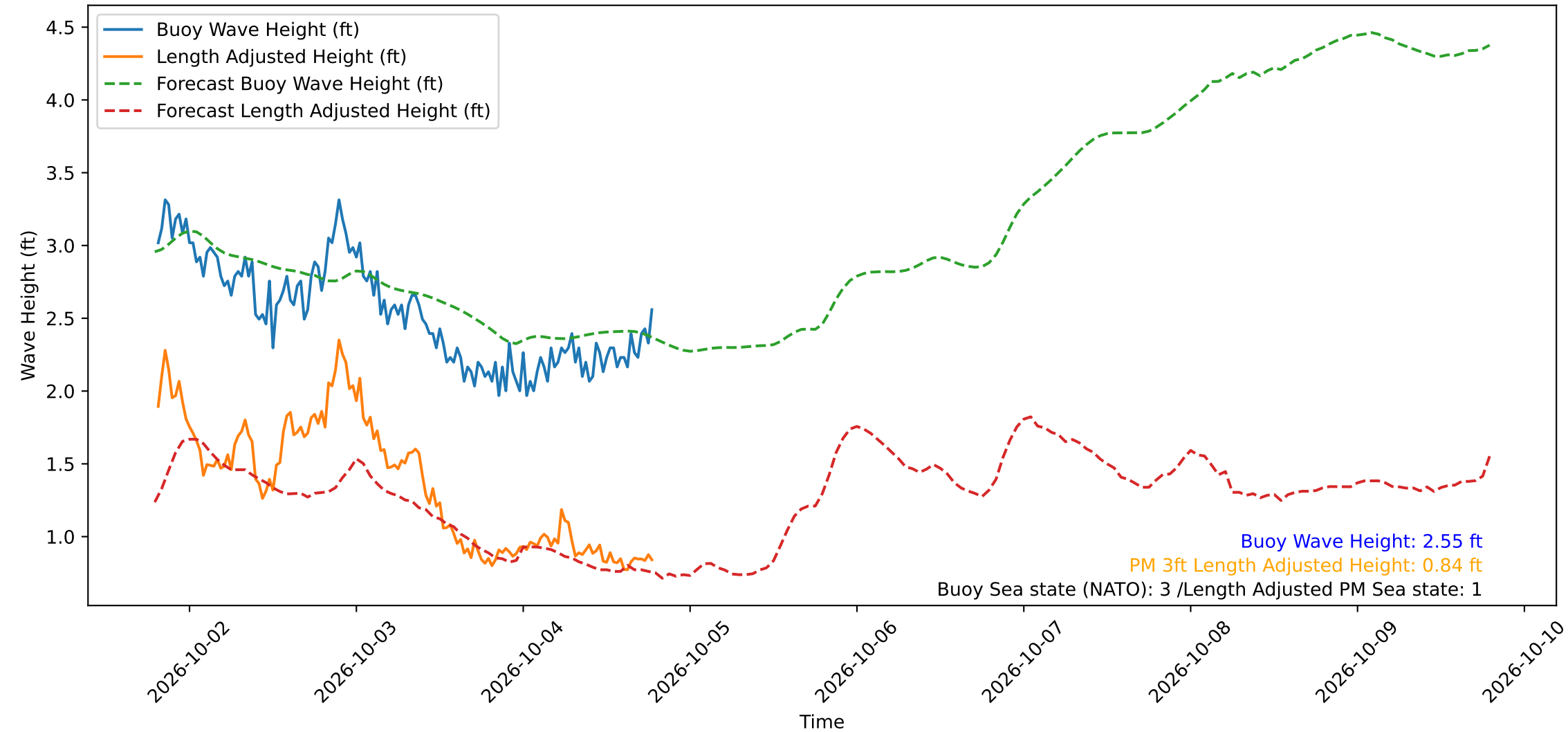
Wave Heights over Time for Oceanside Harbor at 2026-10-04 19:20:29
