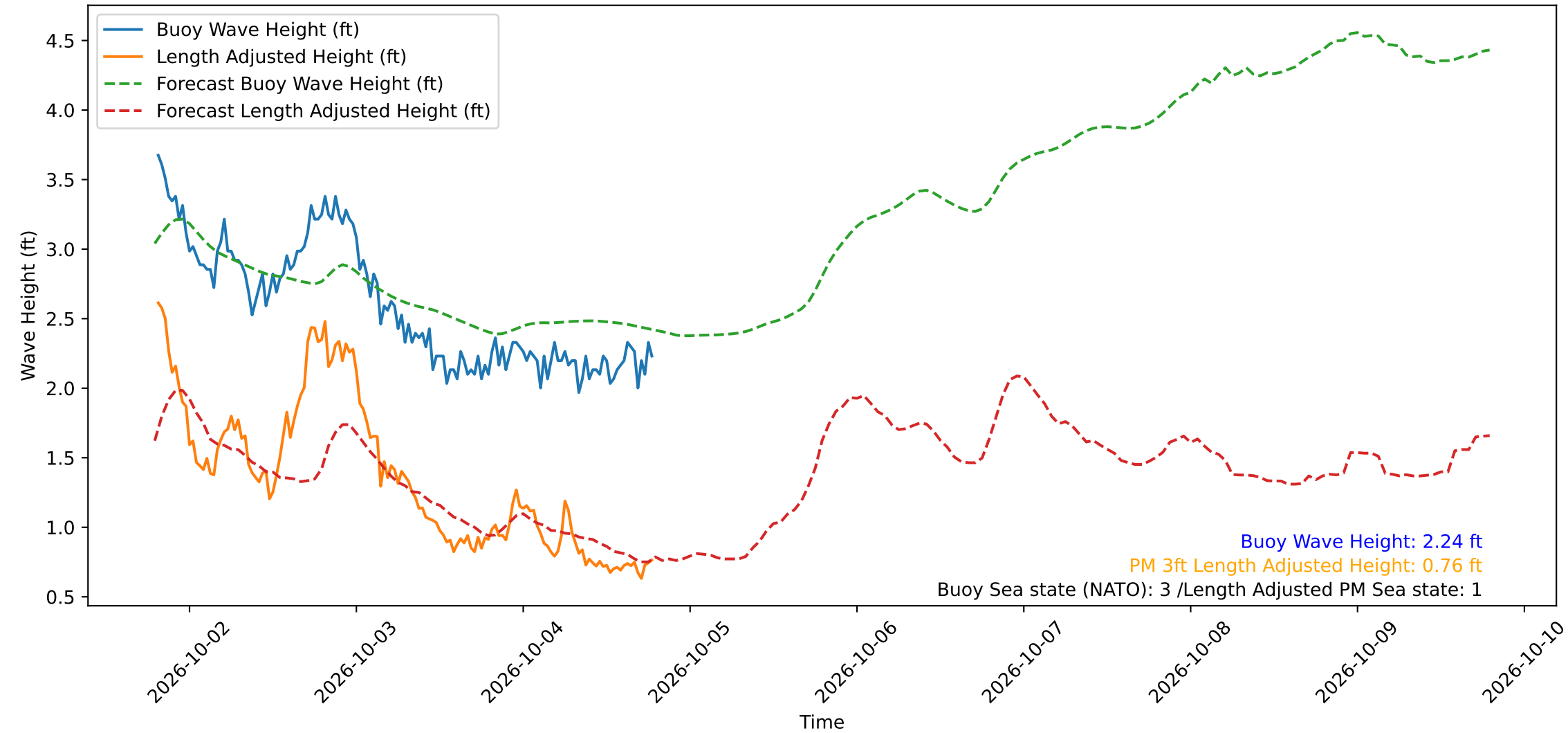
Wave Heights over Time for Green Beach at 2026-10-04 19:21:14
