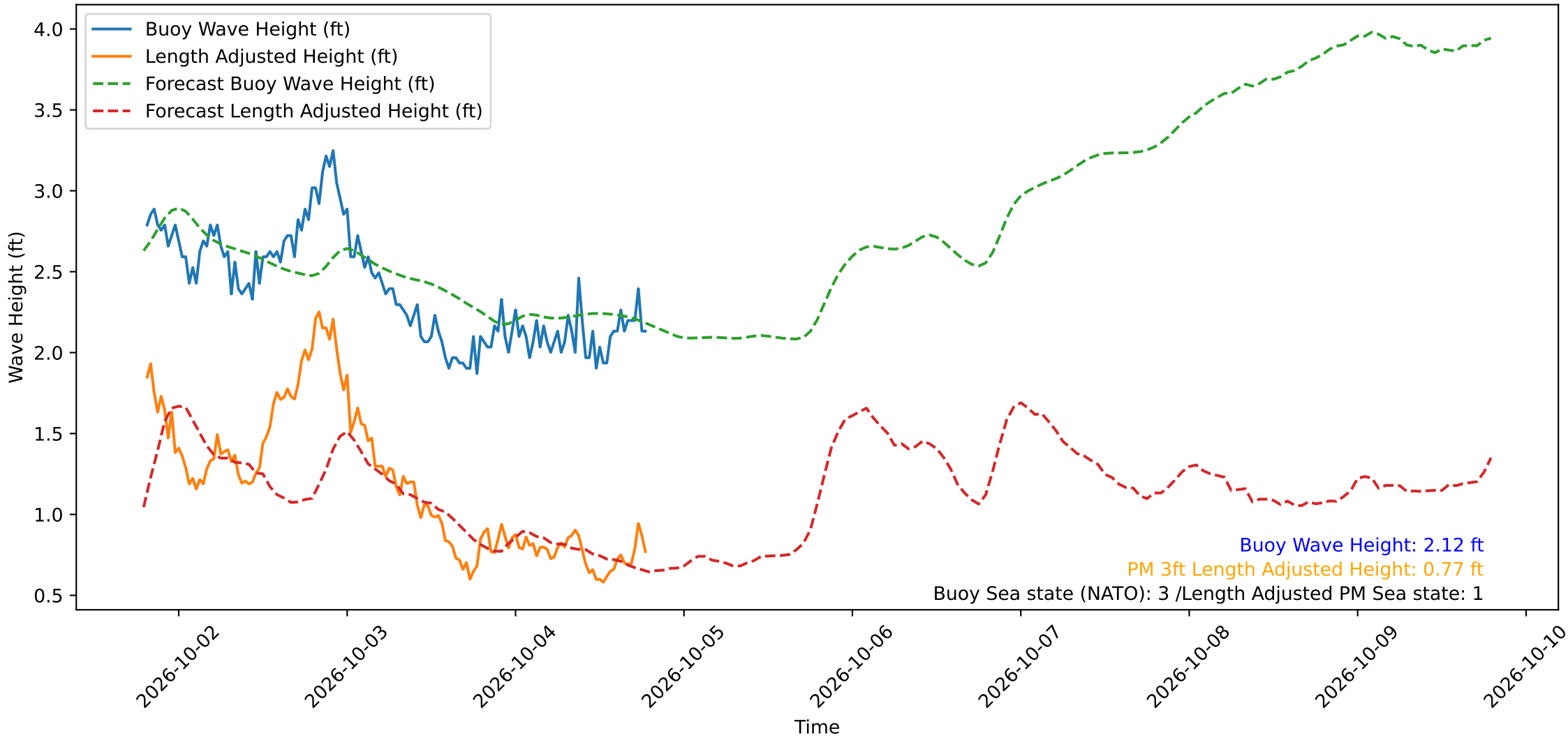
Wave Heights over Time for Red Beach at 2026-10-04 19:20:50
