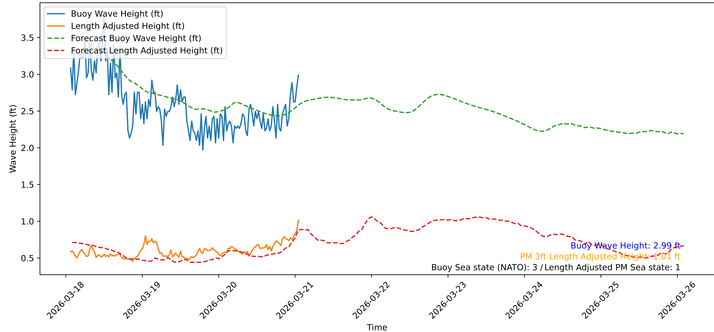
Wave Heights over Time for Oceanside Harbor at 2026-03-21 01:40:32
