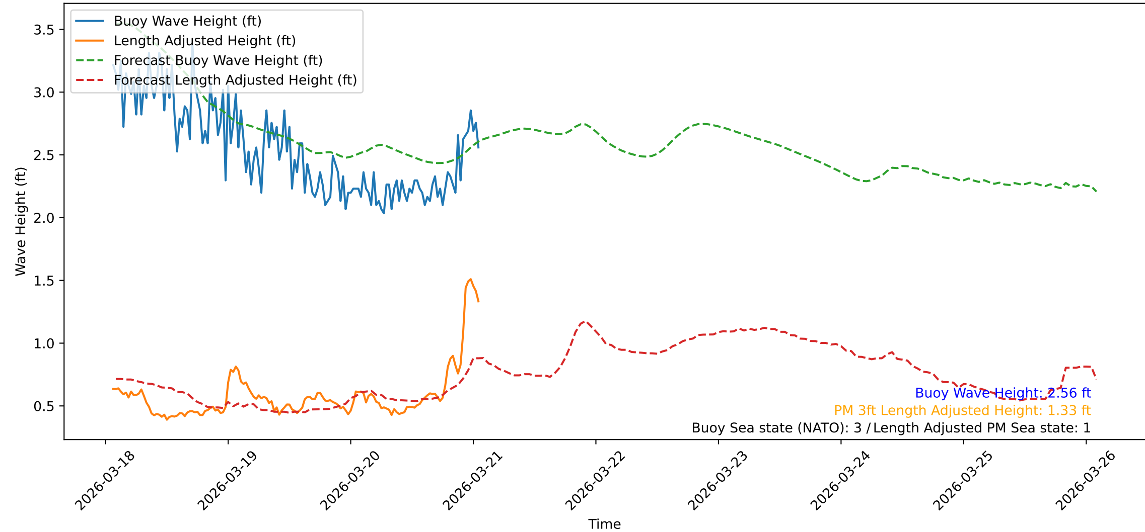
Wave Heights over Time for Green Beach at 2026-03-21 01:41:11
