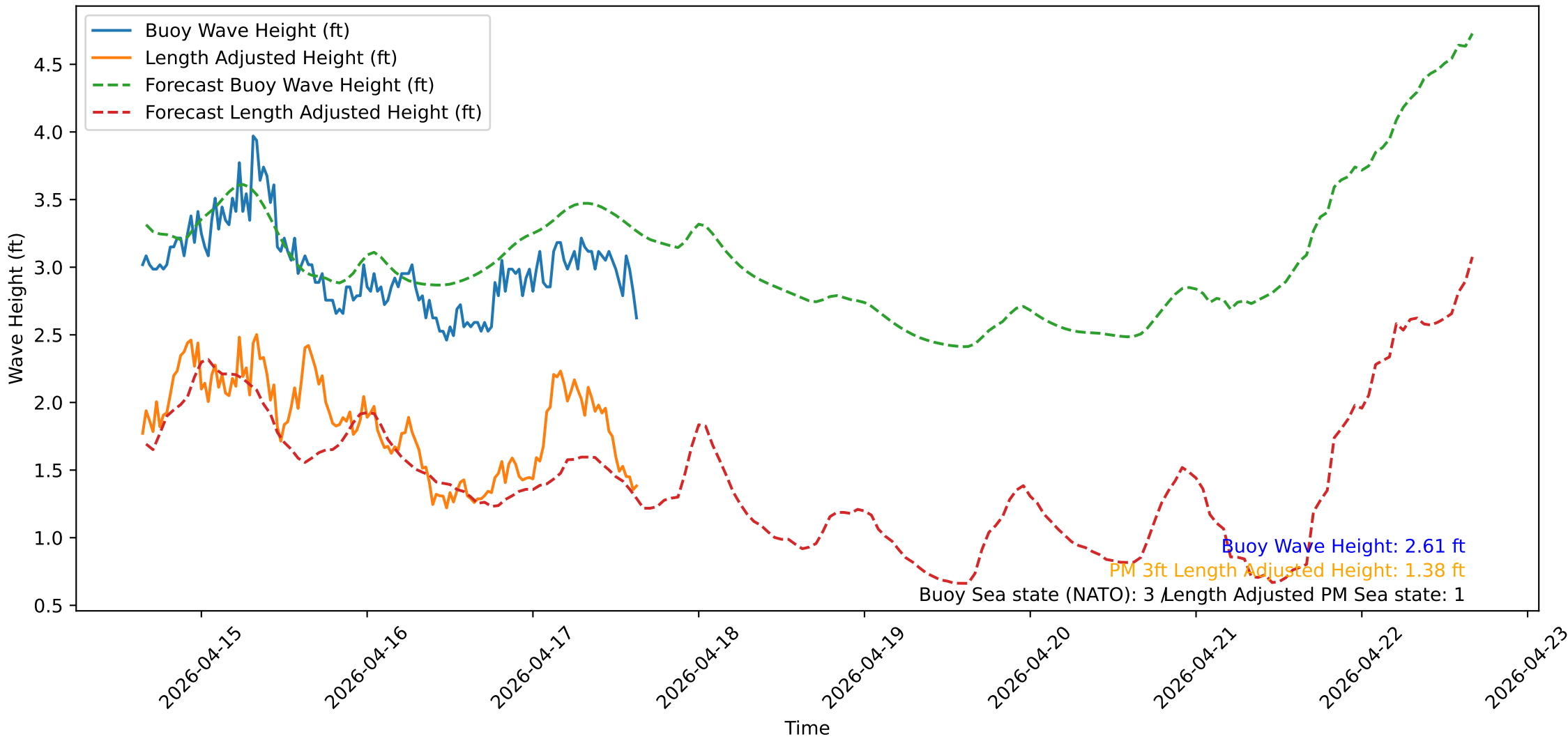
Wave Heights over Time for Green Beach at 2026-04-17 15:41:13
