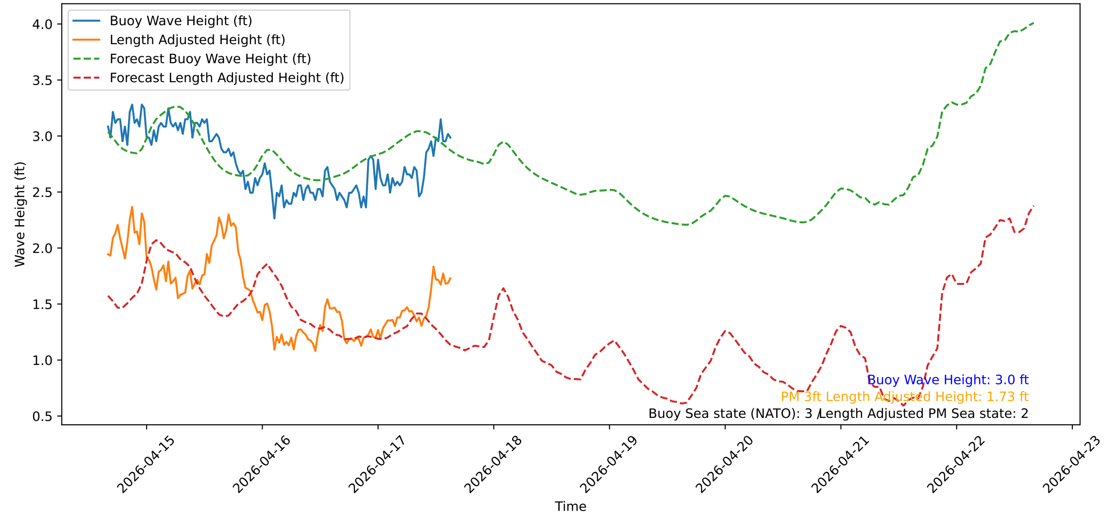
Wave Heights over Time for Red Beach at 2026-04-17 15:40:50
