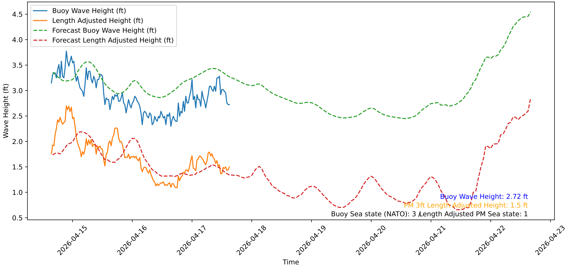
Wave Heights over Time for Oceanside Harbor at 2026-04-17 15:40:31
