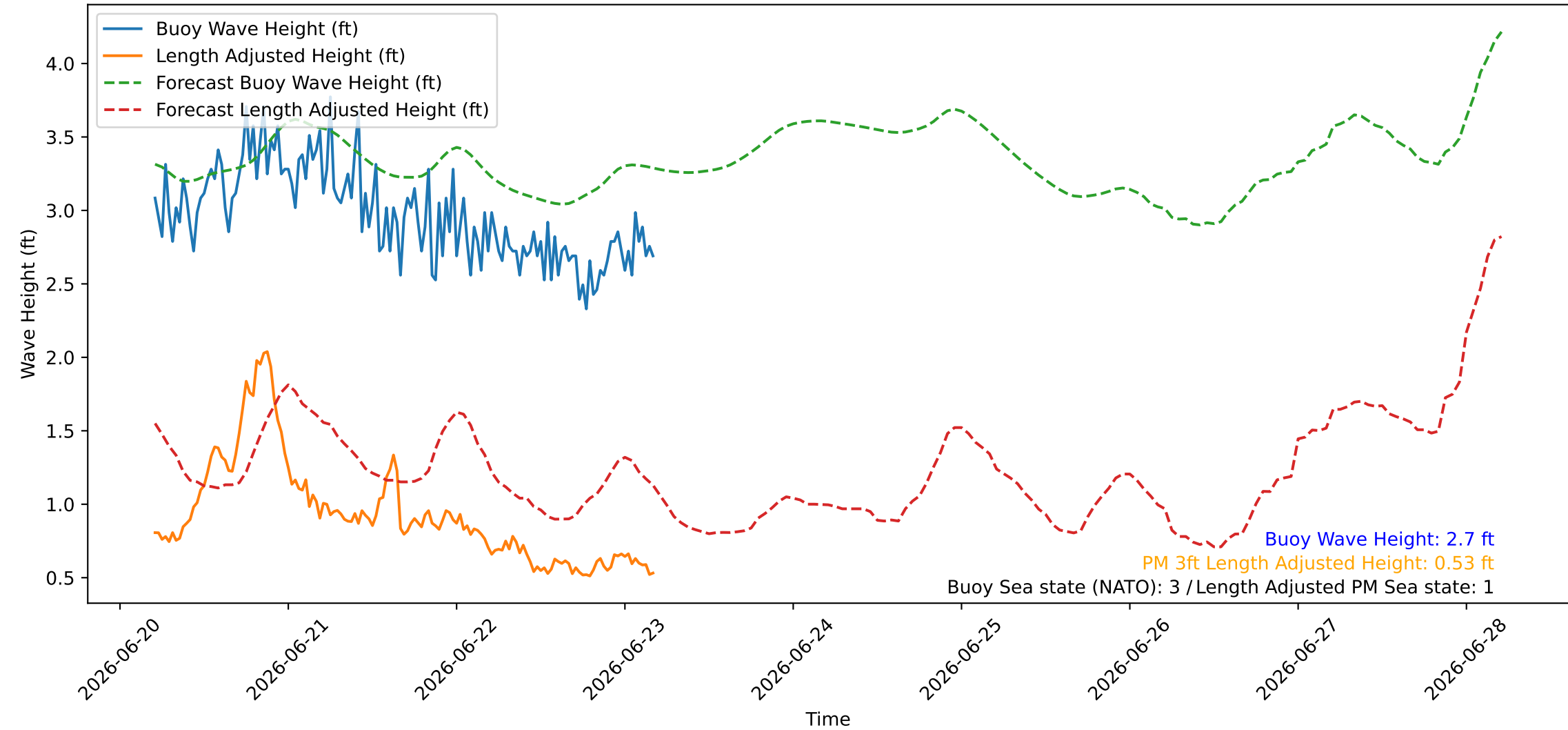
Wave Heights over Time for Red Beach at 2026-06-23 04:50:46
