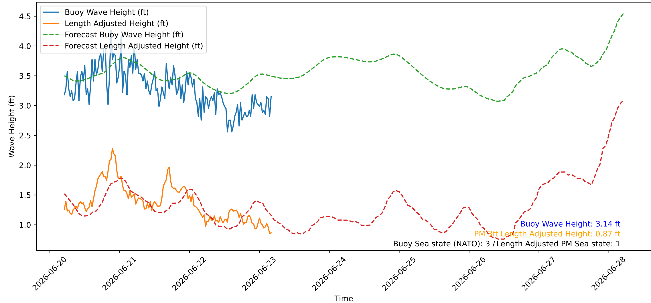
Wave Heights over Time for Oceanside Harbor at 2026-06-23 04:50:26
