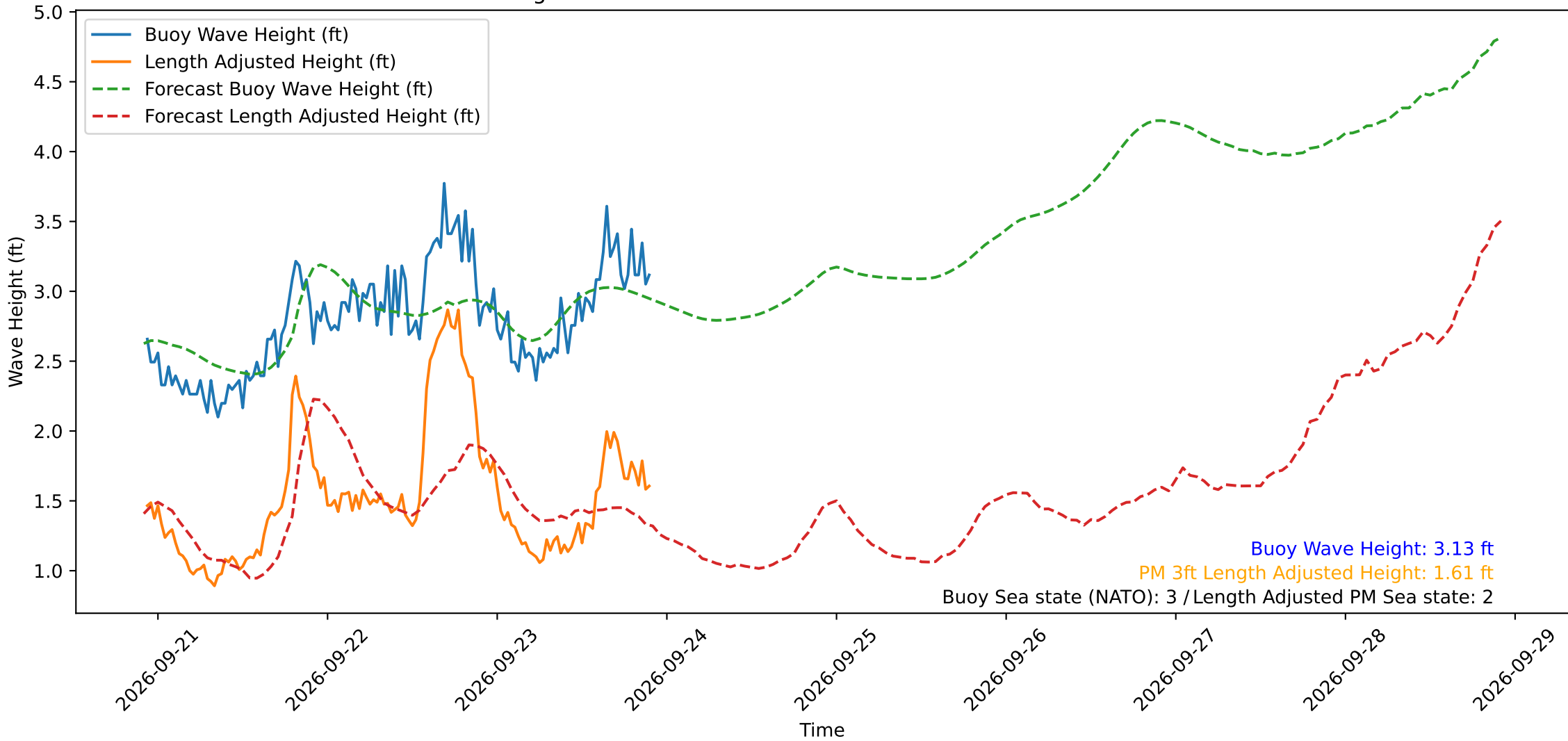
Wave Heights over Time for Oceanside Harbor at 2026-09-23 22:20:29
