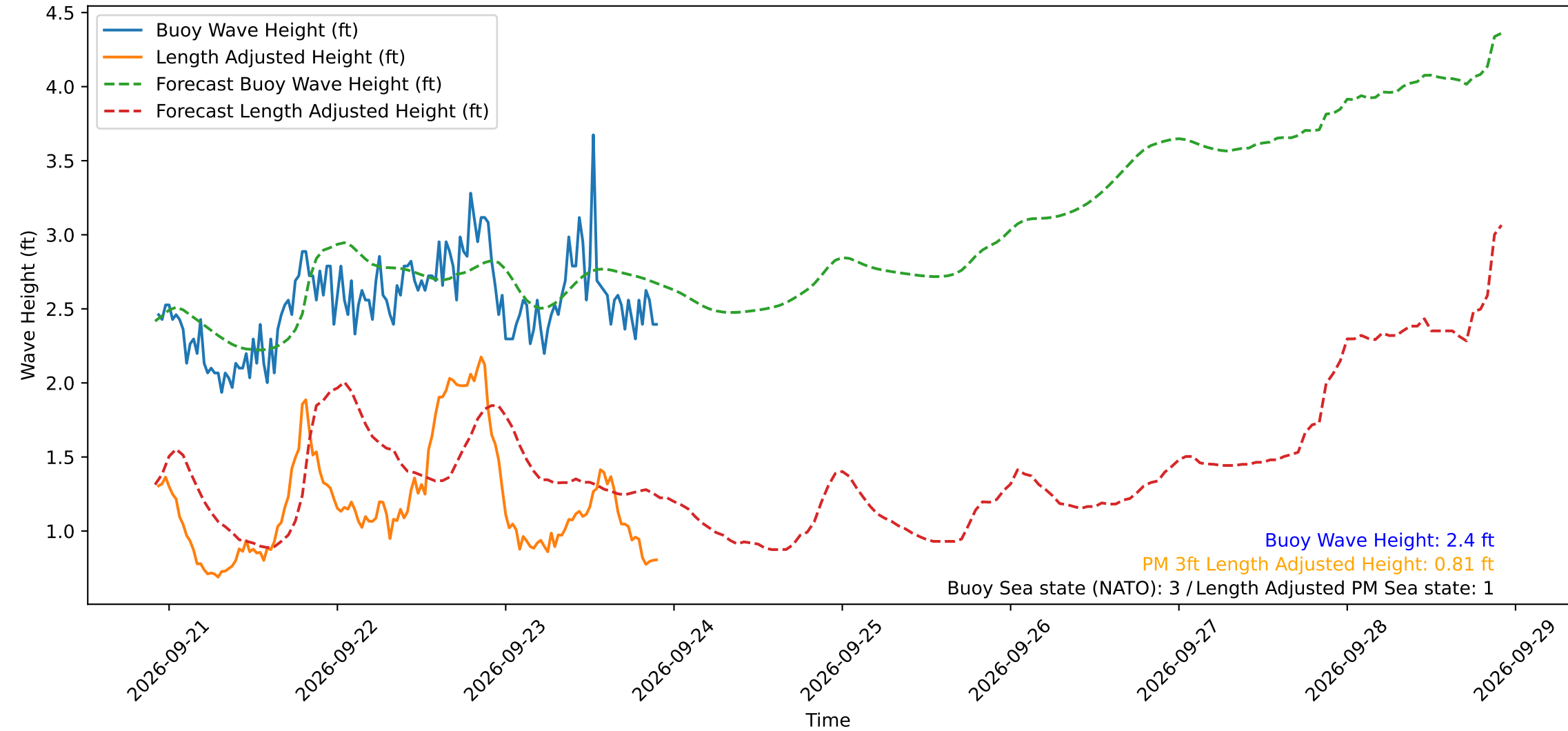
Wave Heights over Time for Red Beach at 2026-09-23 22:20:50
