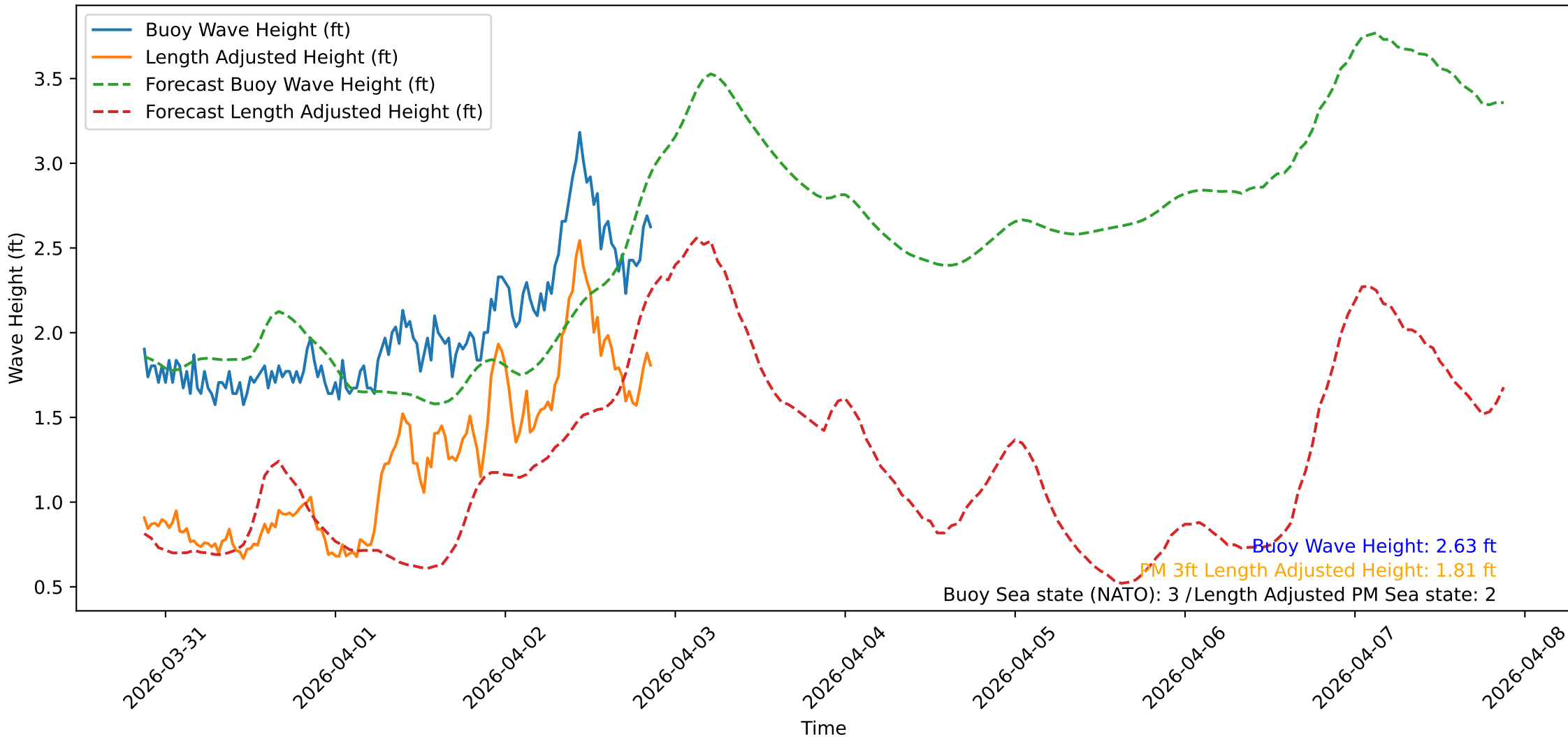
Wave Heights over Time for Oceanside Harbor at 2026-04-02 21:00:31
