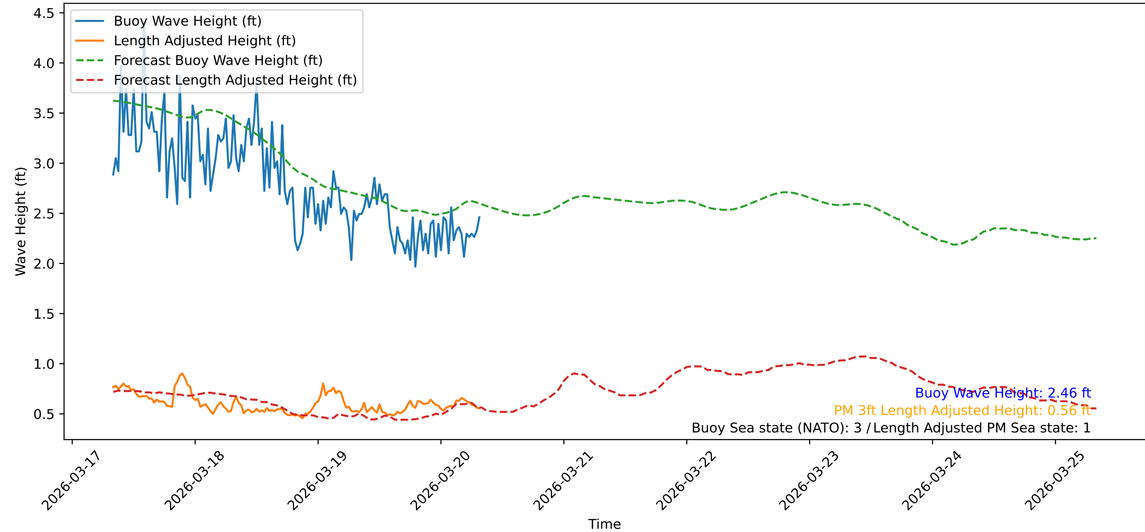
Wave Heights over Time for Oceanside Harbor at 2026-03-20 08:10:32
