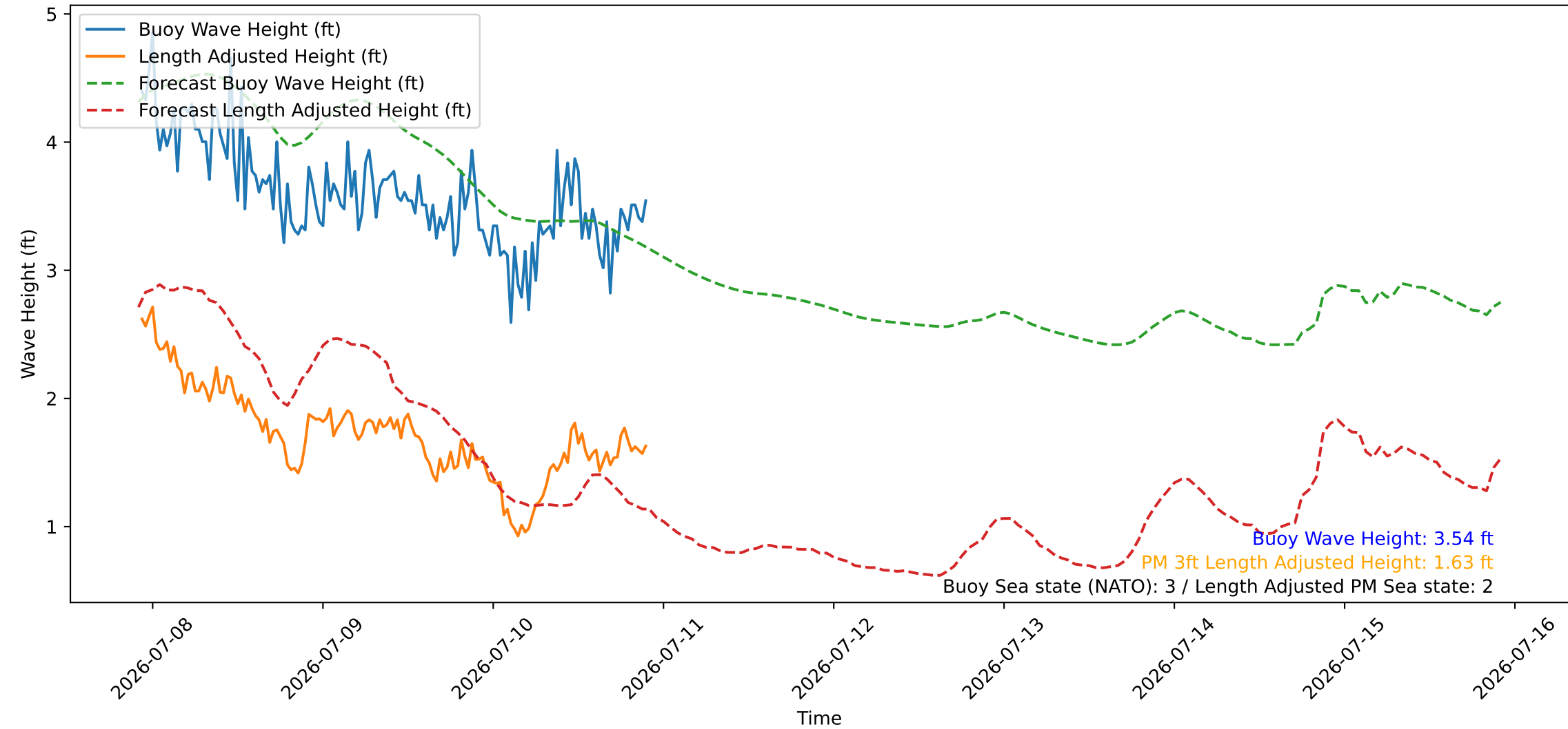
Wave Heights over Time for Red Beach at 2026-07-10 22:20:47
