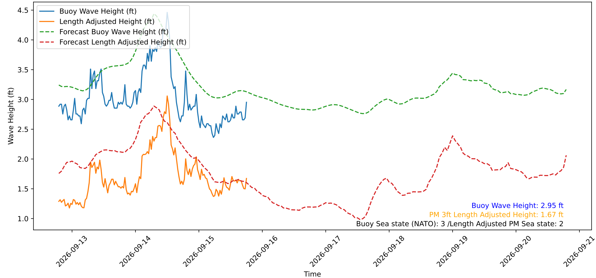
Wave Heights over Time for Oceanside Harbor at 2026-09-15 18:50:29
