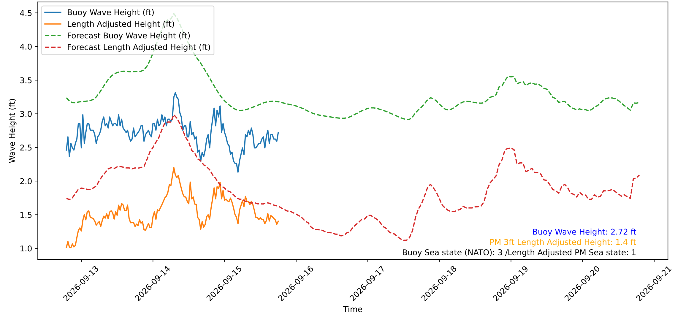
Wave Heights over Time for Green Beach at 2026-09-15 18:51:14
