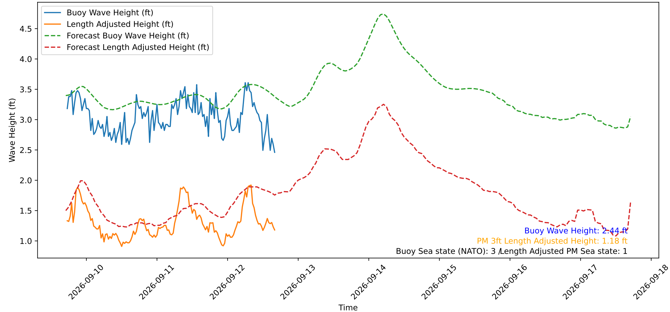
Wave Heights over Time for Green Beach at 2026-09-12 17:01:12
