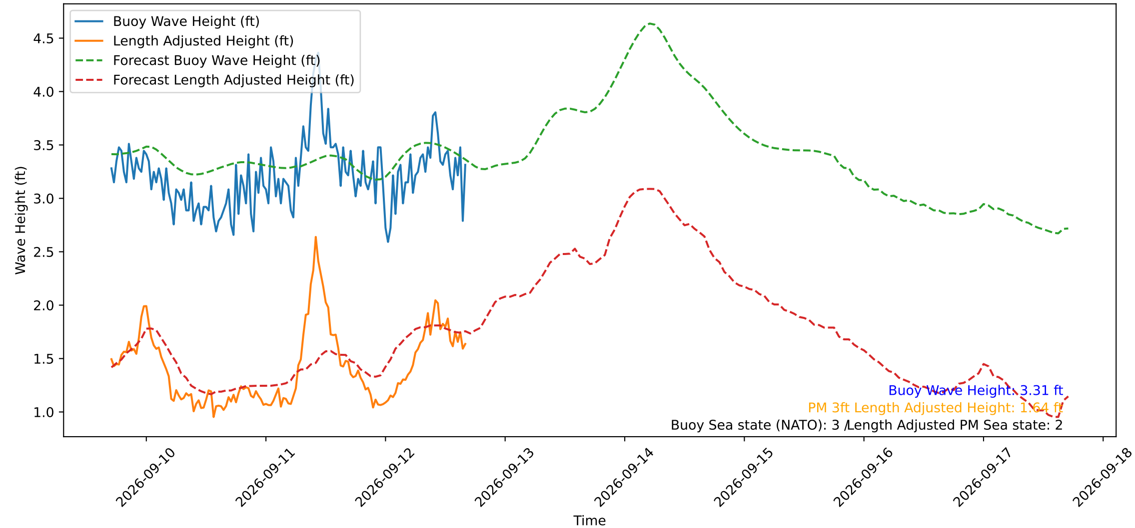
Wave Heights over Time for Oceanside Harbor at 2026-09-12 17:00:30
