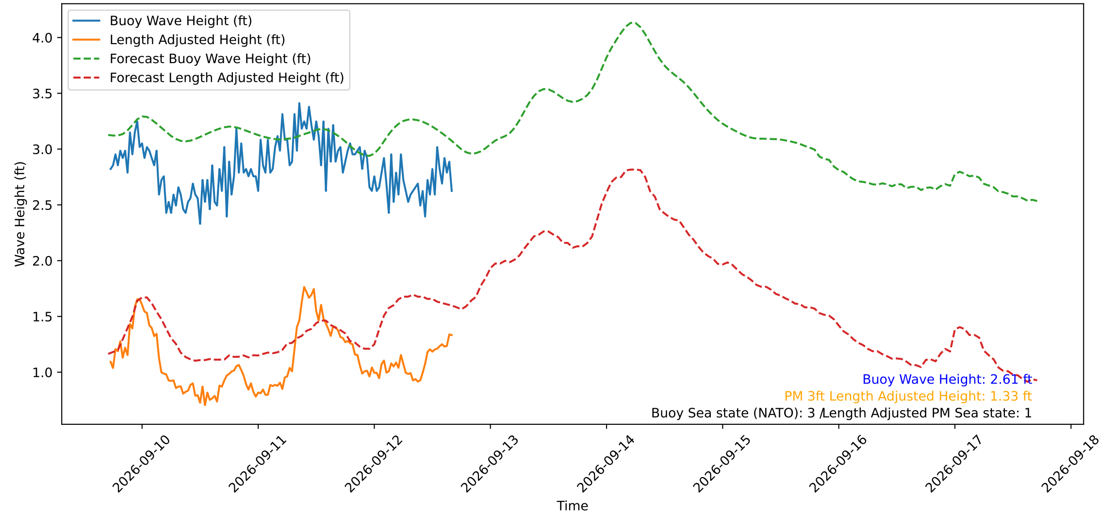
Wave Heights over Time for Red Beach at 2026-09-12 17:00:49
