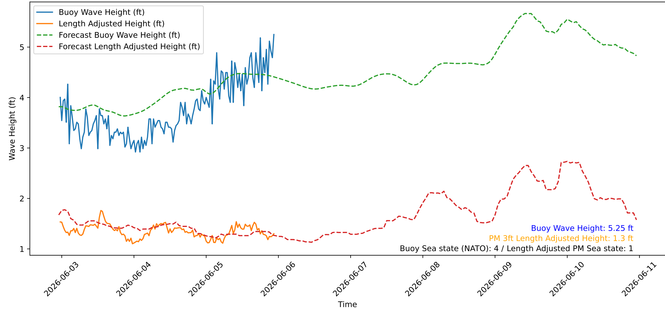
Wave Heights over Time for Oceanside Harbor at 2026-06-05 23:20:26
