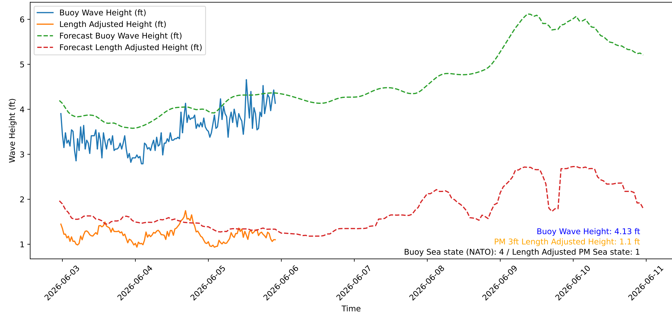
Wave Heights over Time for Green Beach at 2026-06-05 23:21:09
