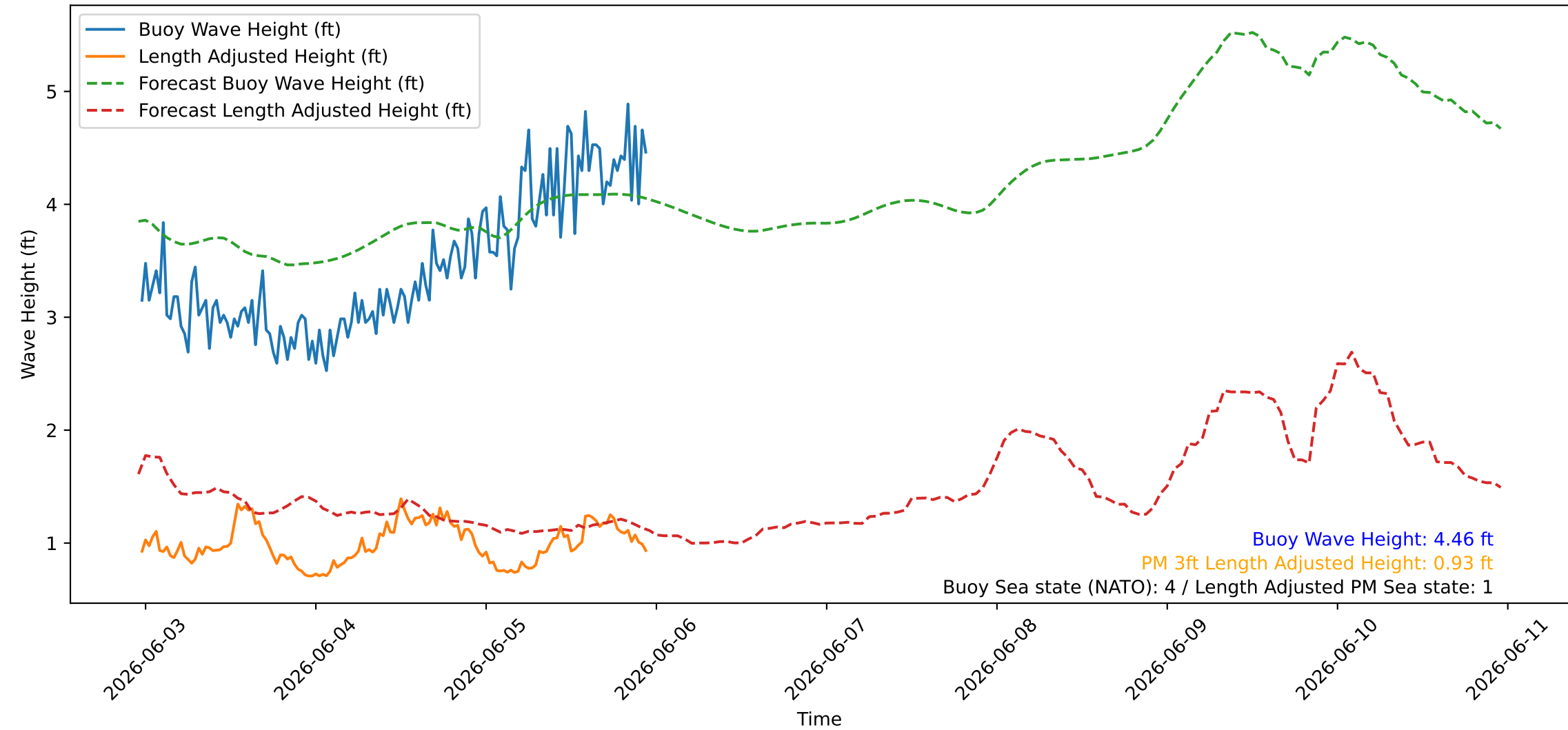
Wave Heights over Time for Red Beach at 2026-06-05 23:20:46
