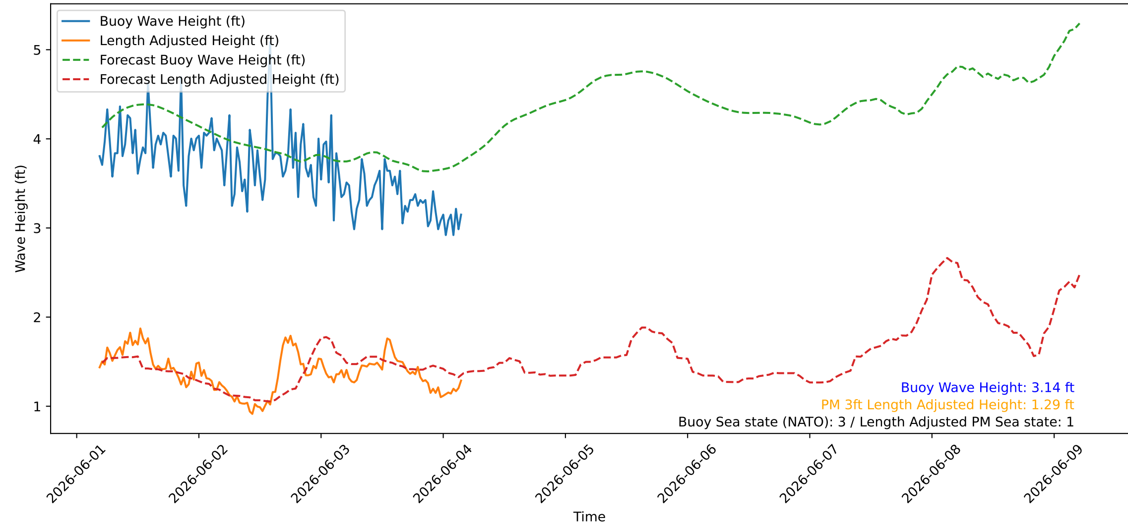
Wave Heights over Time for Oceanside Harbor at 2026-06-04 04:40:26
