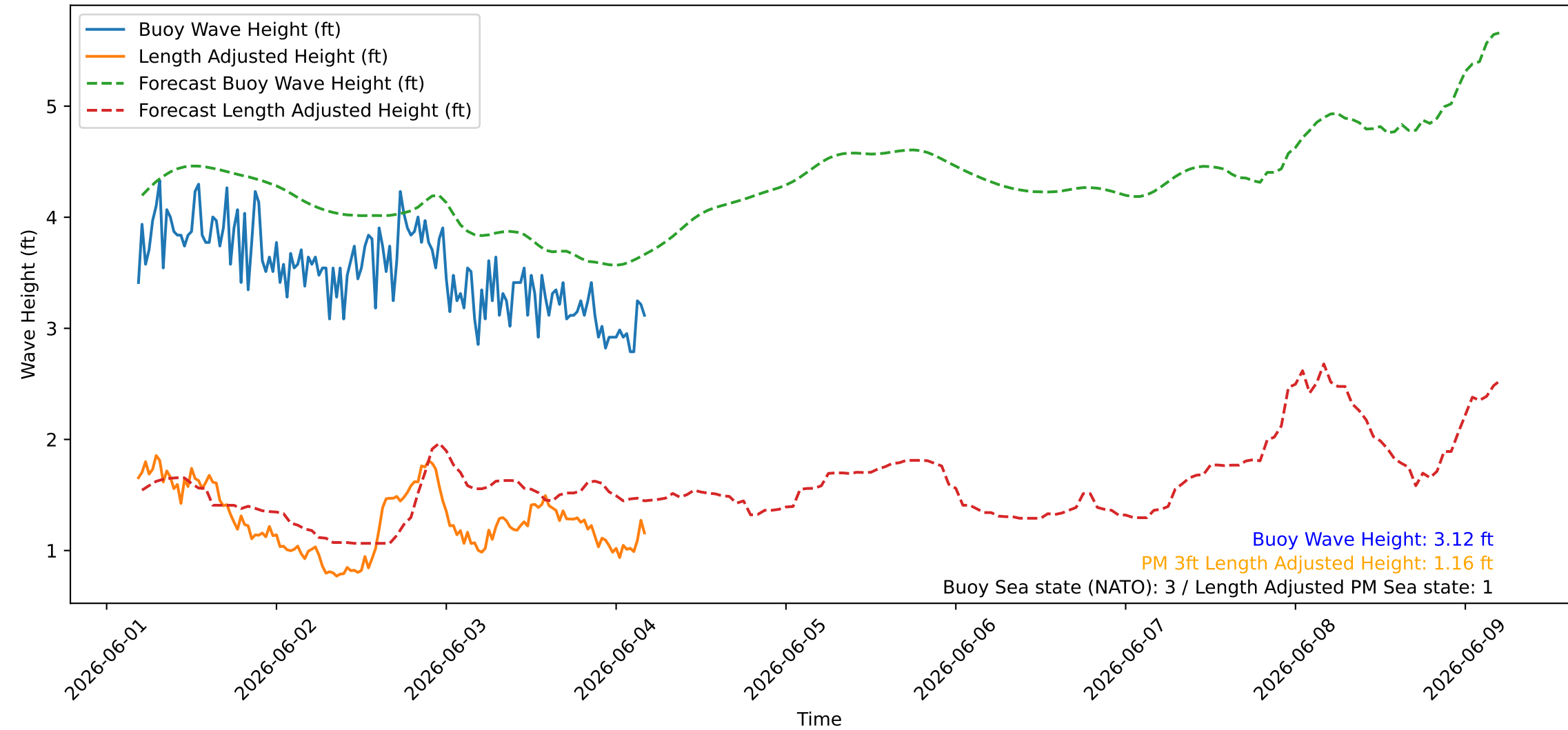
Wave Heights over Time for Green Beach at 2026-06-04 04:41:07
