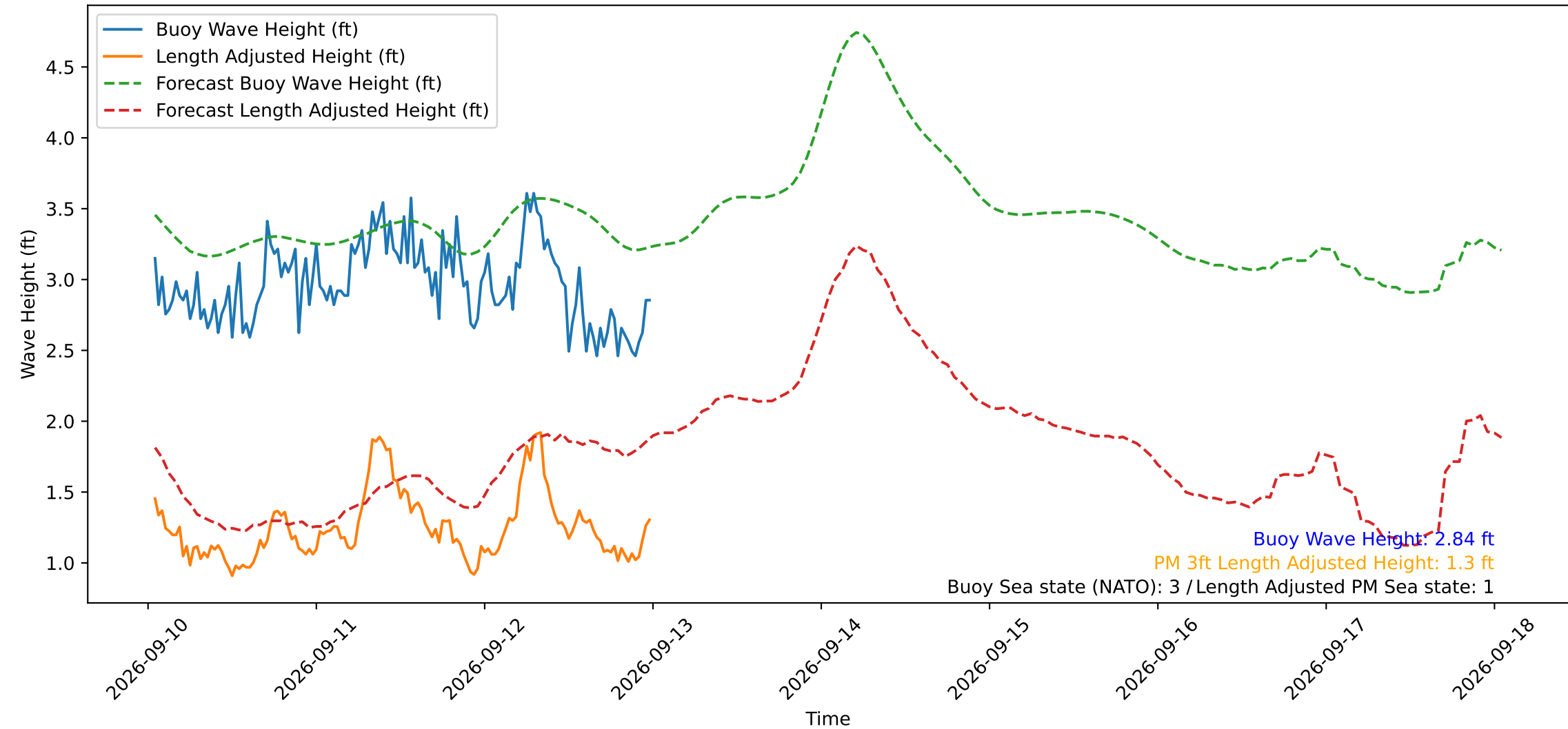
Wave Heights over Time for Green Beach at 2026-09-13 00:31:11
