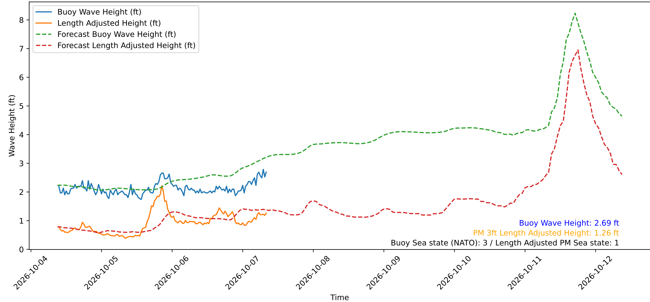
Wave Heights over Time for Red Beach at 2026-10-07 09:00:49
