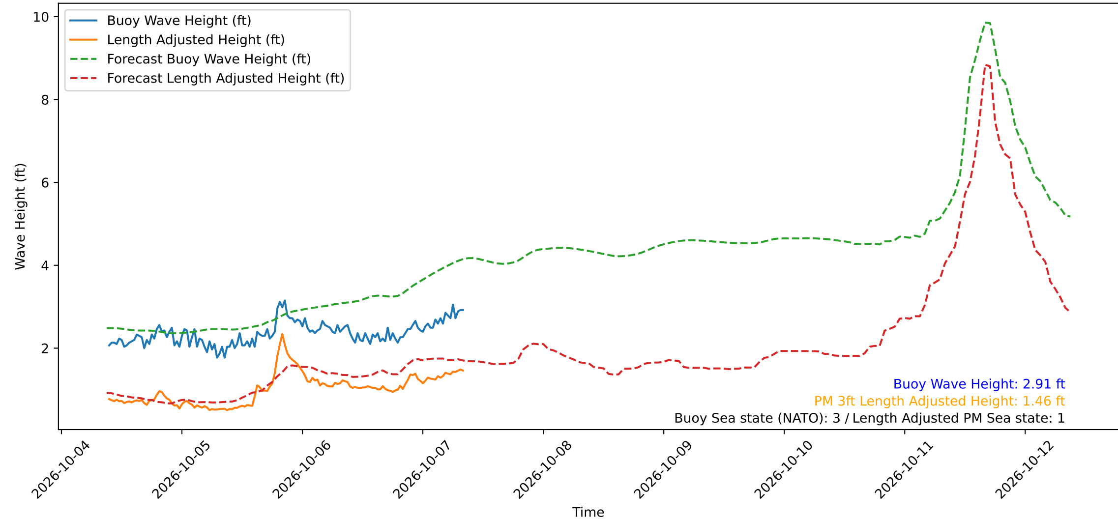
Wave Heights over Time for Green Beach at 2026-10-07 09:01:12
