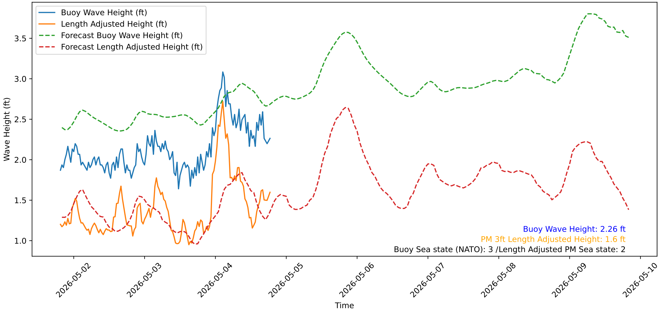
Wave Heights over Time for Oceanside Harbor at 2026-05-04 19:30:31
