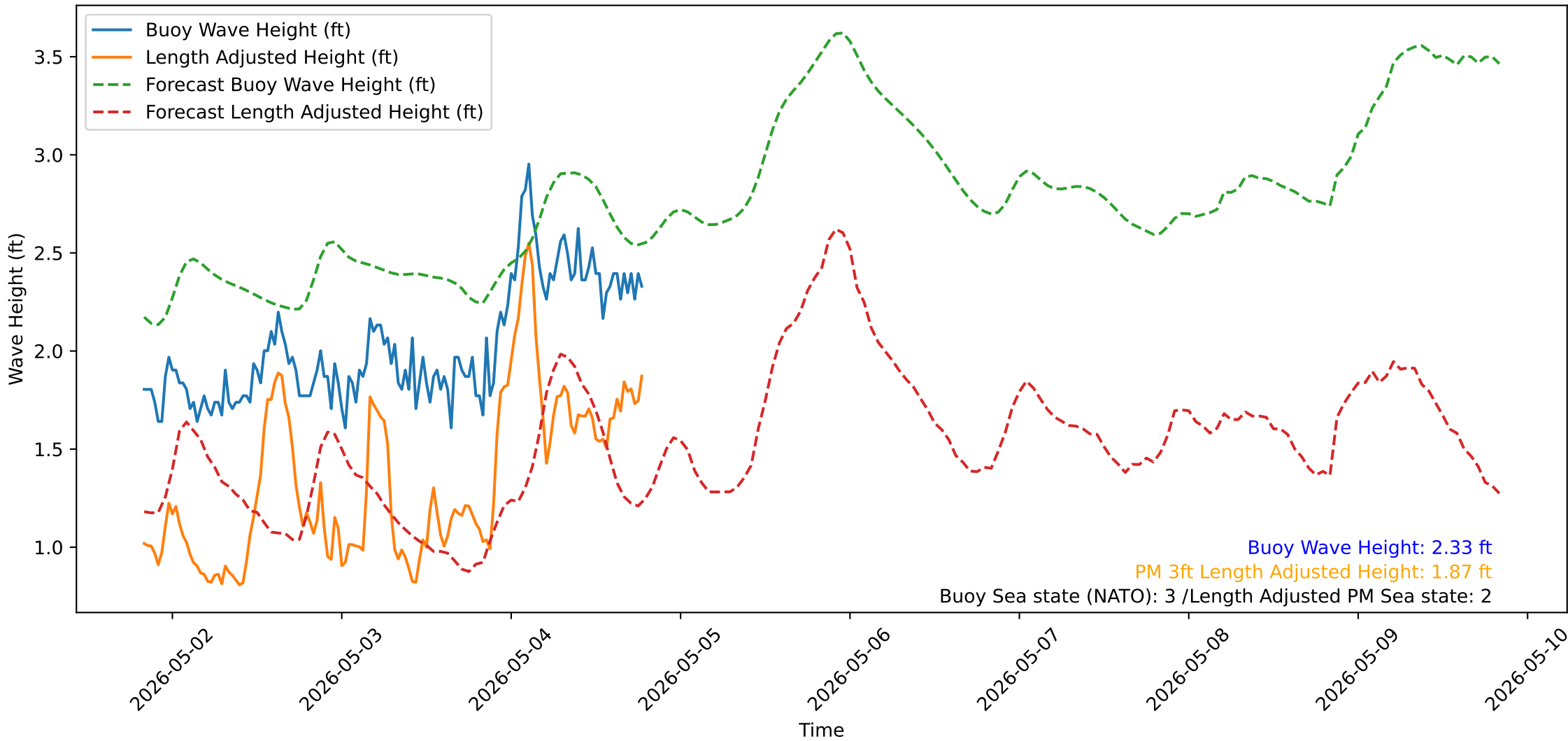
Wave Heights over Time for Red Beach at 2026-05-04 19:30:50
