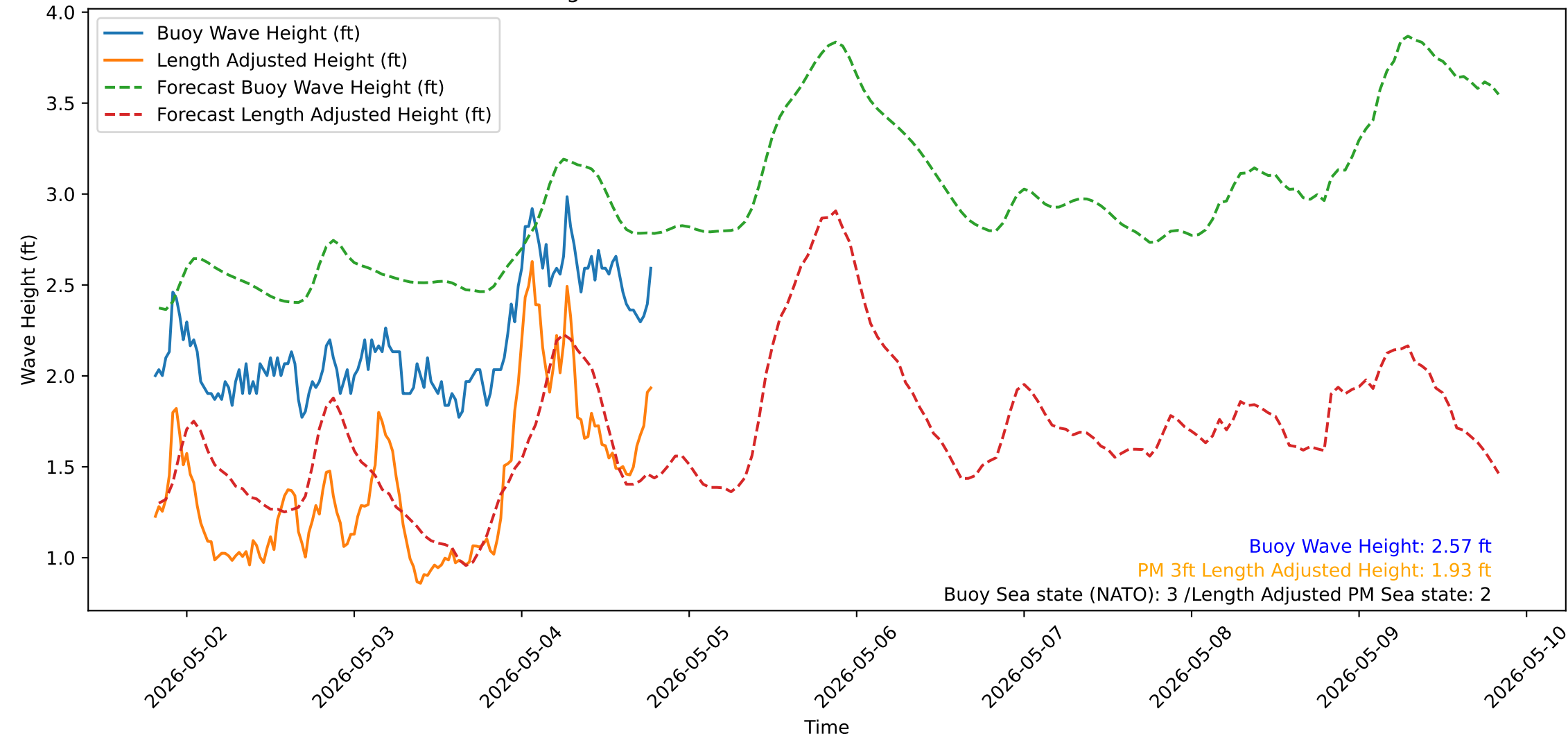
Wave Heights over Time for Green Beach at 2026-05-04 19:31:12
