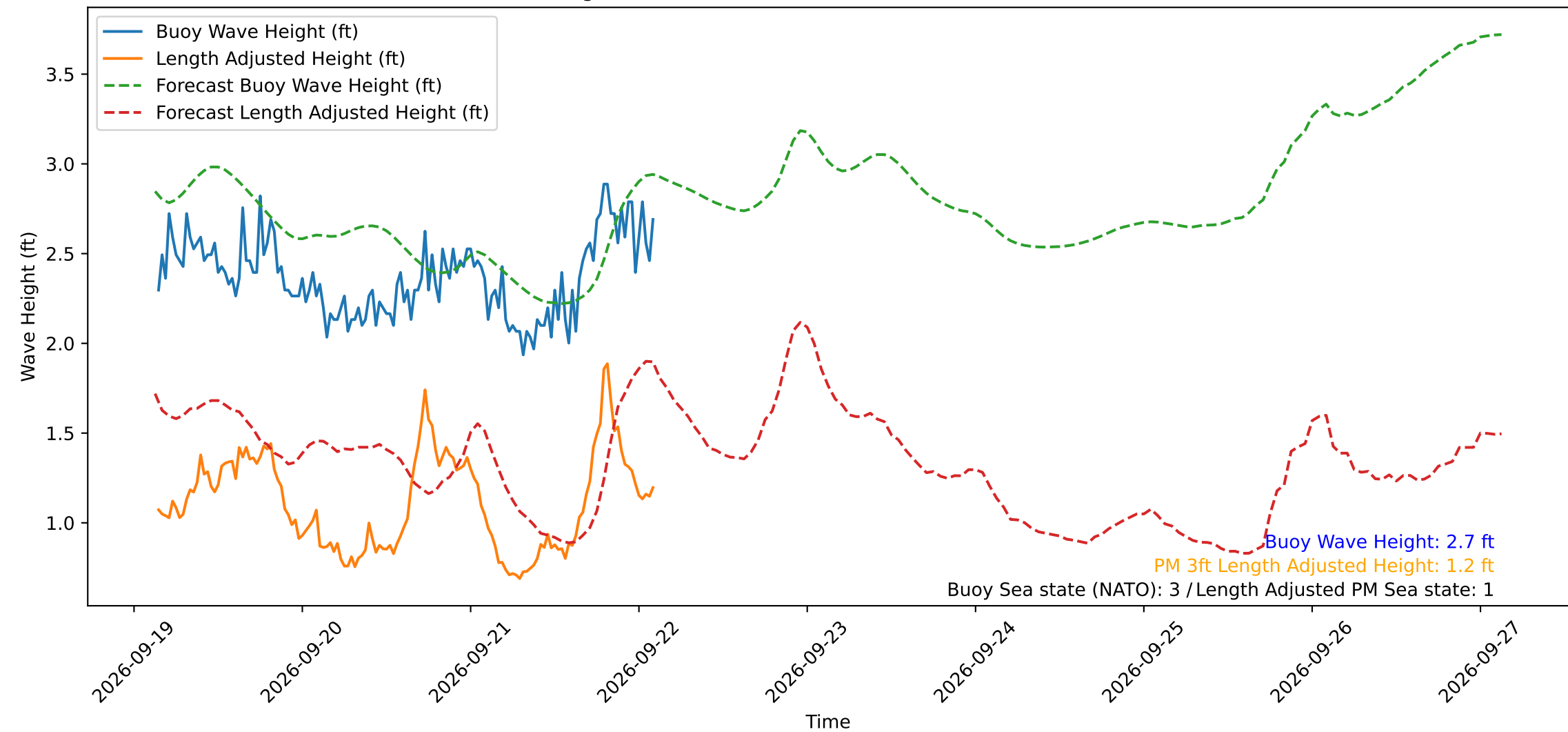
Wave Heights over Time for Red Beach at 2026-09-22 03:00:48
