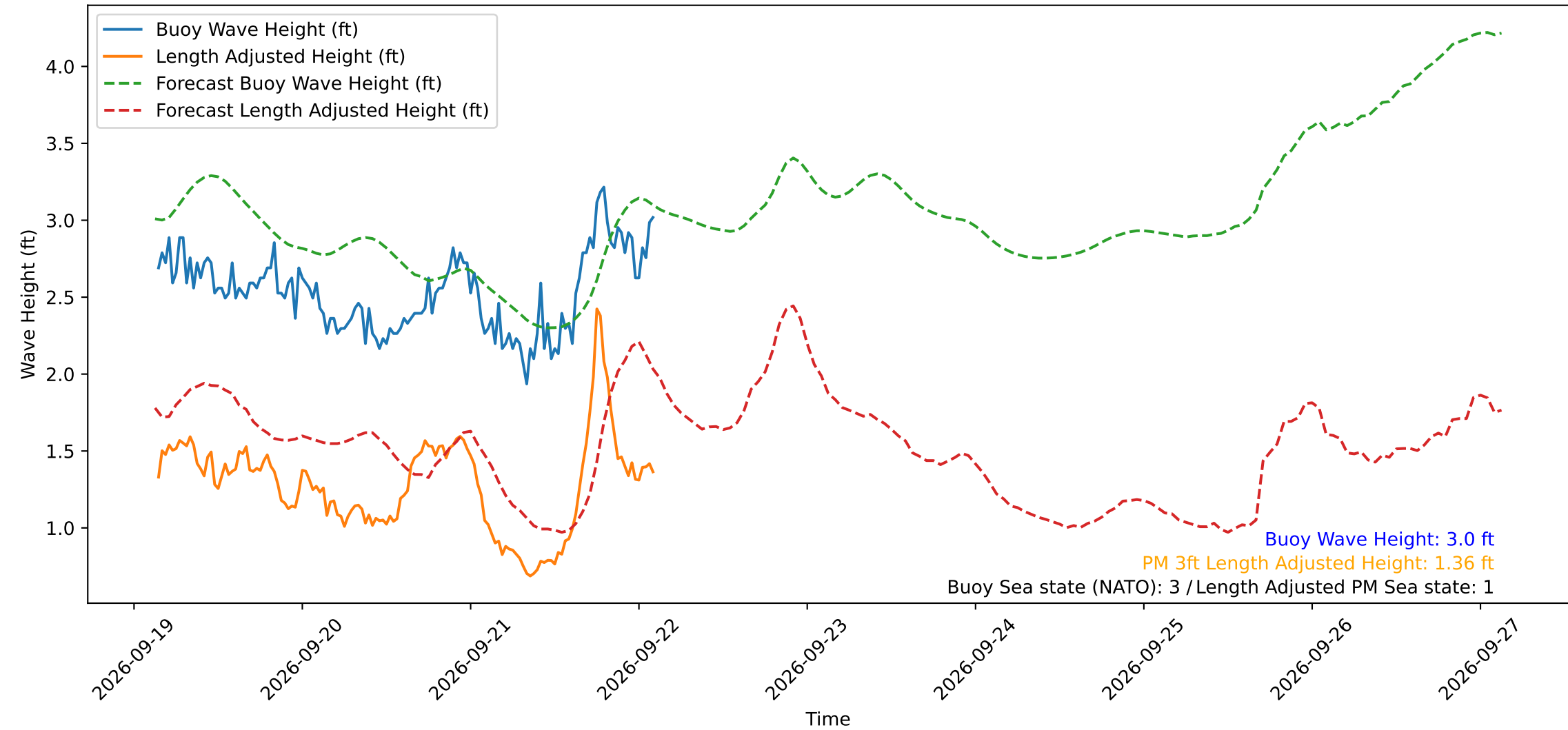
Wave Heights over Time for Green Beach at 2026-09-22 03:01:10
