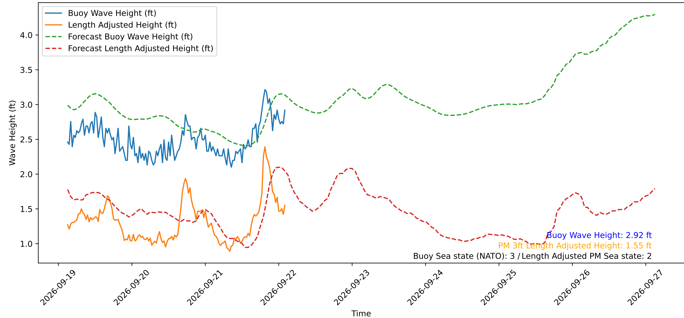
Wave Heights over Time for Oceanside Harbor at 2026-09-22 03:00:29
