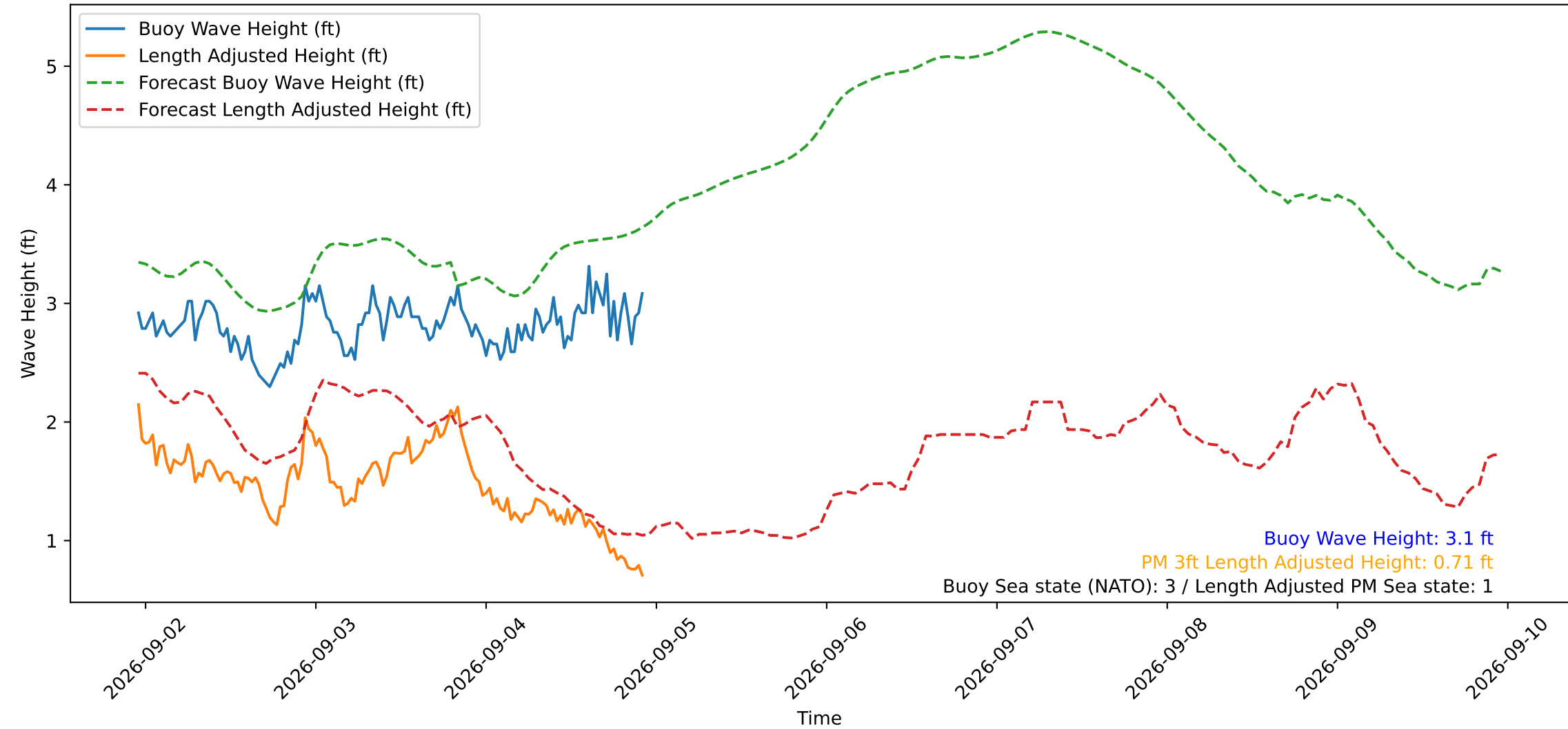
Wave Heights over Time for Red Beach at 2026-09-04 22:50:51
