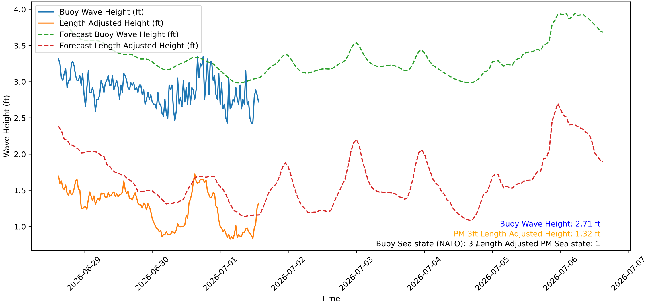
Wave Heights over Time for Red Beach at 2026-07-01 14:30:46
