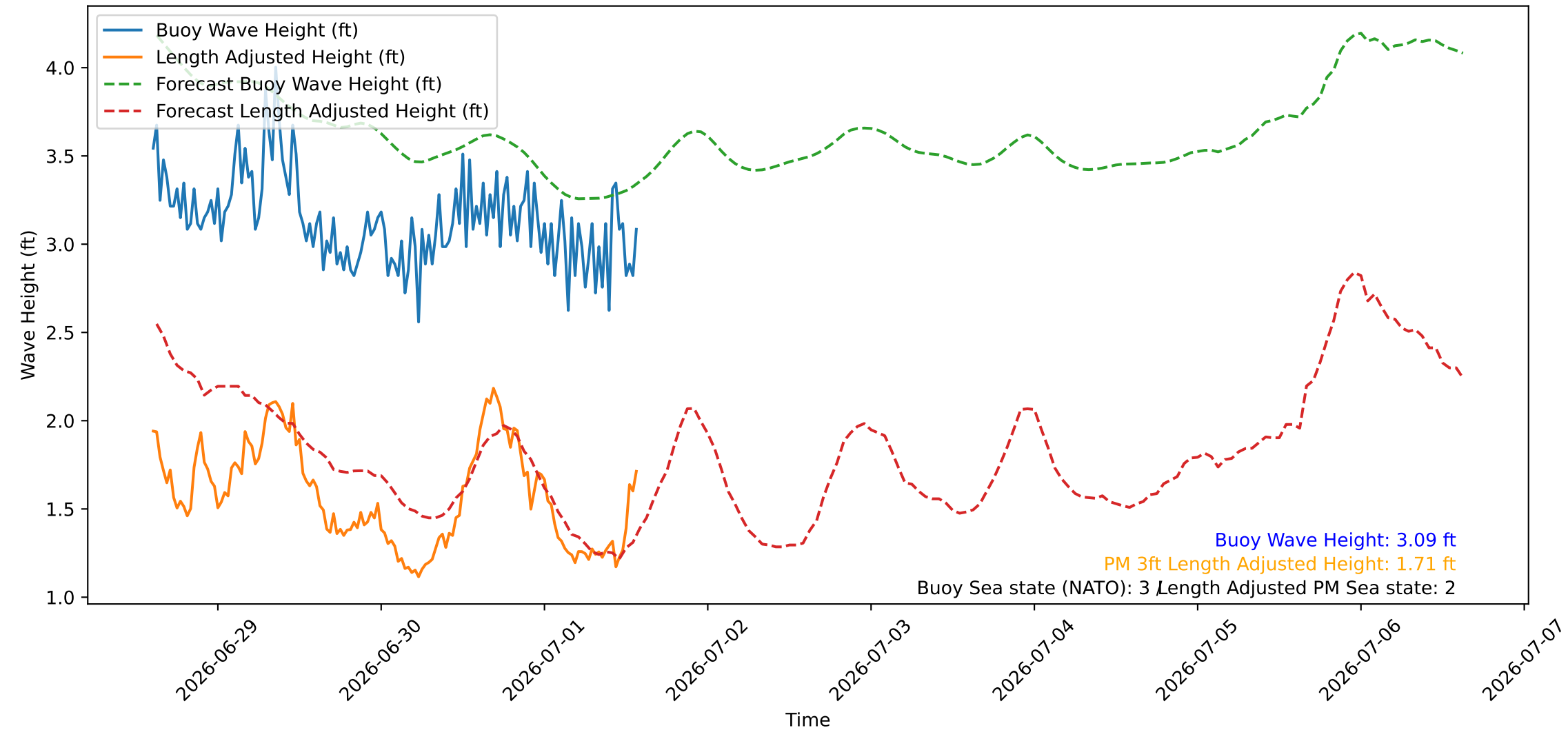
Wave Heights over Time for Oceanside Harbor at 2026-07-01 14:30:26
