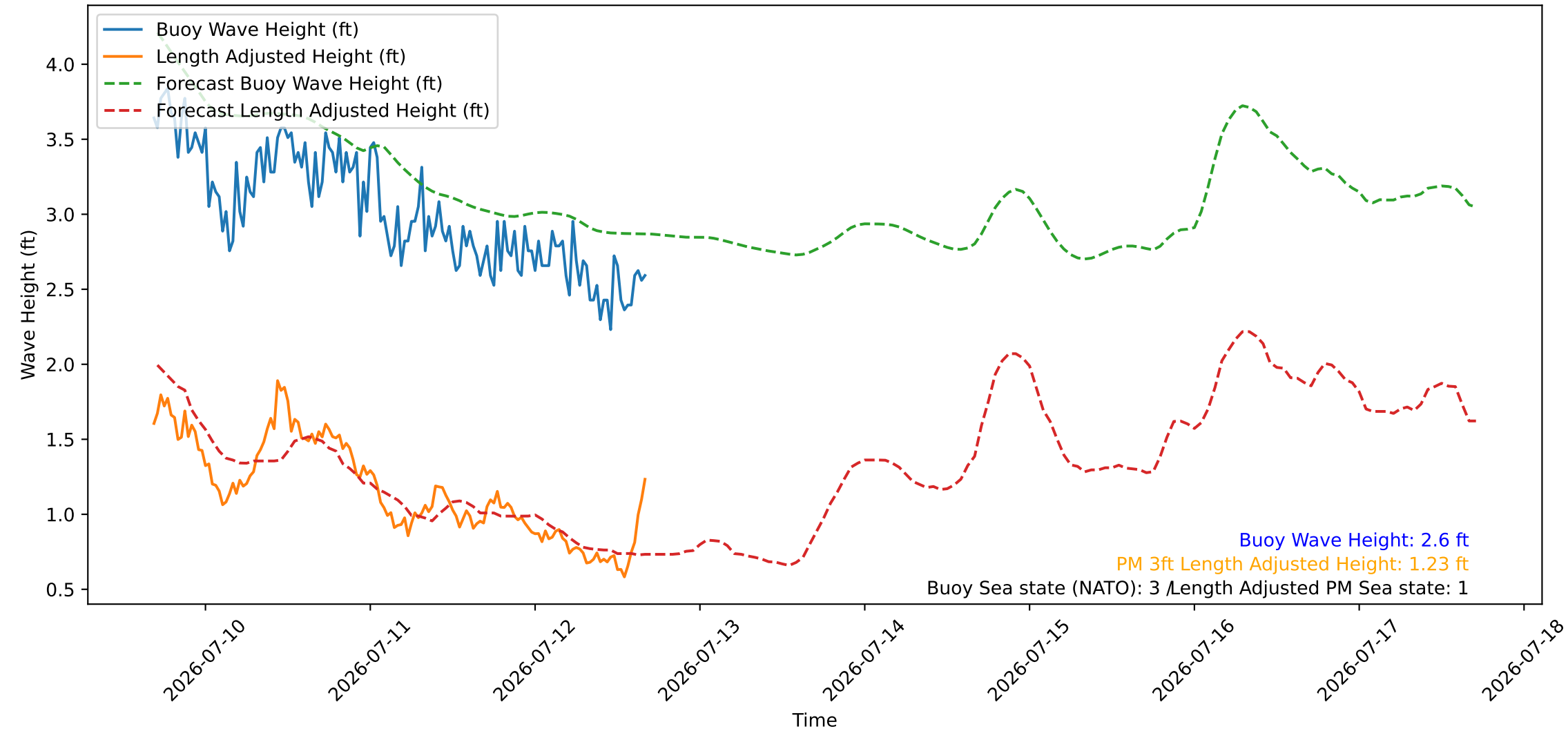
Wave Heights over Time for Green Beach at 2026-07-12 16:41:08
