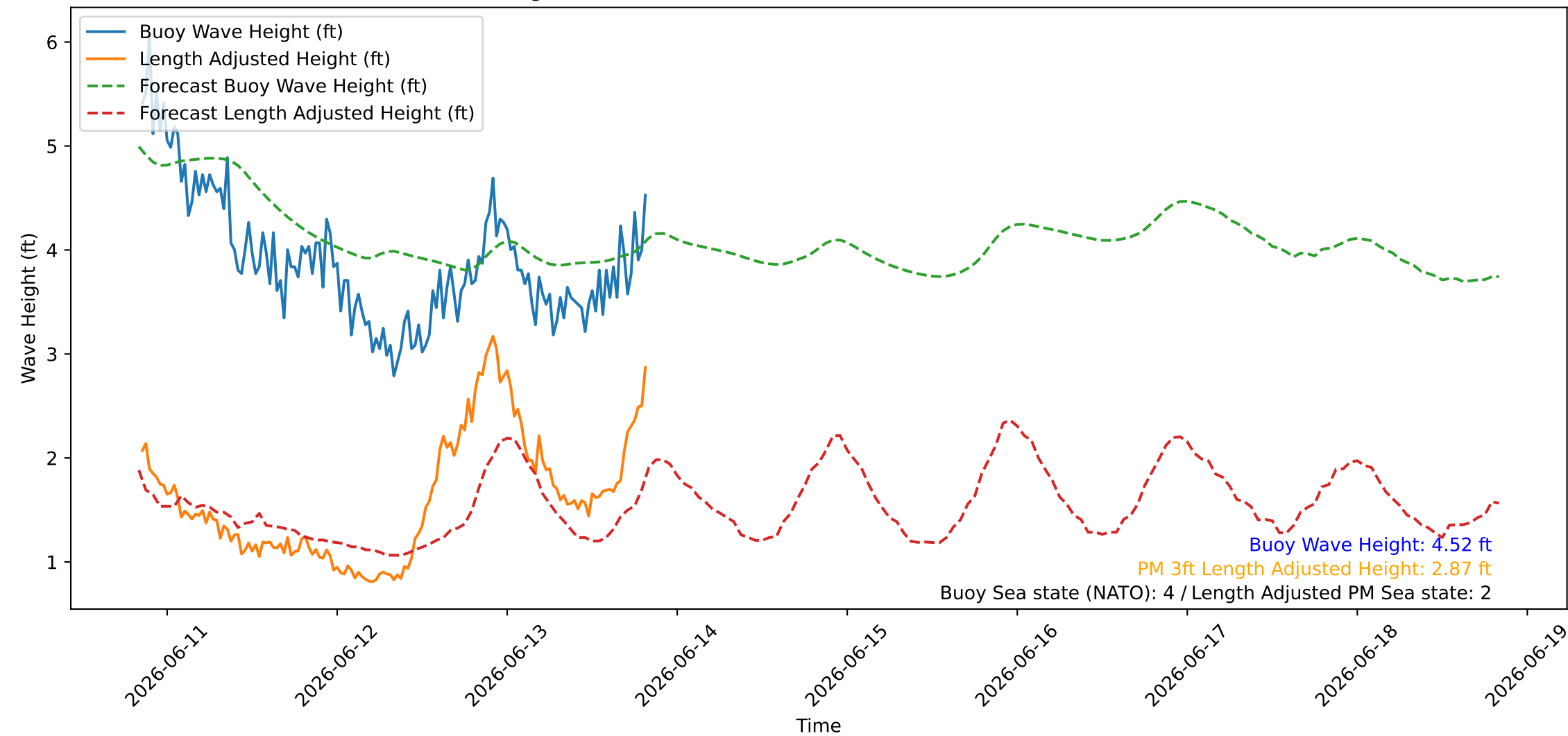
Wave Heights over Time for Oceanside Harbor at 2026-06-13 20:20:26
