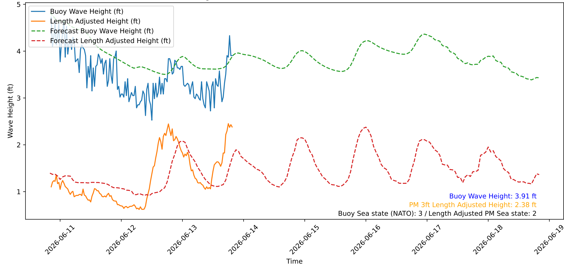
Wave Heights over Time for Red Beach at 2026-06-13 20:20:47
