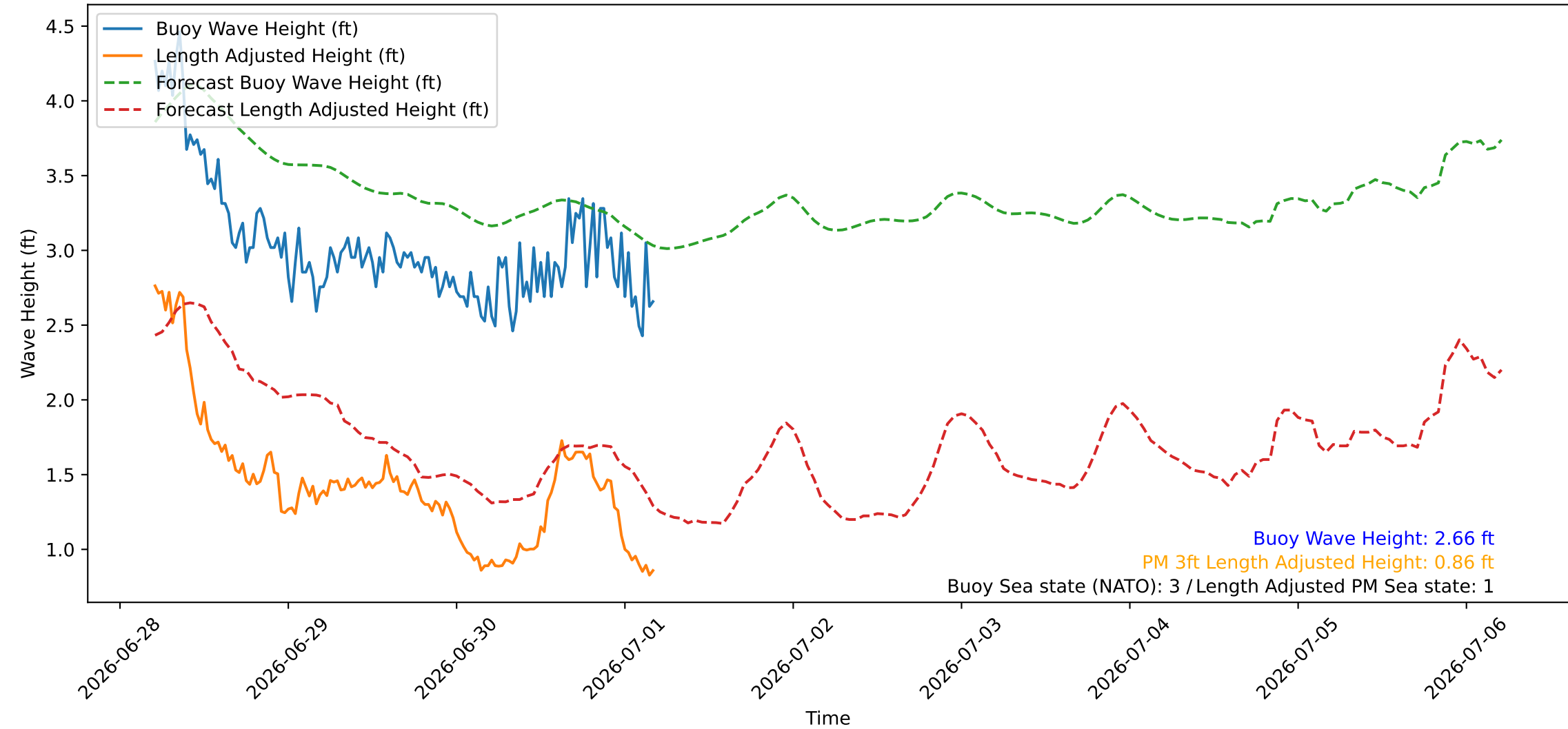
Wave Heights over Time for Red Beach at 2026-07-01 04:50:47
