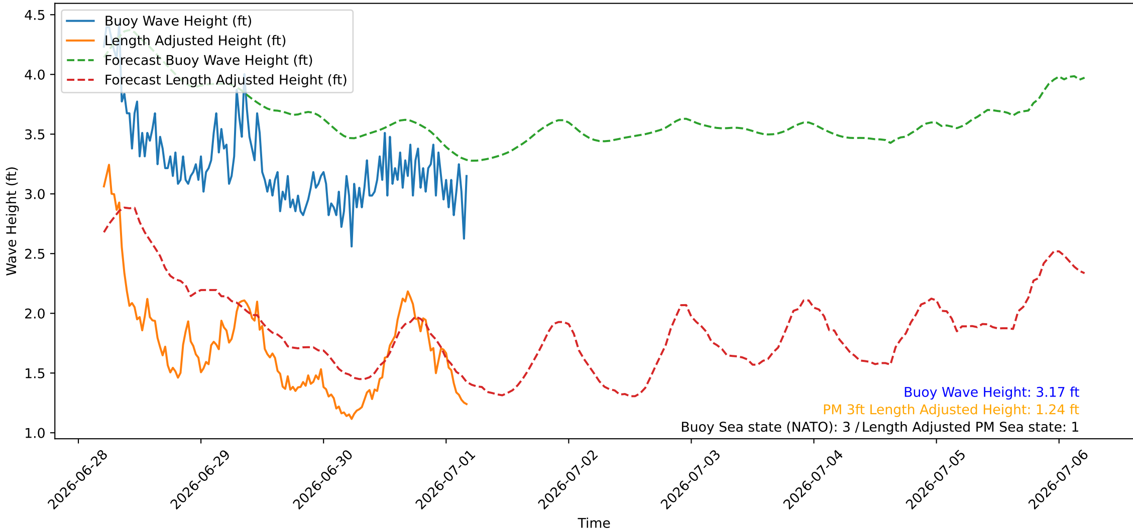
Wave Heights over Time for Oceanside Harbor at 2026-07-01 04:50:26
