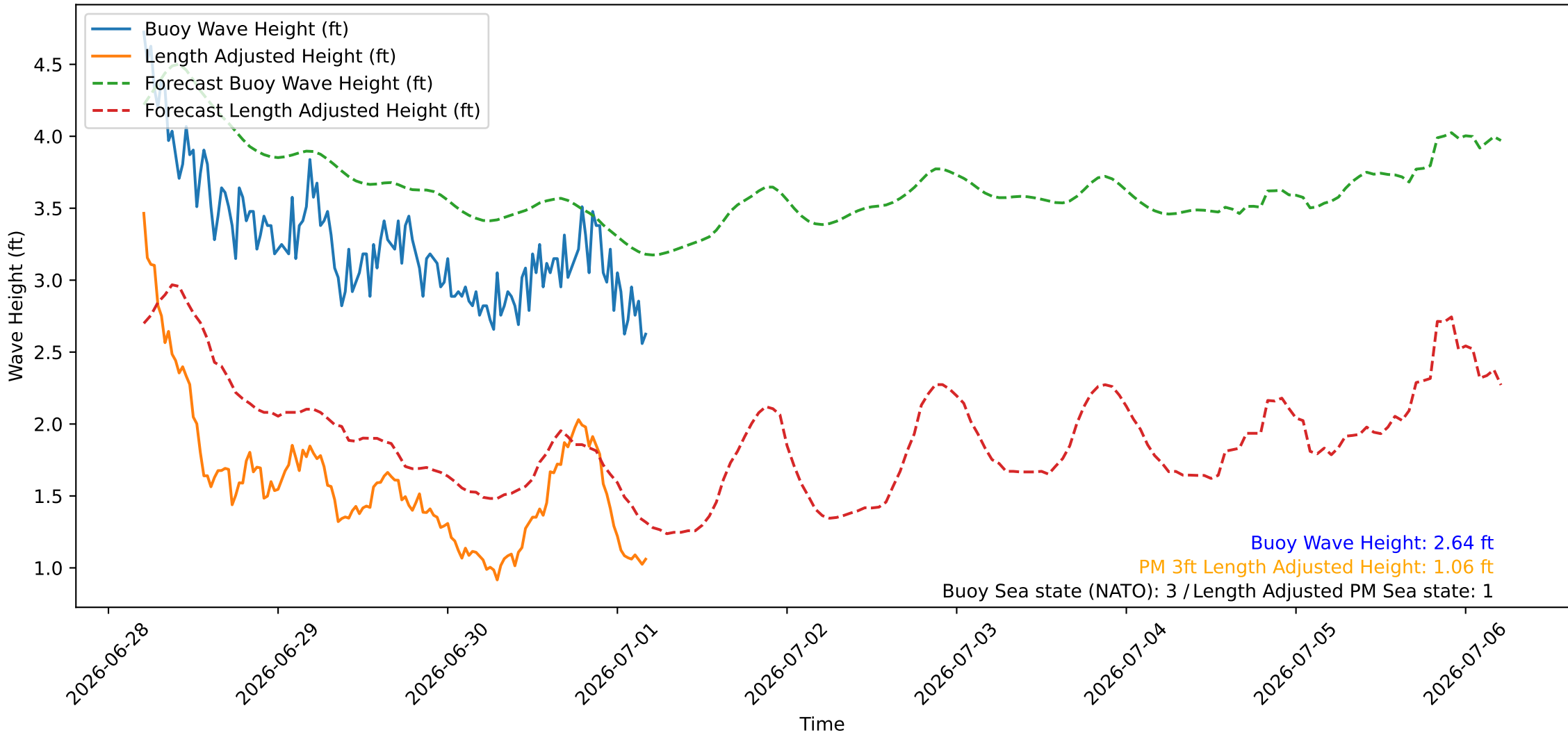
Wave Heights over Time for Green Beach at 2026-07-01 04:51:09
