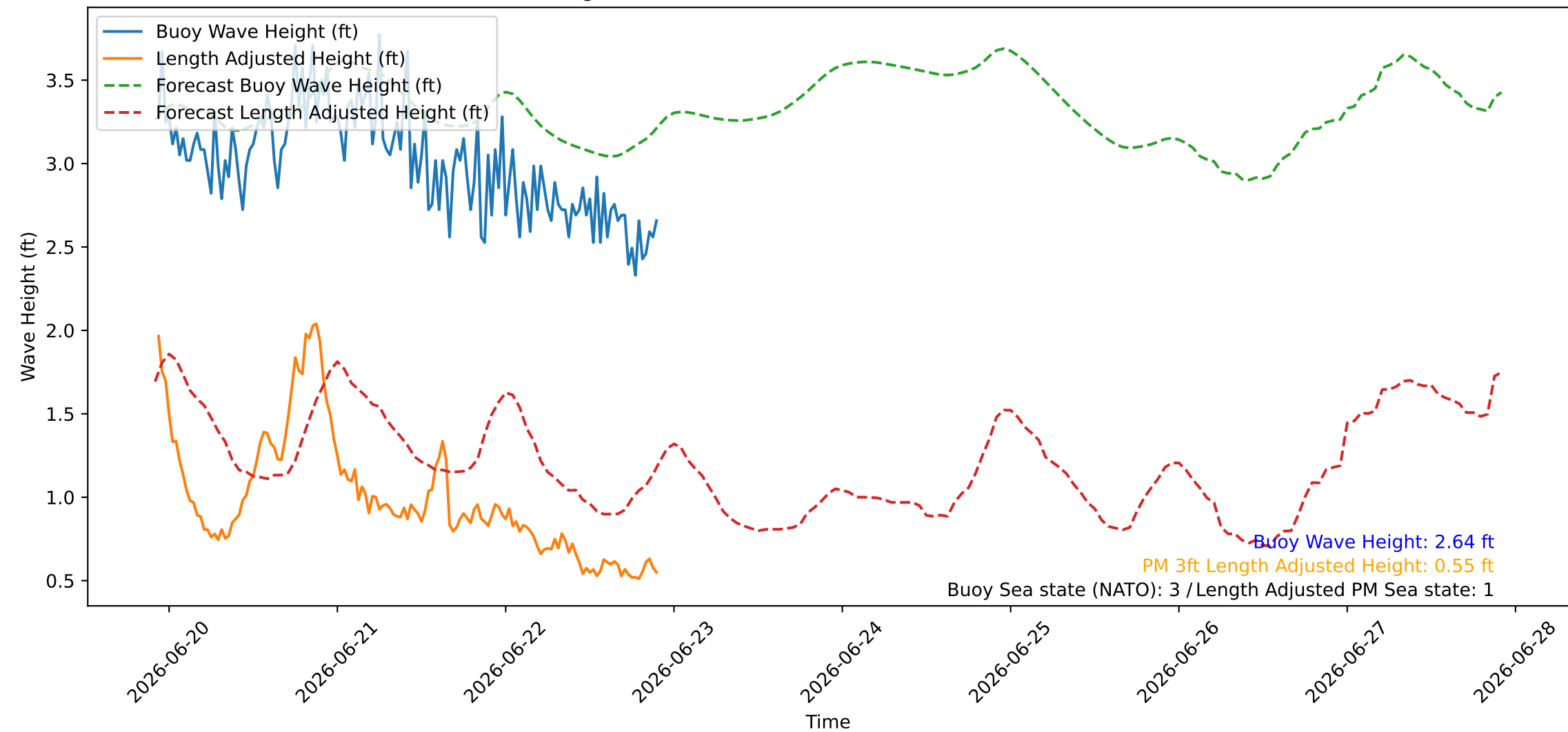
Wave Heights over Time for Red Beach at 2026-06-22 22:10:45
