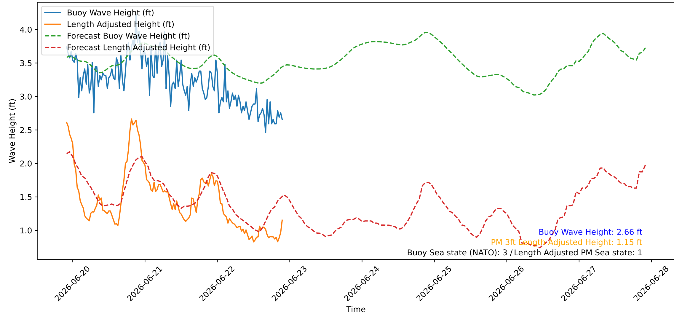
Wave Heights over Time for Green Beach at 2026-06-22 22:11:08
