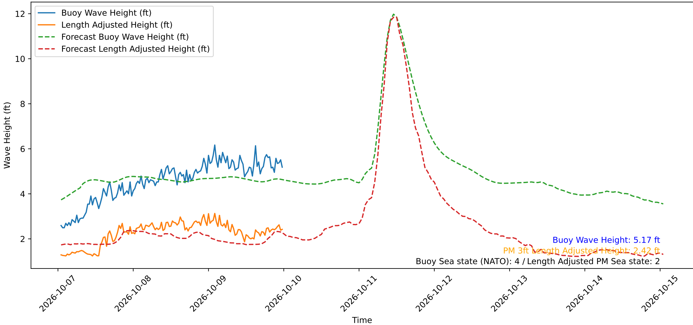
Wave Heights over Time for Green Beach at 2026-10-10 00:31:11
