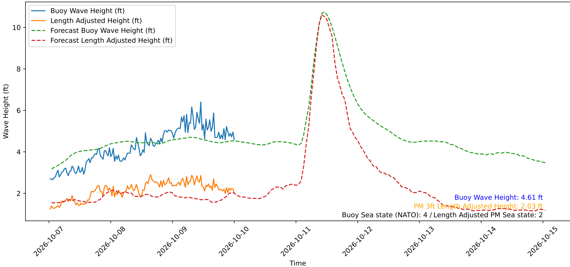
Wave Heights over Time for Oceanside Harbor at 2026-10-10 00:30:29
