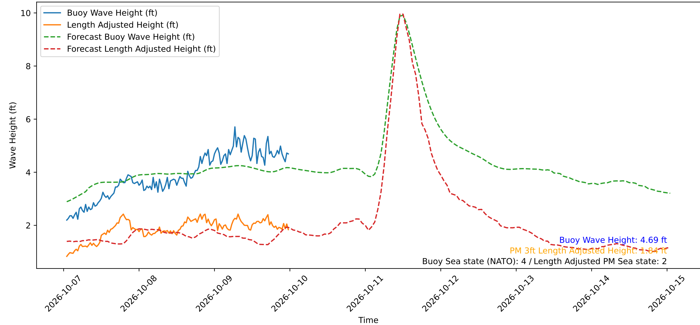
Wave Heights over Time for Red Beach at 2026-10-10 00:30:49
