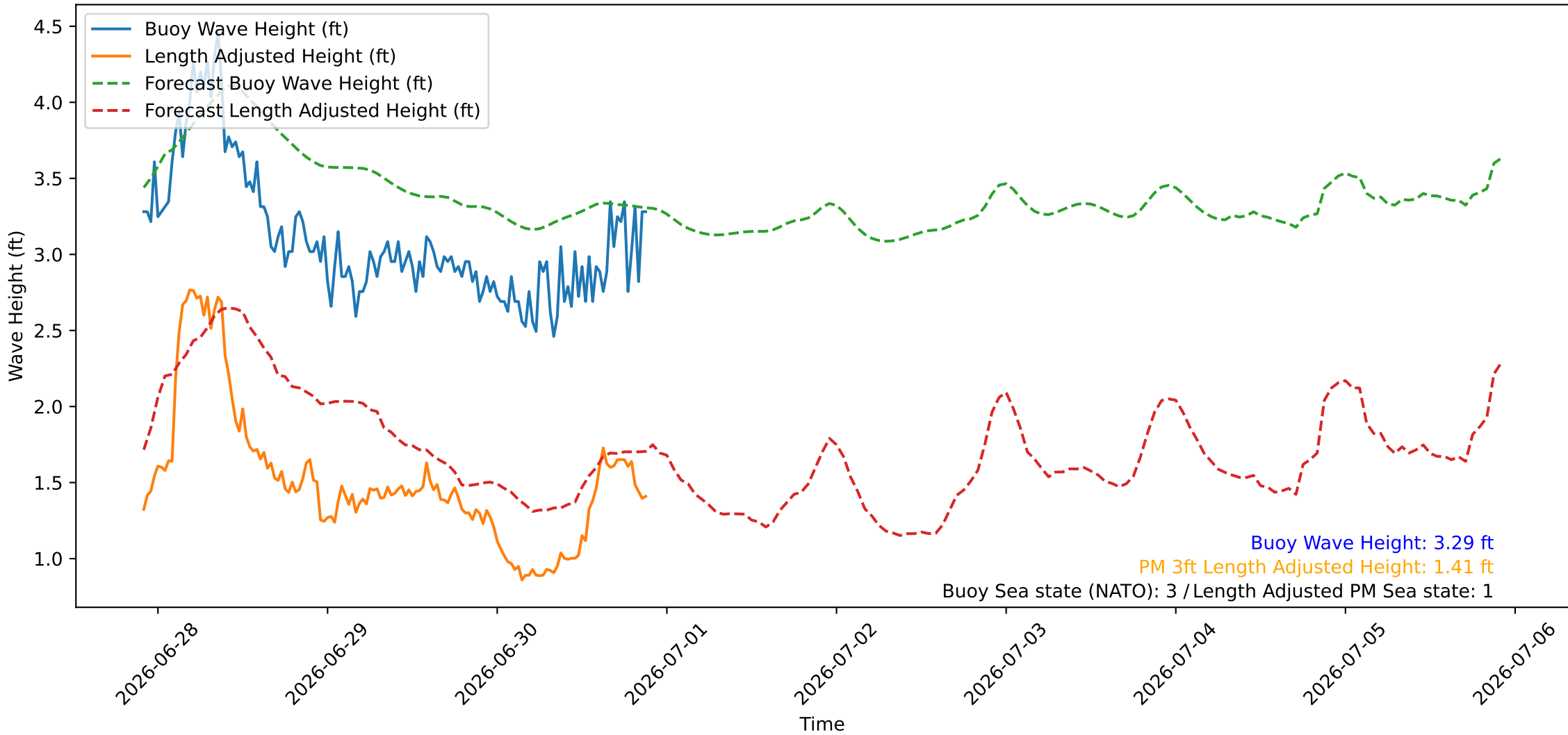
Wave Heights over Time for Red Beach at 2026-06-30 21:50:47
