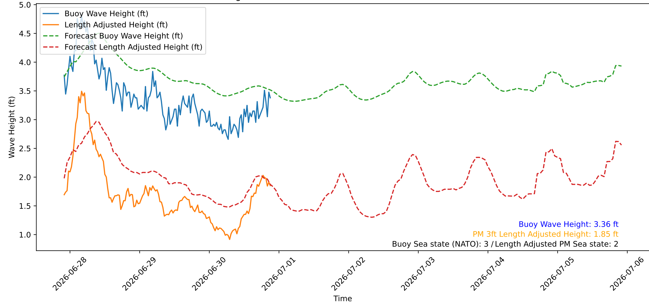
Wave Heights over Time for Green Beach at 2026-06-30 21:51:10
