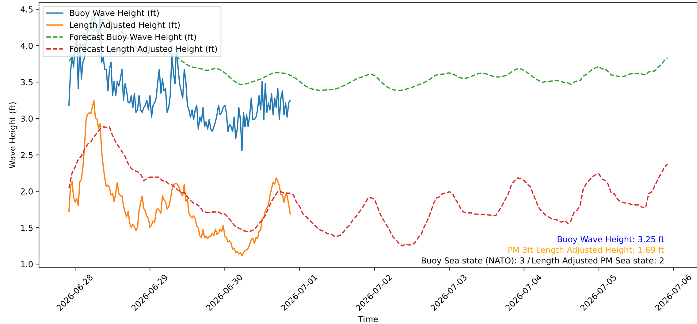
Wave Heights over Time for Oceanside Harbor at 2026-06-30 21:50:27
