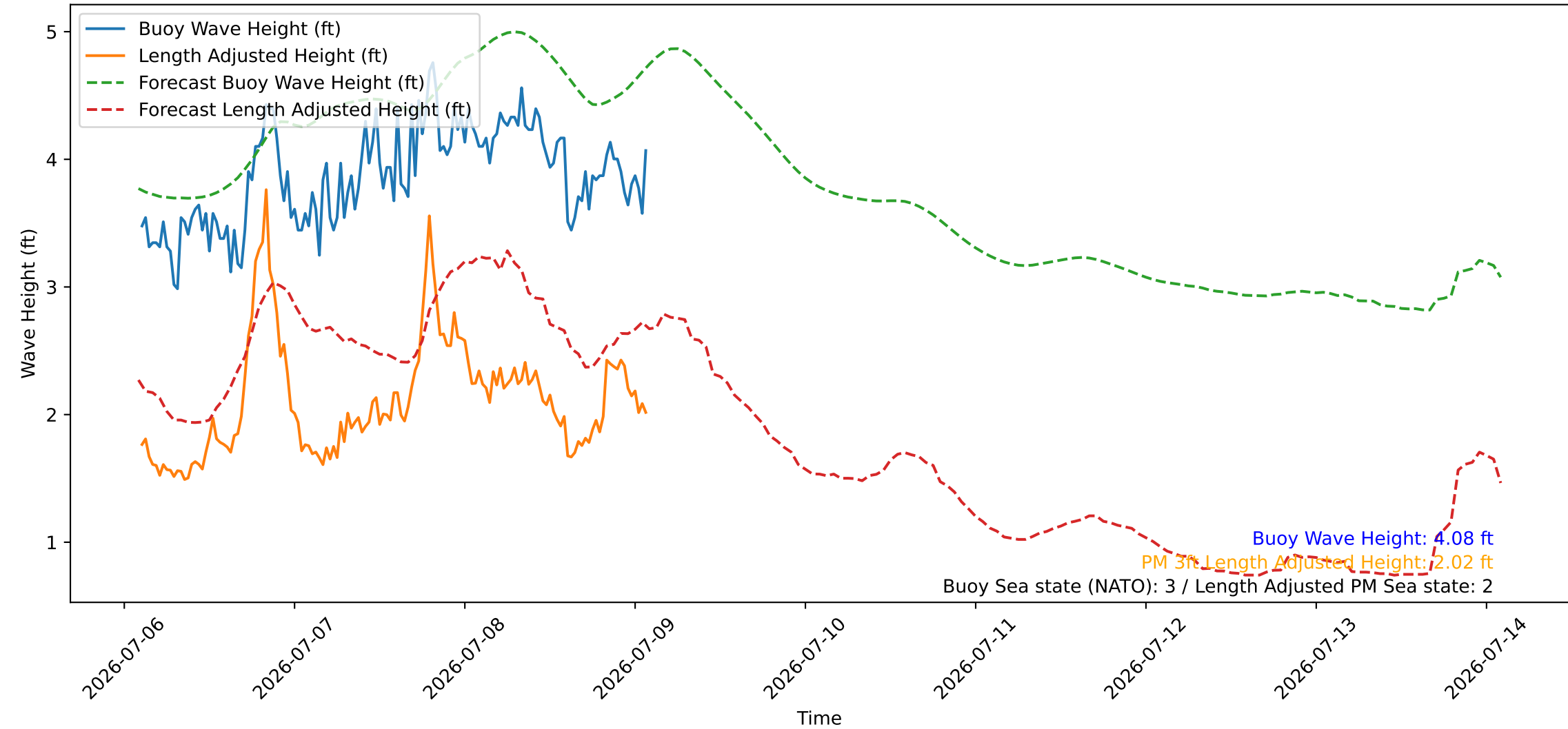
Wave Heights over Time for Green Beach at 2026-07-09 02:21:09
