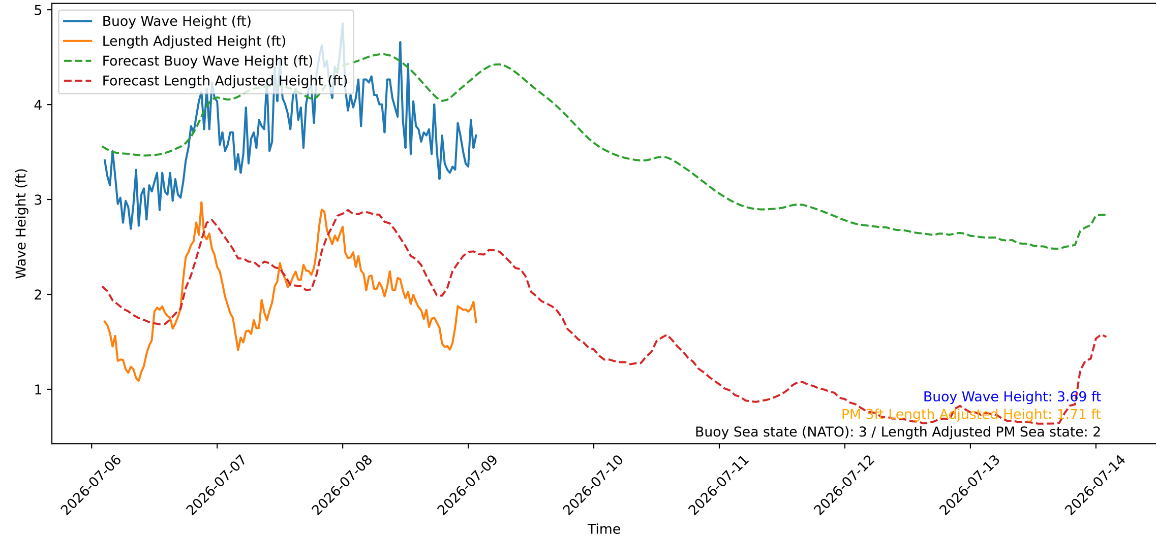
Wave Heights over Time for Red Beach at 2026-07-09 02:20:47
