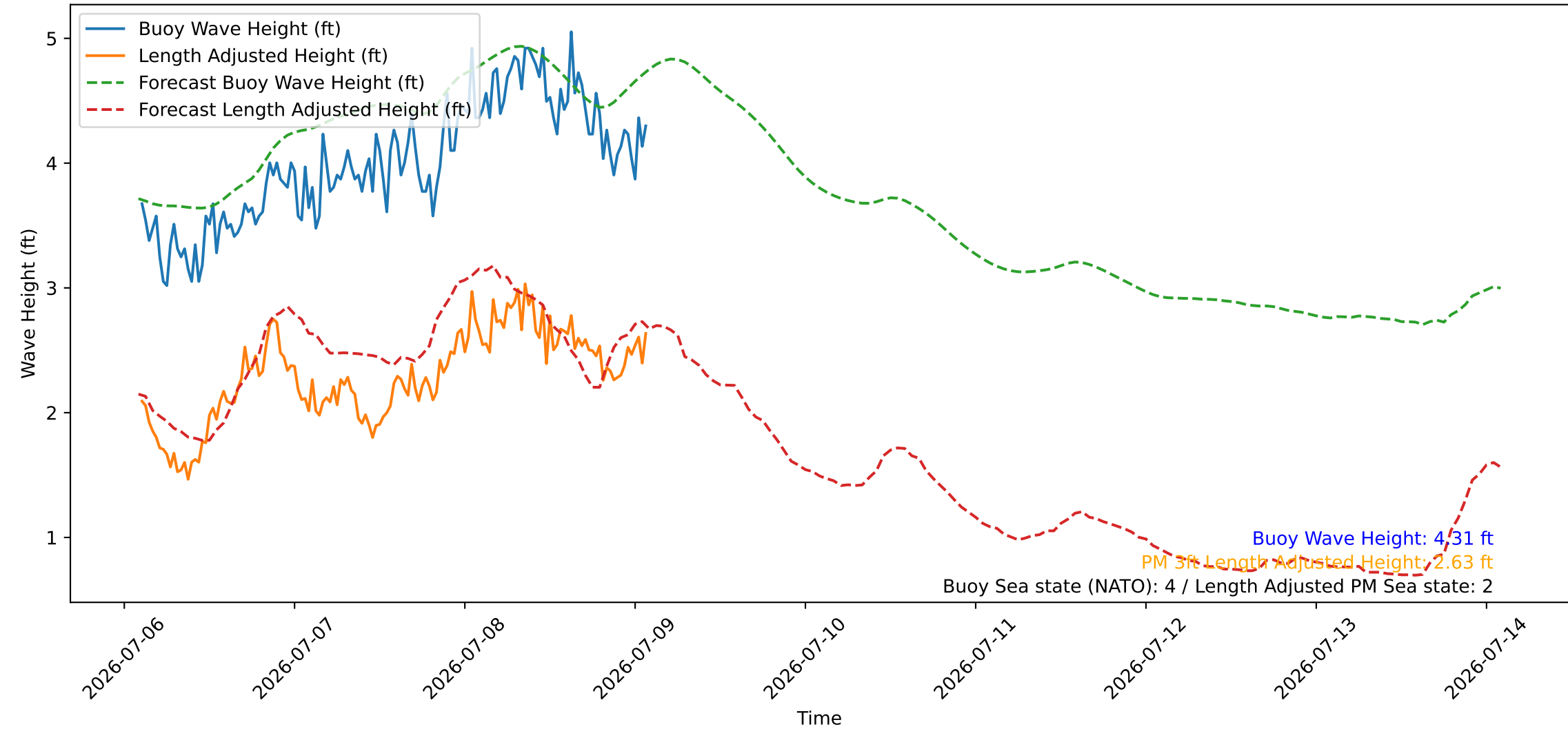
Wave Heights over Time for Oceanside Harbor at 2026-07-09 02:20:26
