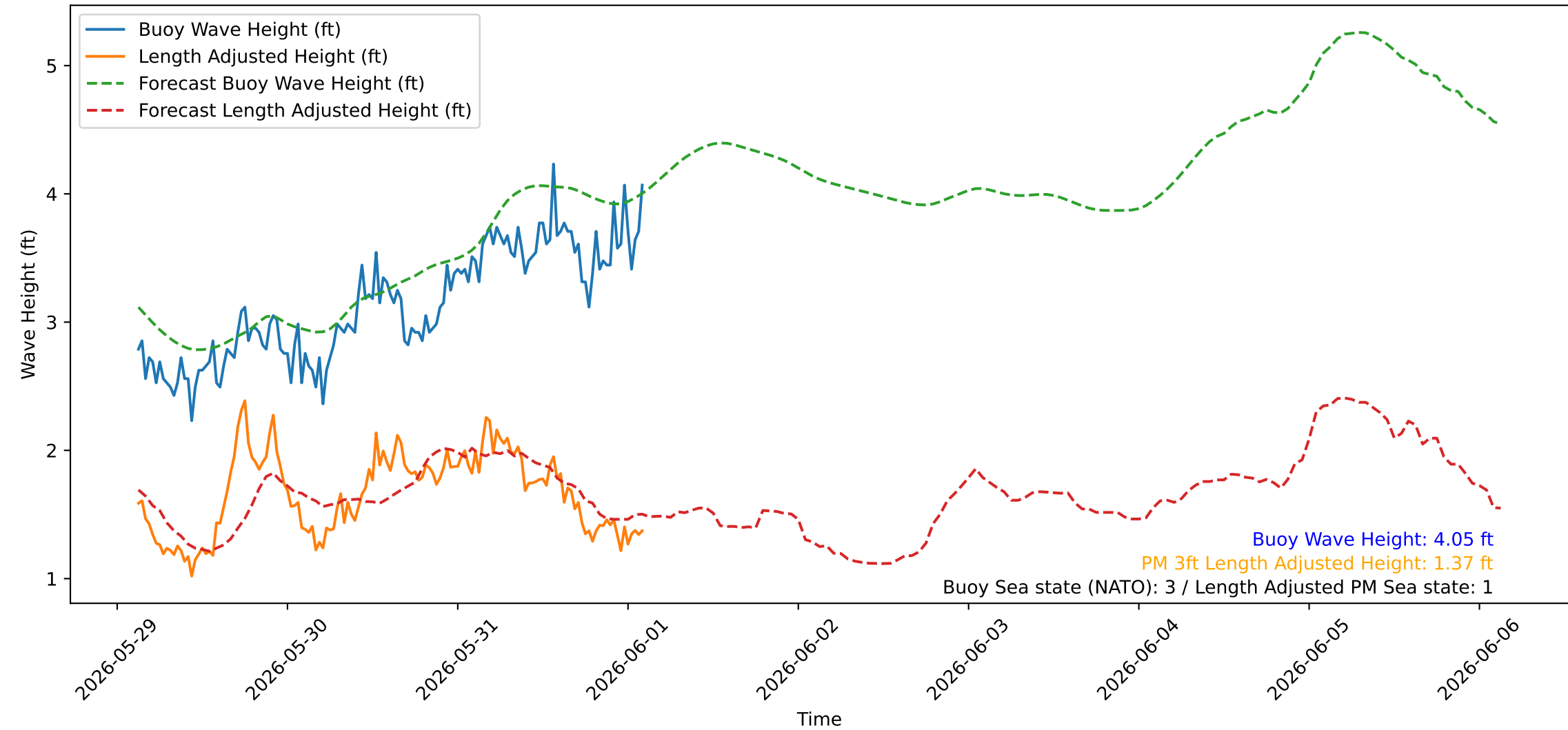
Wave Heights over Time for Oceanside Harbor at 2026-06-01 02:50:26
