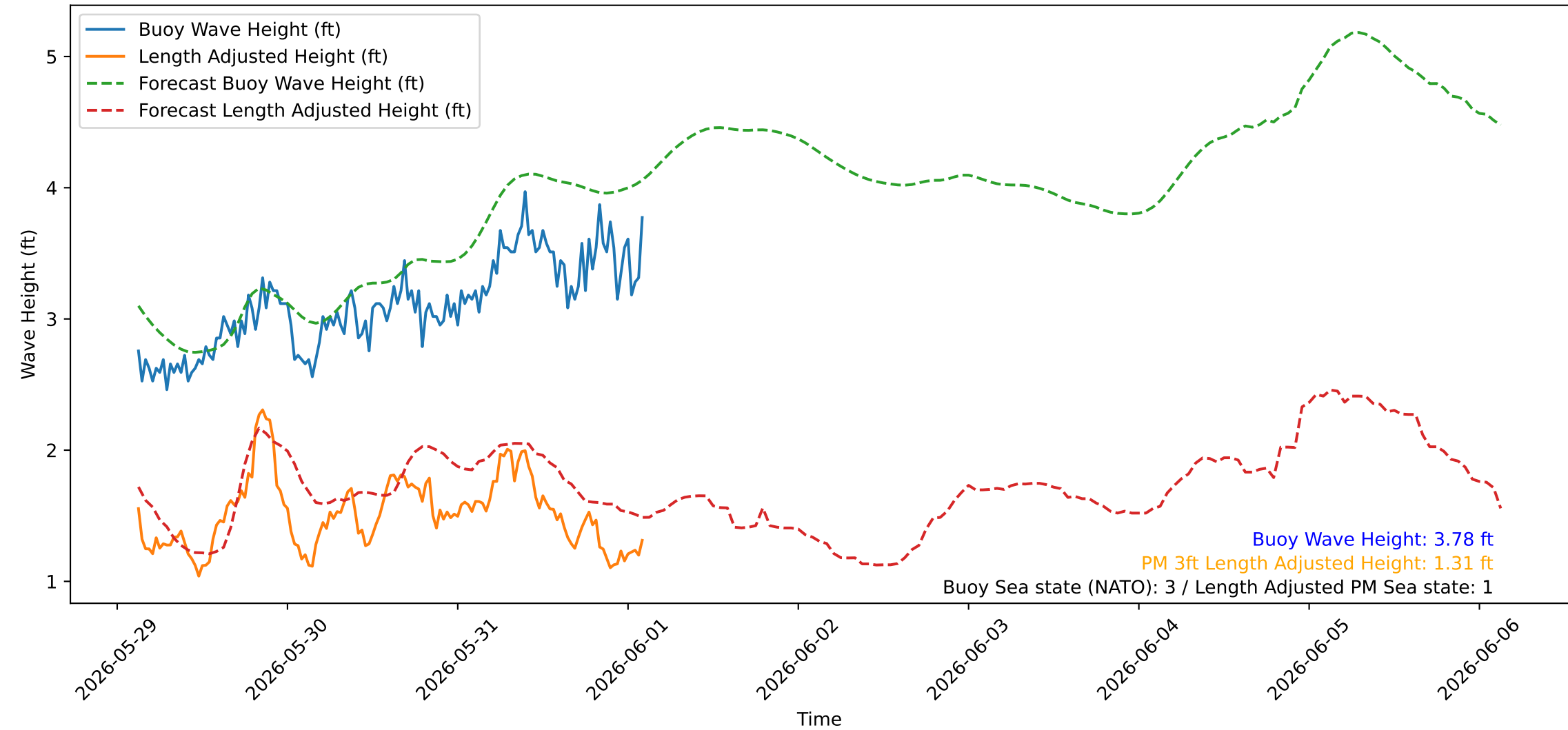
Wave Heights over Time for Green Beach at 2026-06-01 02:51:10
