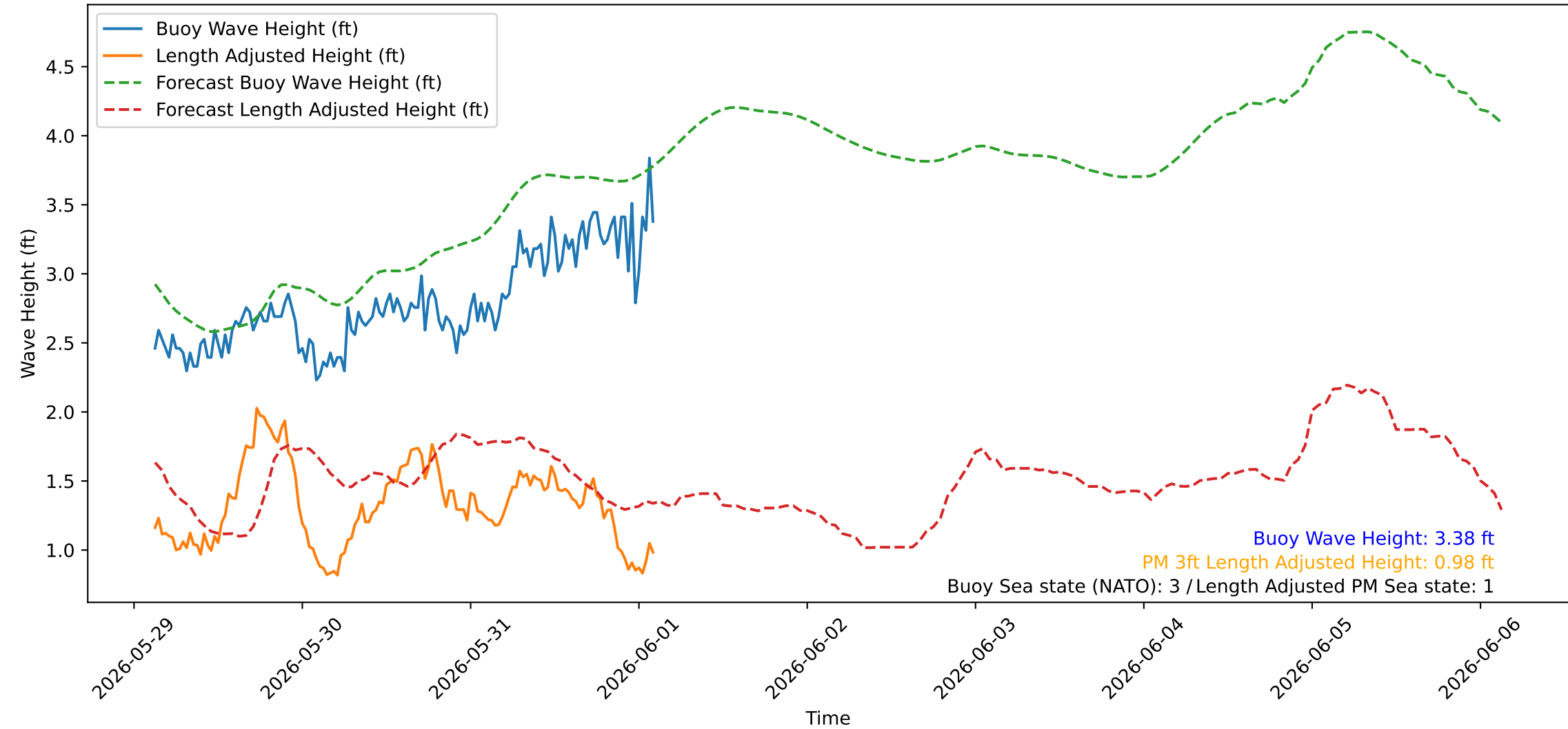
Wave Heights over Time for Red Beach at 2026-06-01 02:50:47
