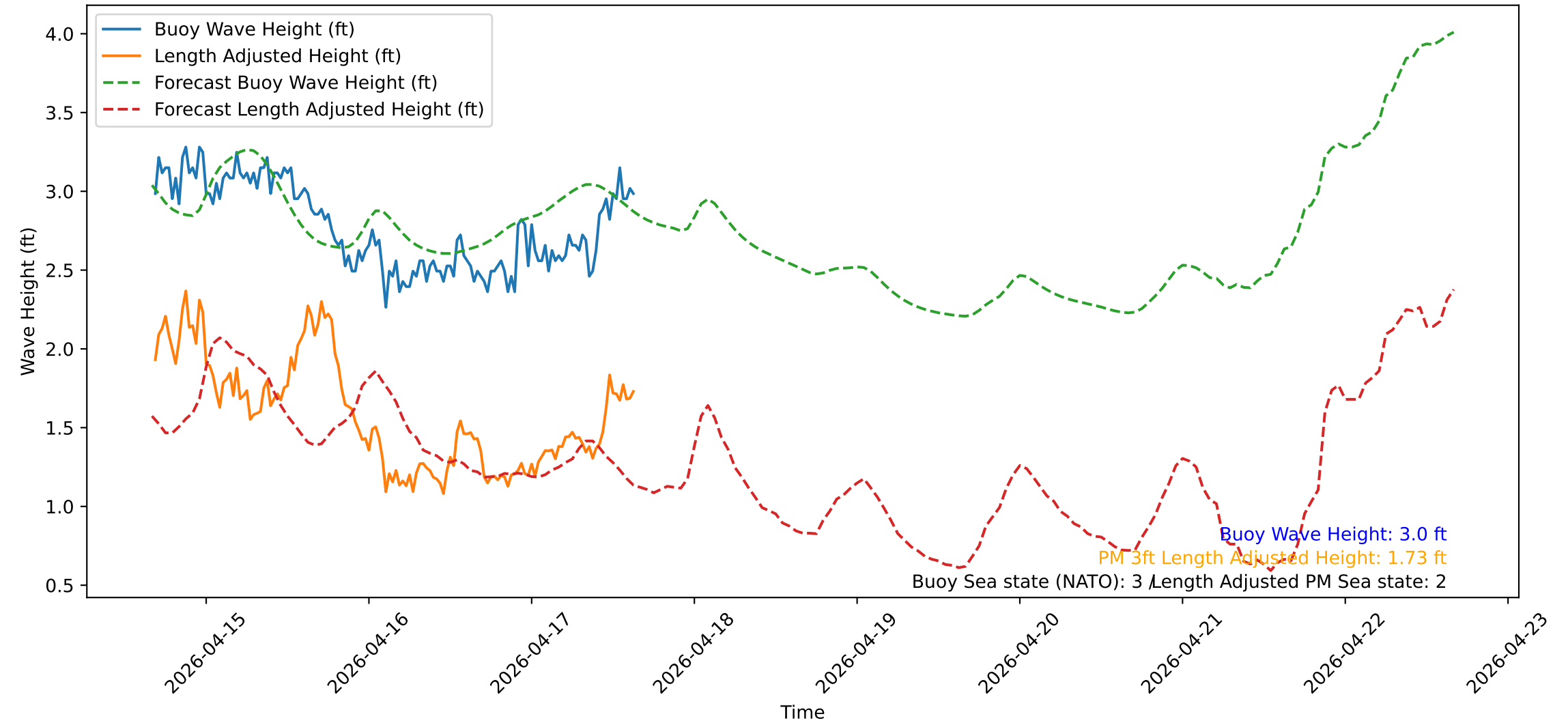
Wave Heights over Time for Red Beach at 2026-04-17 16:00:54
