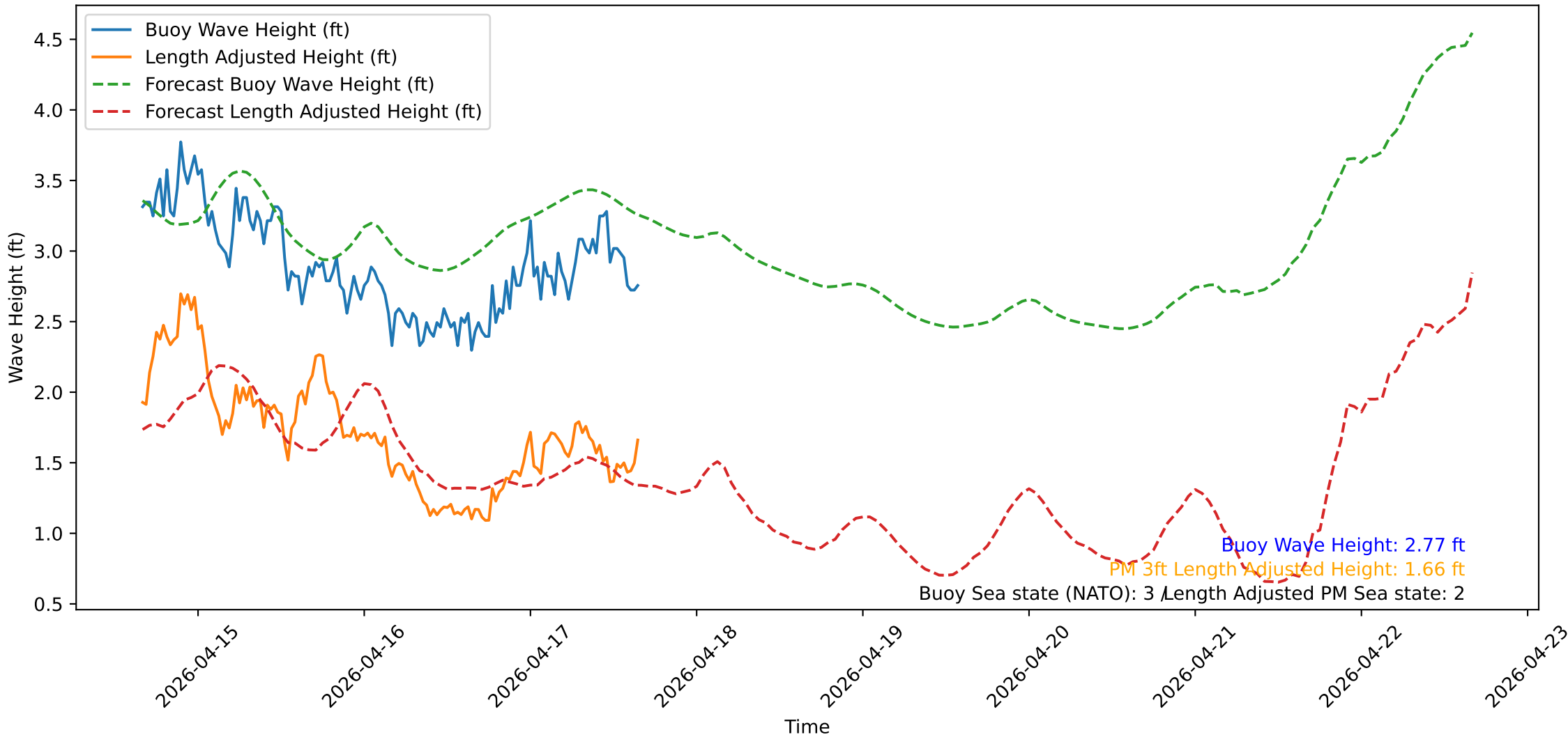
Wave Heights over Time for Oceanside Harbor at 2026-04-17 16:00:33
