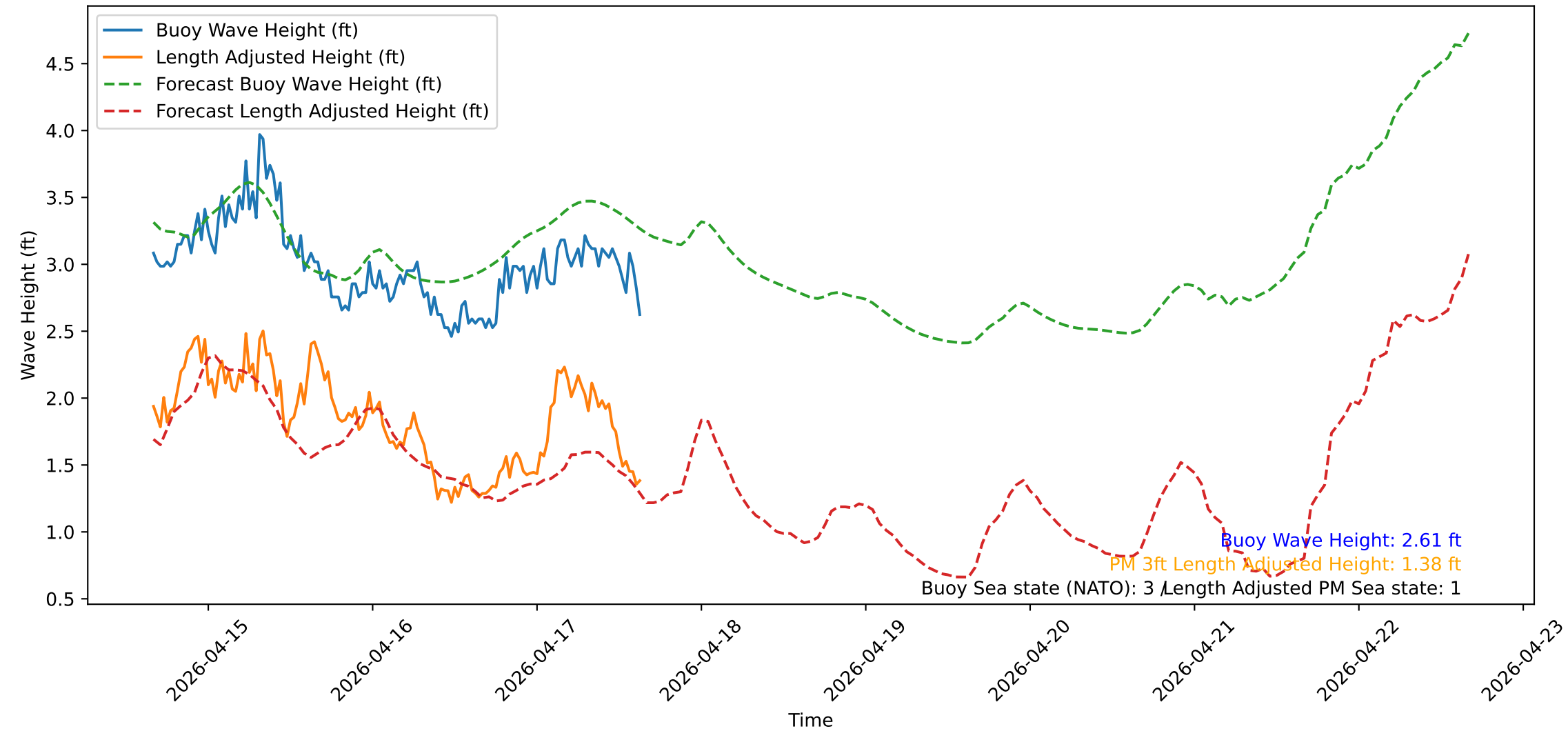
Wave Heights over Time for Green Beach at 2026-04-17 16:01:20
