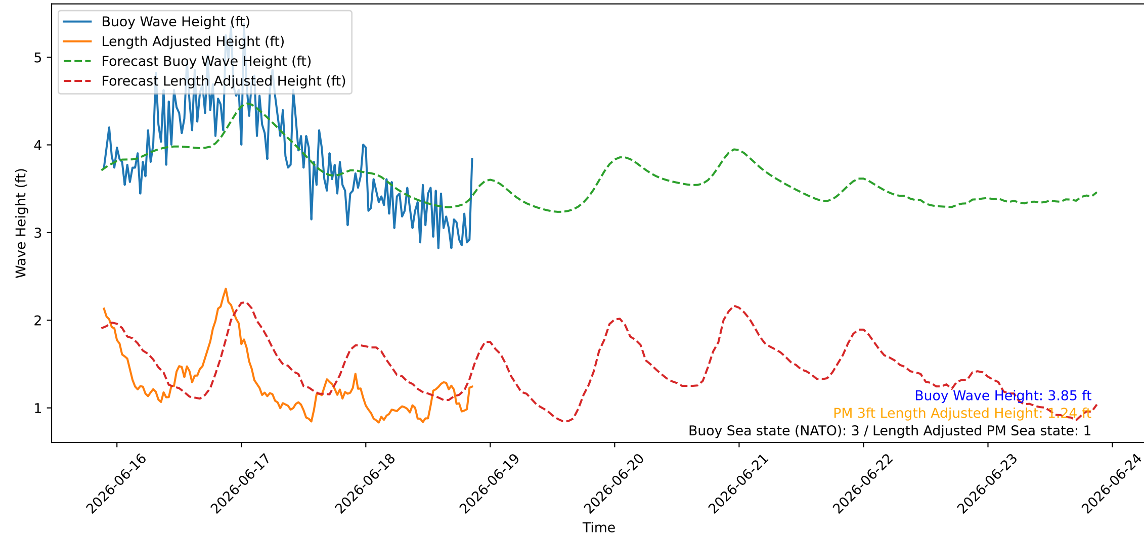
Wave Heights over Time for Red Beach at 2026-06-18 21:10:45
