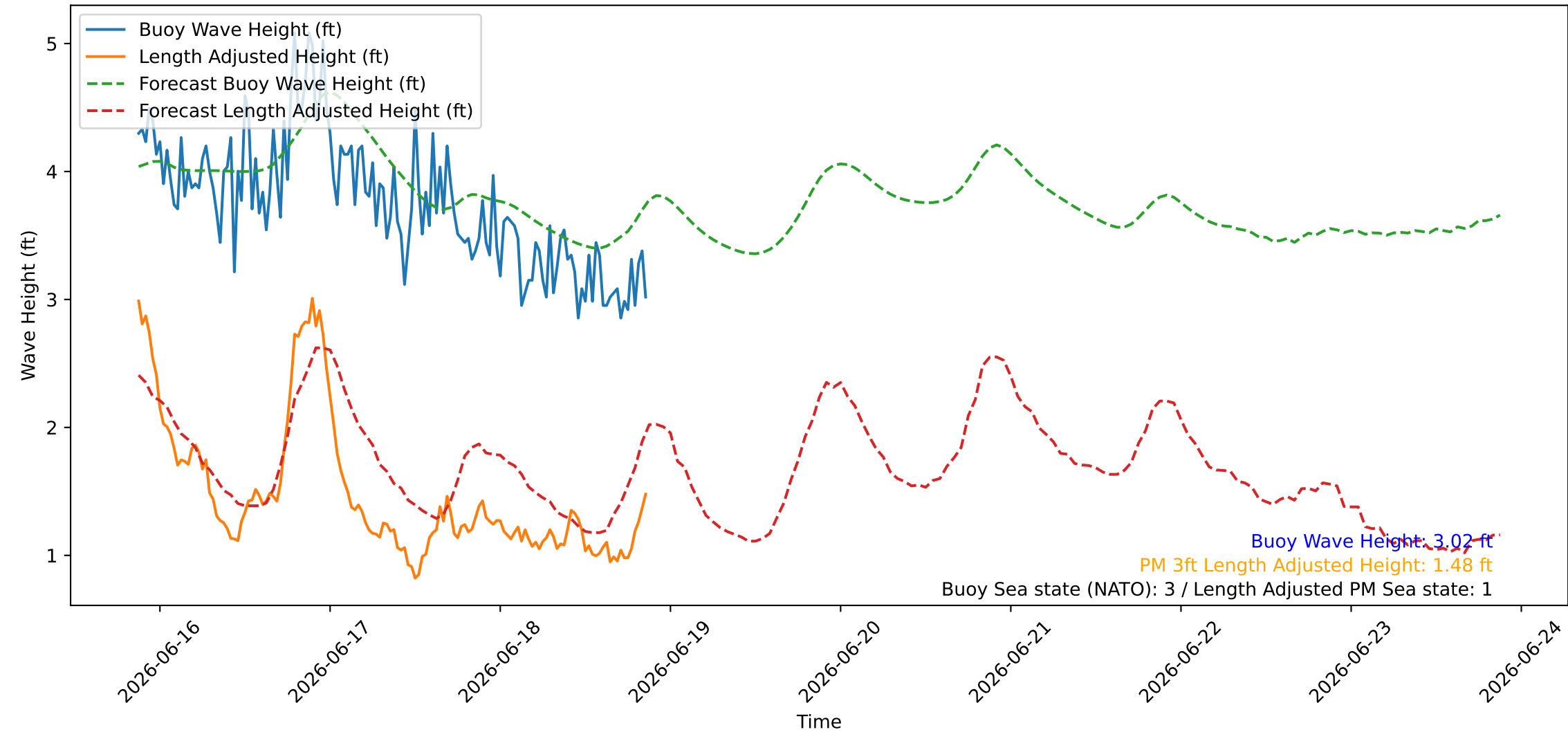
Wave Heights over Time for Green Beach at 2026-06-18 21:11:07
