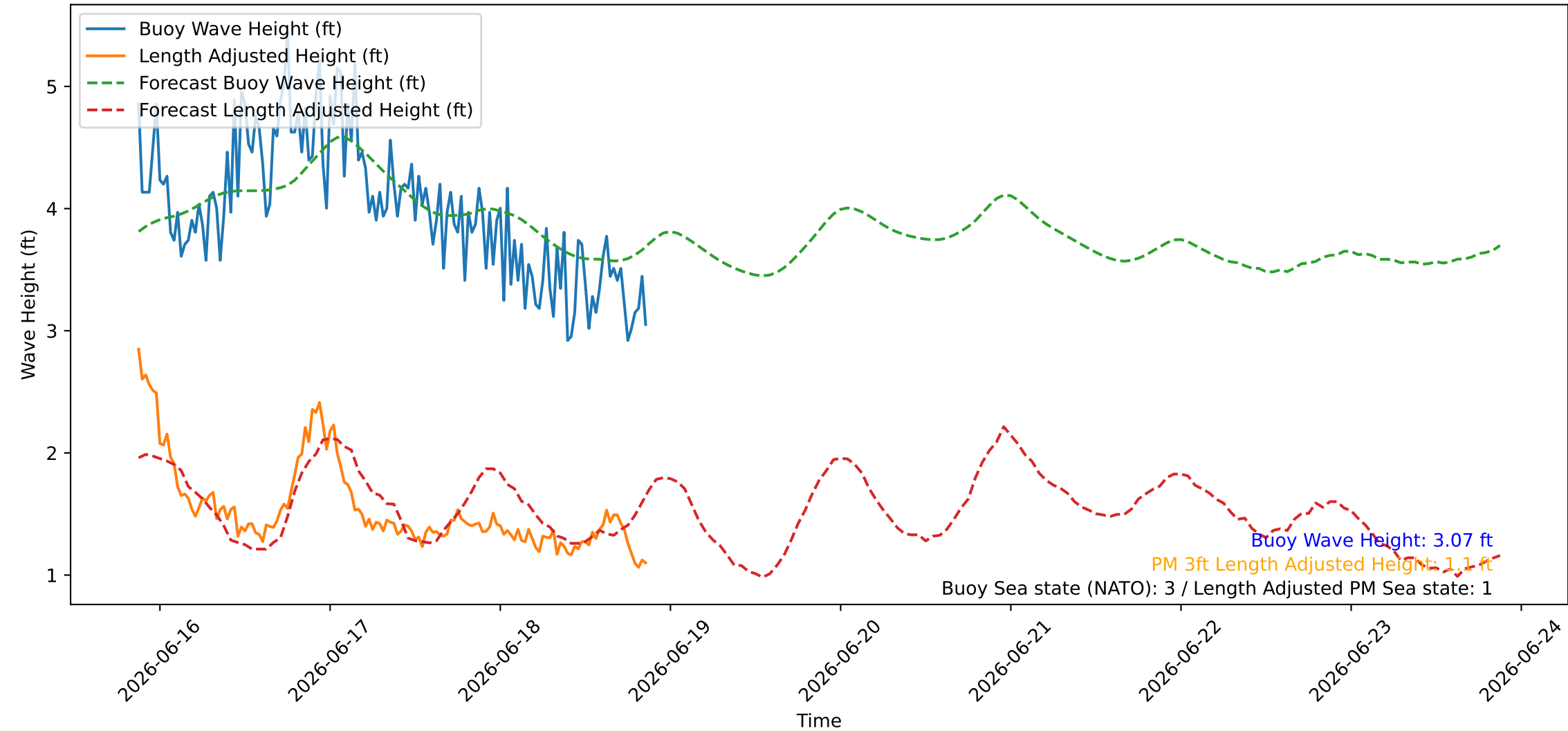
Wave Heights over Time for Oceanside Harbor at 2026-06-18 21:10:26
