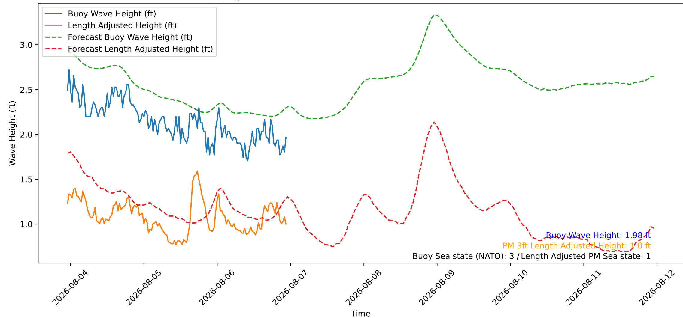
Wave Heights over Time for Oceanside Harbor at 2026-08-06 23:10:27
