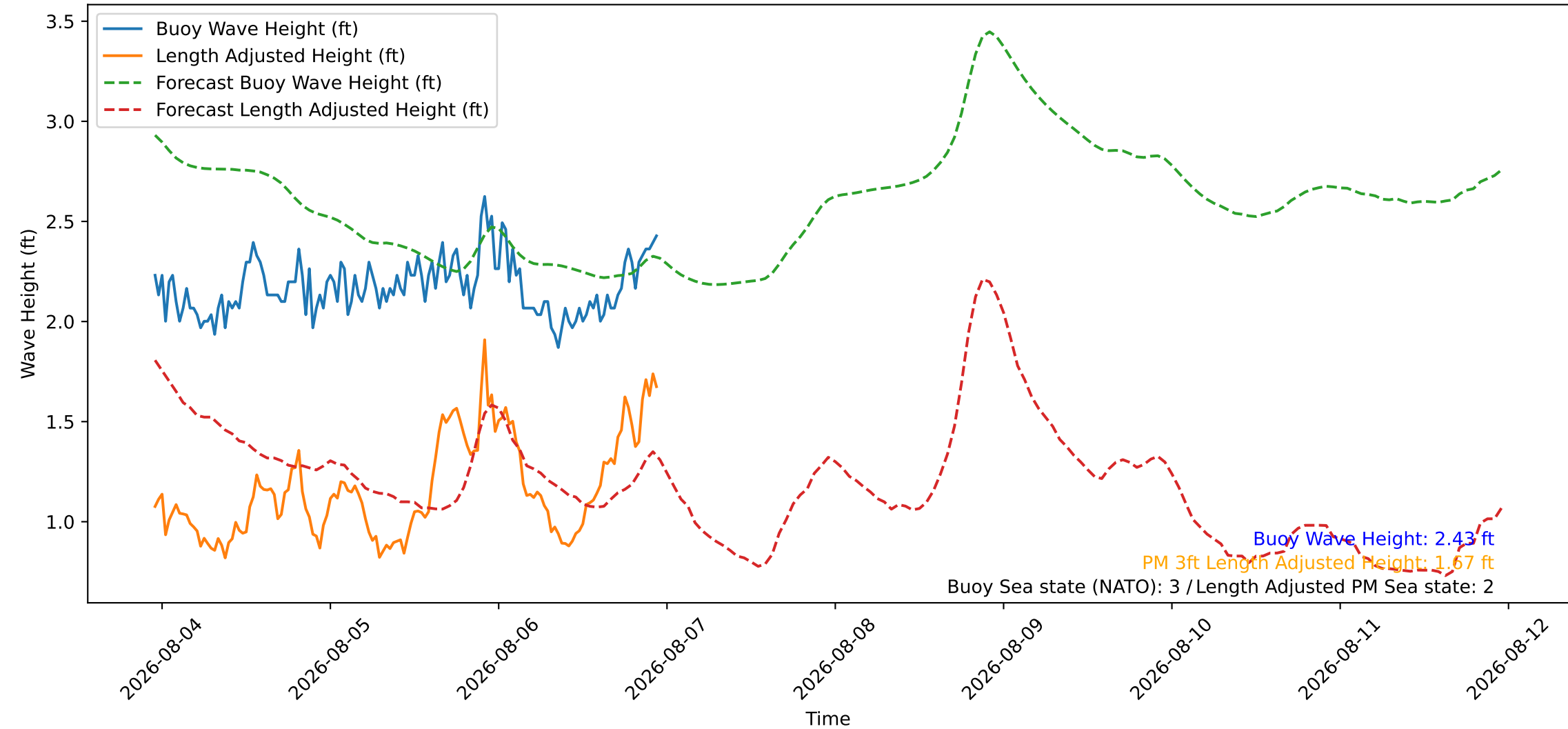
Wave Heights over Time for Green Beach at 2026-08-06 23:11:09
