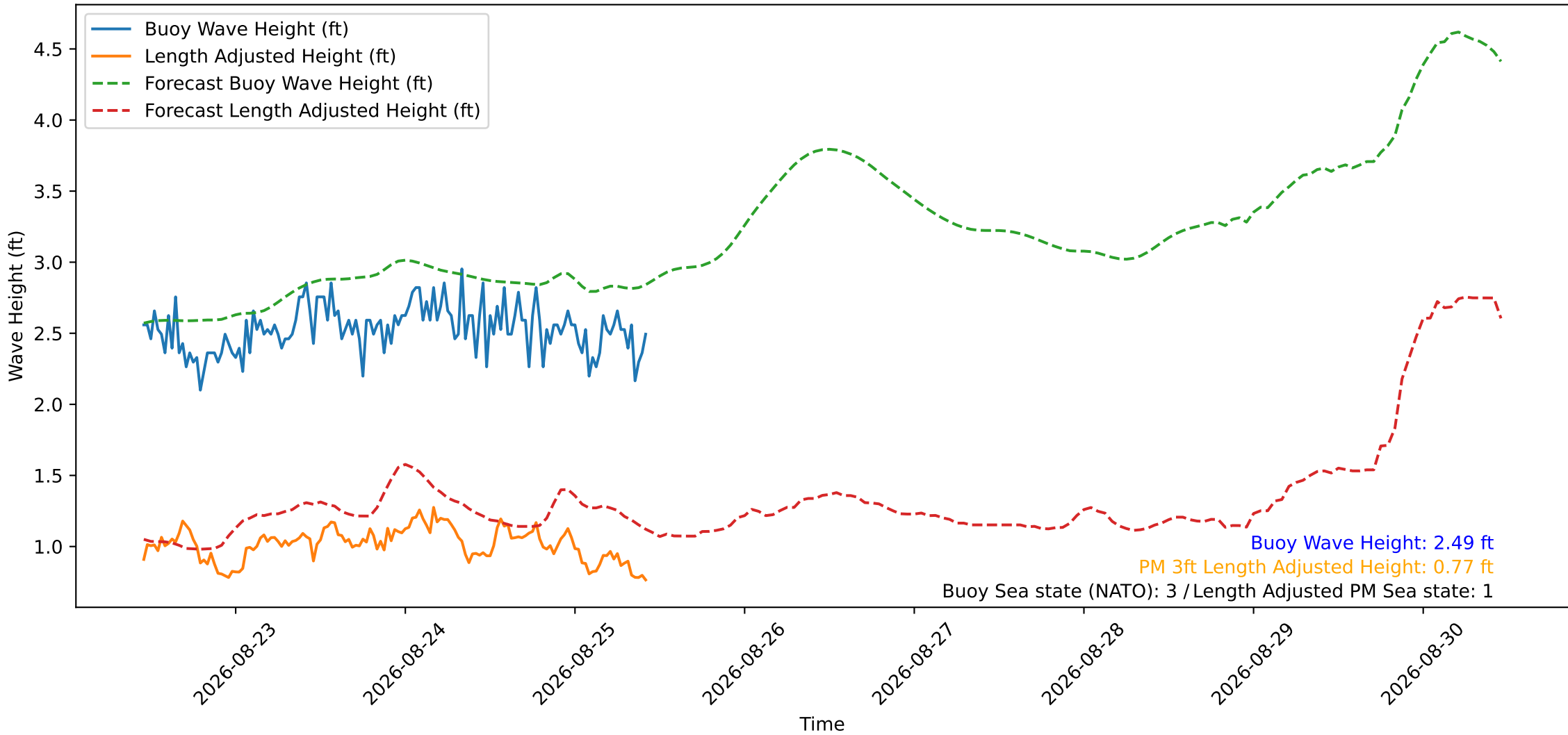
Wave Heights over Time for Red Beach at 2026-08-25 10:50:50
