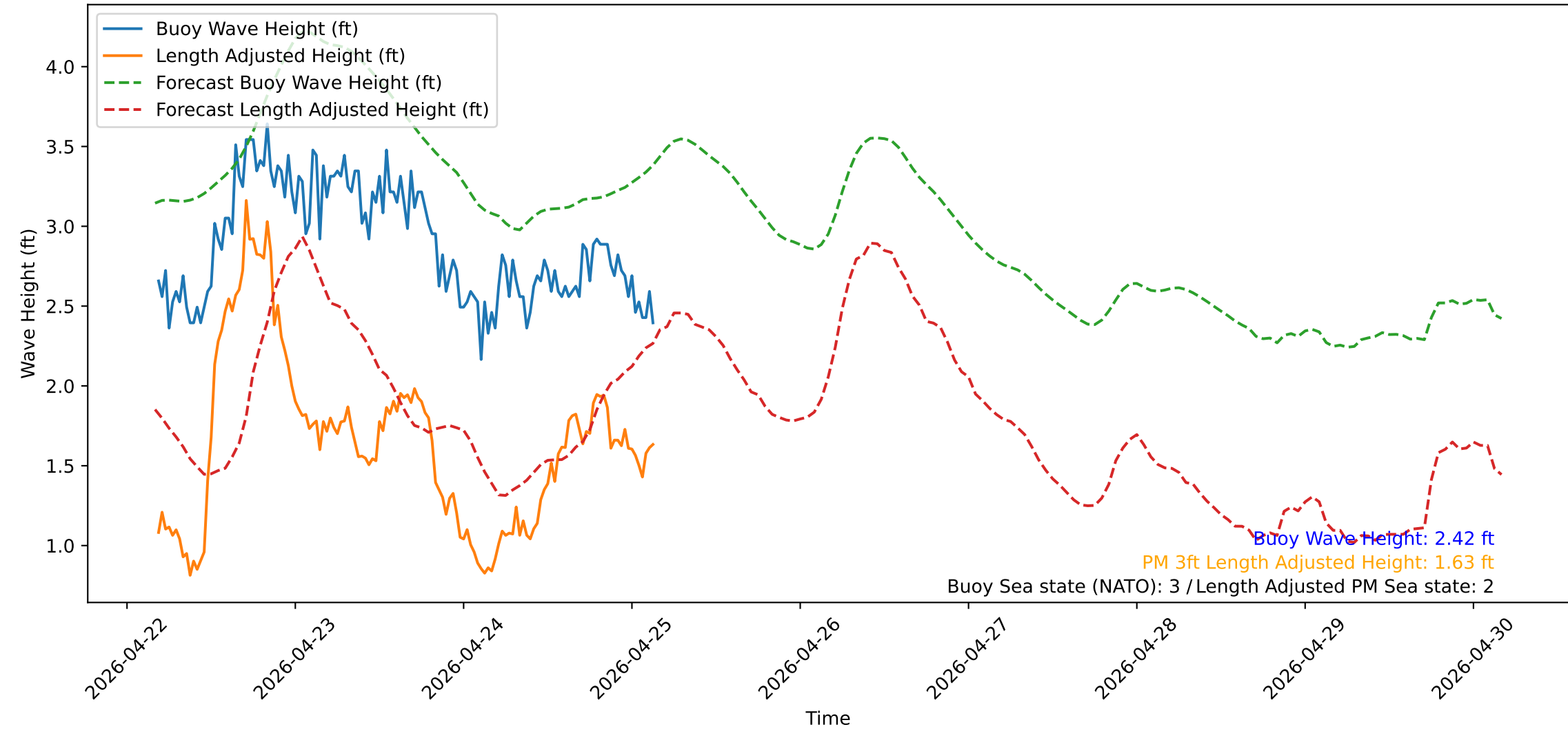
Wave Heights over Time for Red Beach at 2026-04-25 04:00:50
