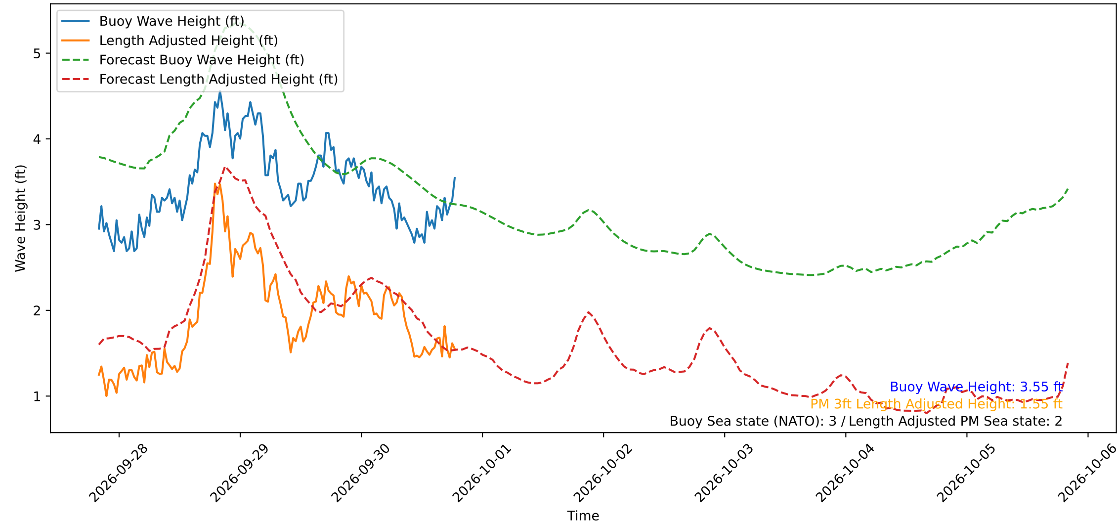
Wave Heights over Time for Green Beach at 2026-09-30 19:41:11
