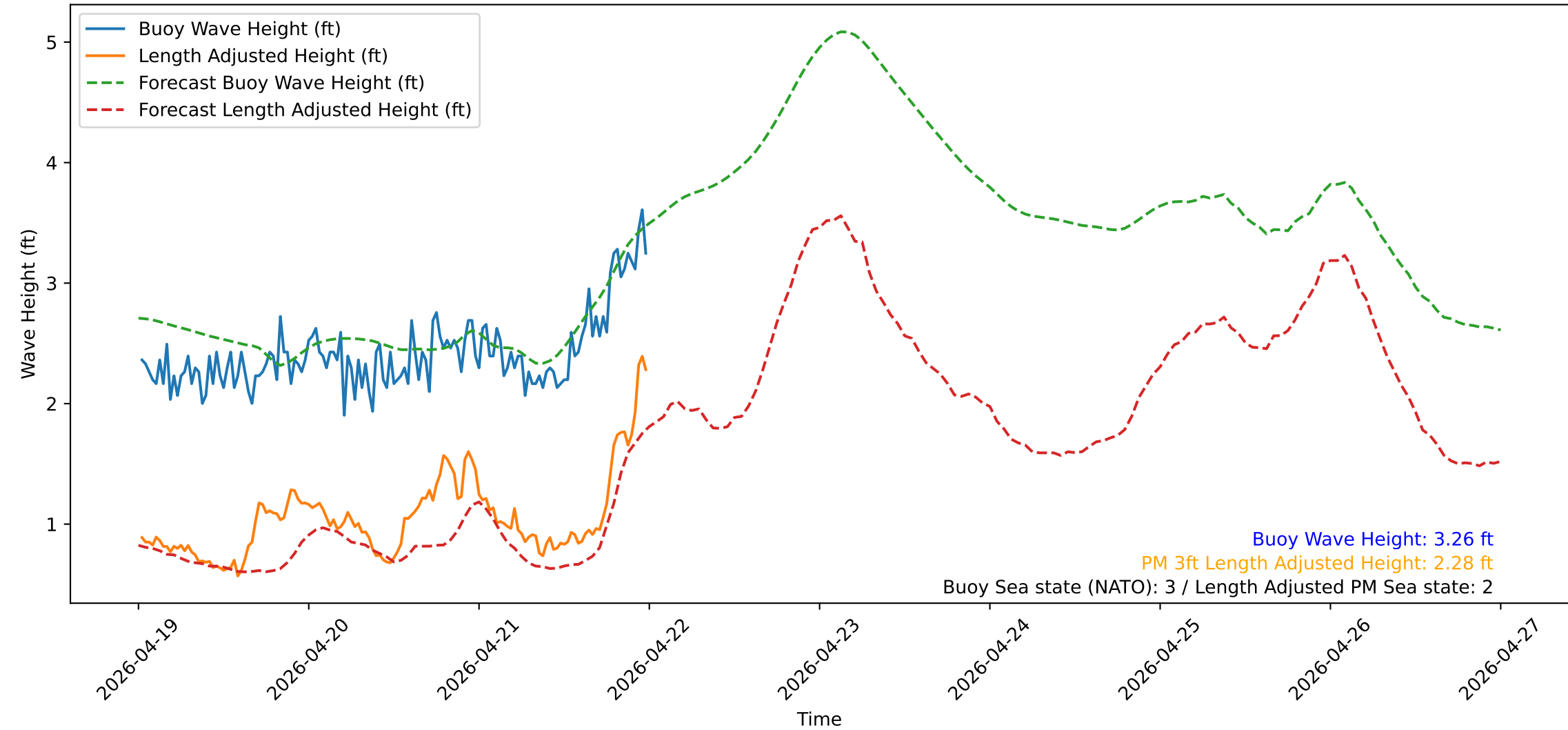
Wave Heights over Time for Oceanside Harbor at 2026-04-22 00:20:32
