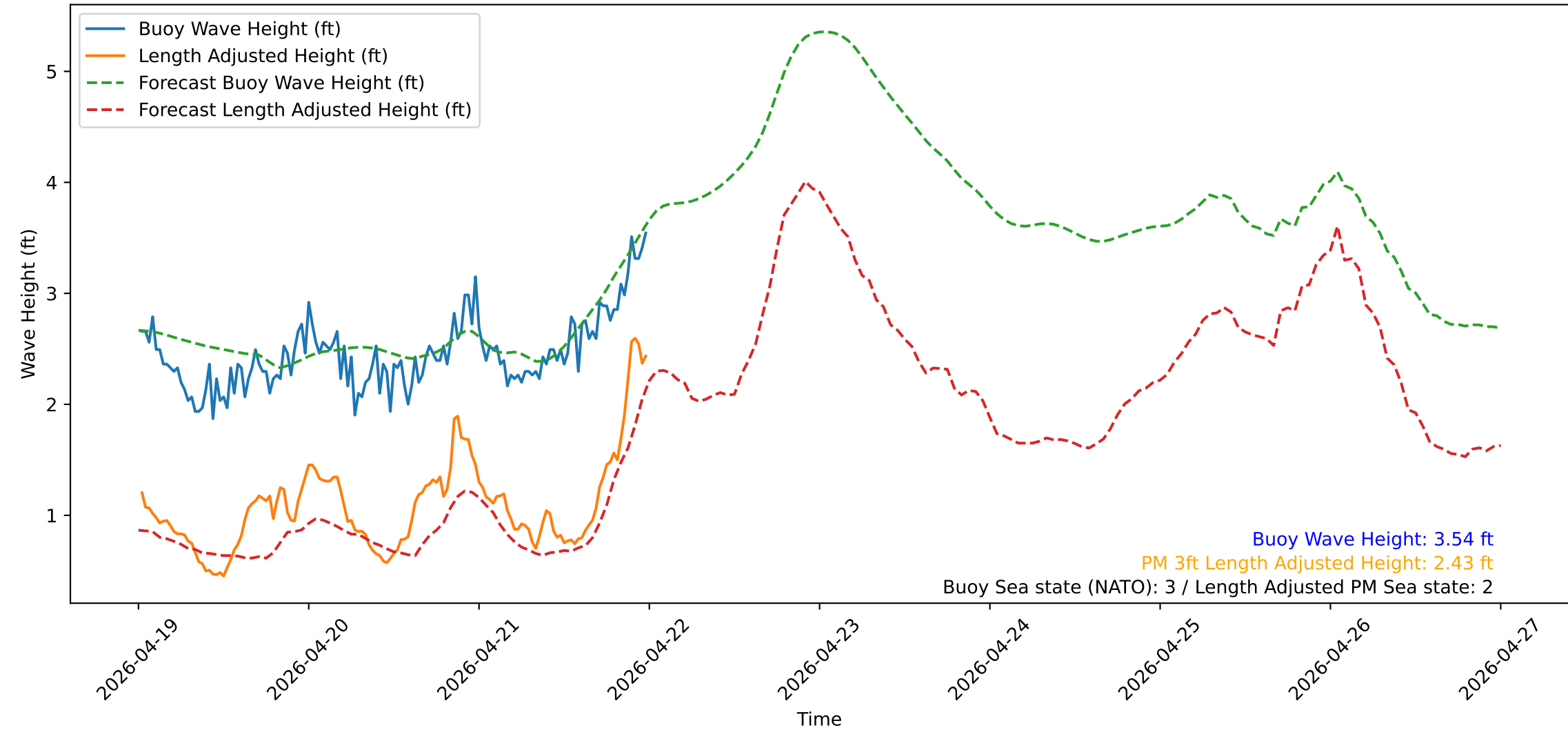
Wave Heights over Time for Green Beach at 2026-04-22 00:21:14
