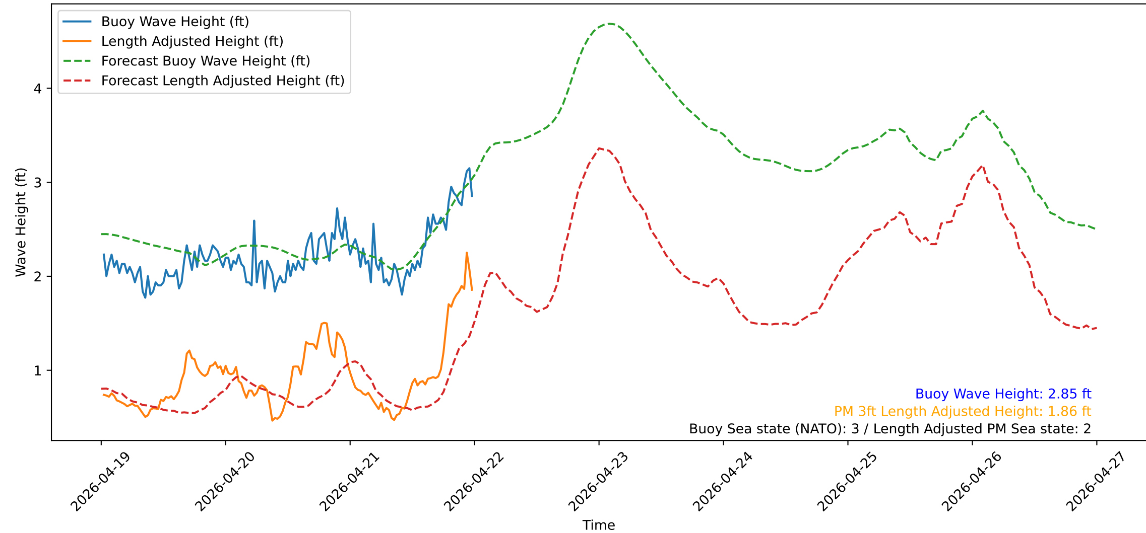
Wave Heights over Time for Red Beach at 2026-04-22 00:20:52
