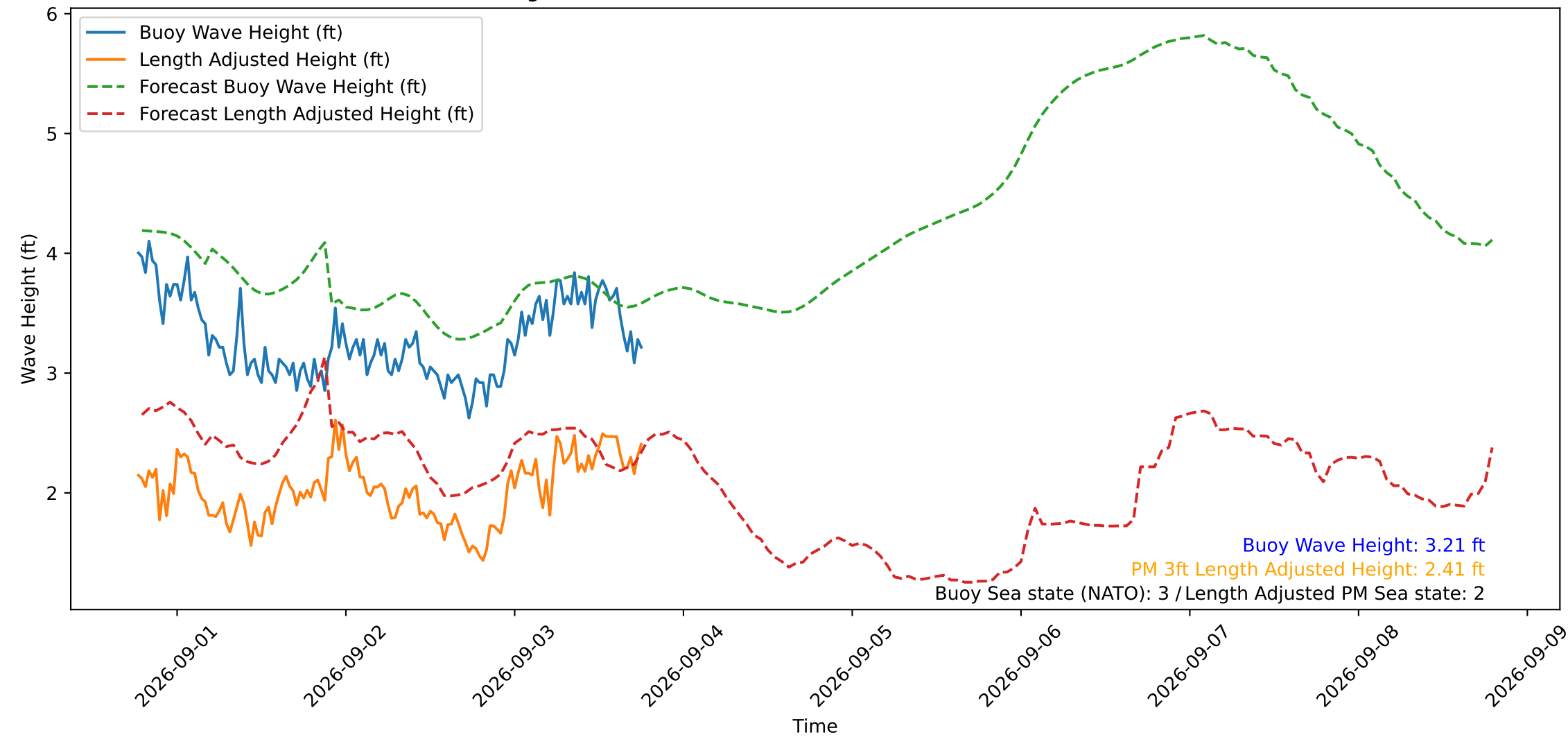
Wave Heights over Time for Oceanside Harbor at 2026-09-03 18:30:29
