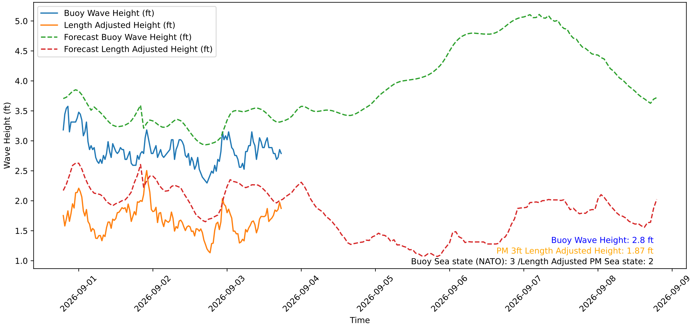
Wave Heights over Time for Red Beach at 2026-09-03 18:30:49
