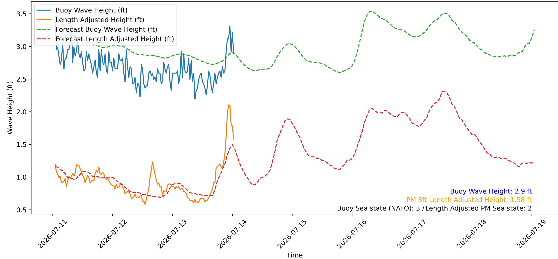
Wave Heights over Time for Green Beach at 2026-07-14 01:11:07
