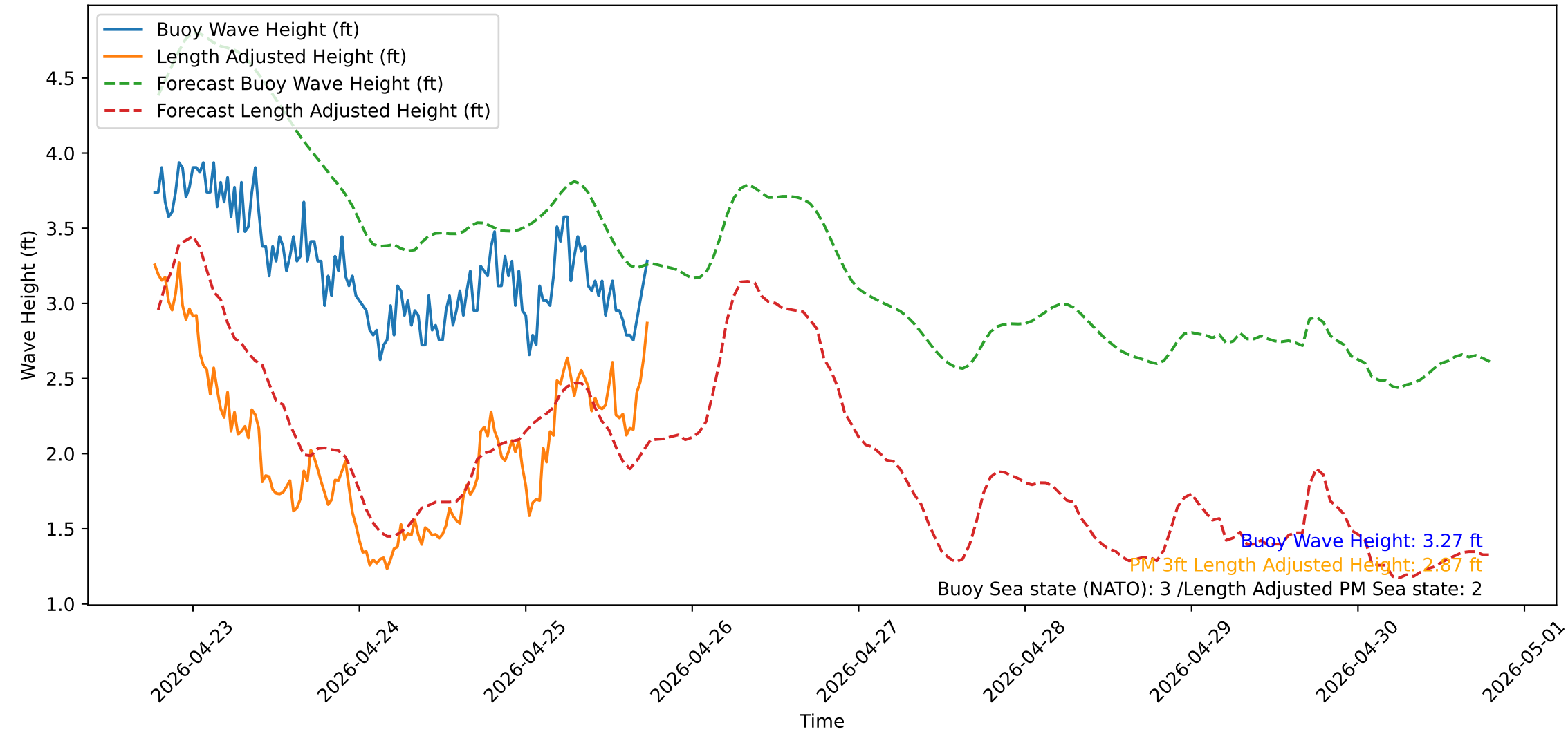
Wave Heights over Time for Green Beach at 2026-04-25 18:31:13
