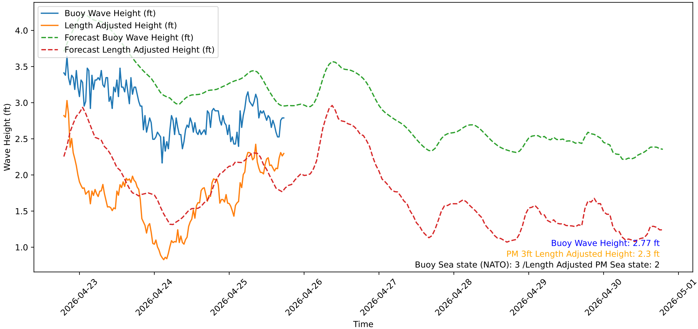
Wave Heights over Time for Red Beach at 2026-04-25 18:30:50
