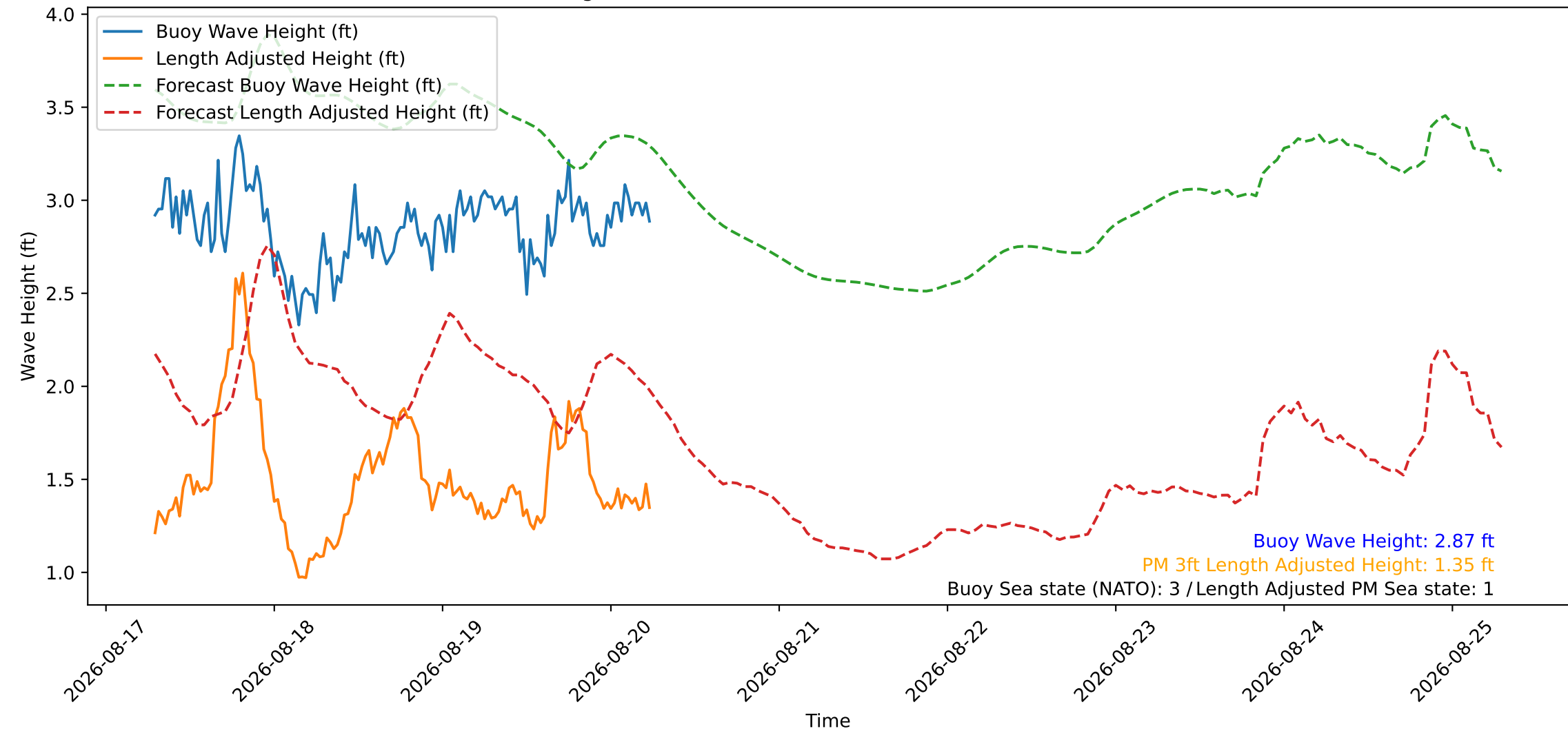
Wave Heights over Time for Red Beach at 2026-08-20 06:30:46
