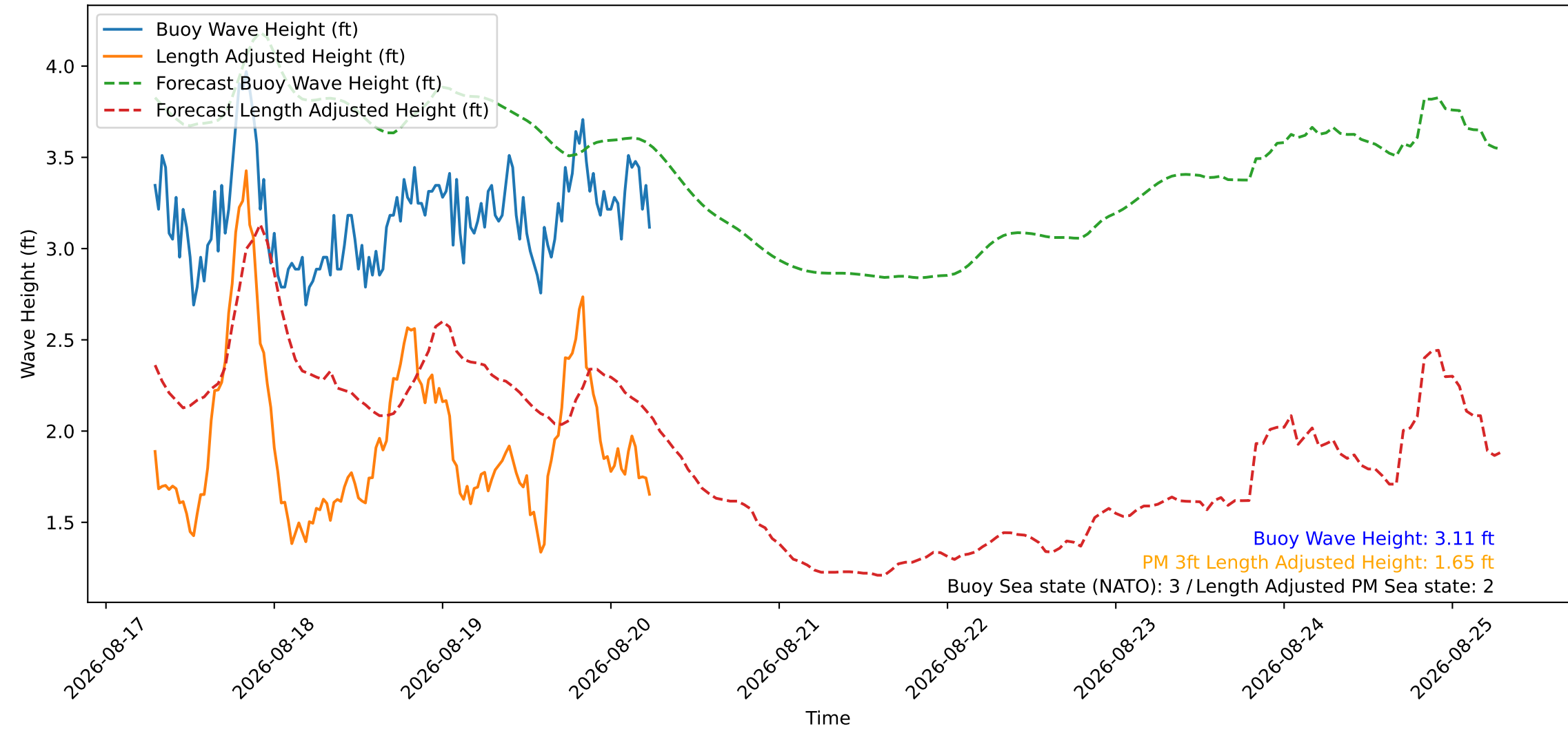
Wave Heights over Time for Green Beach at 2026-08-20 06:31:08
