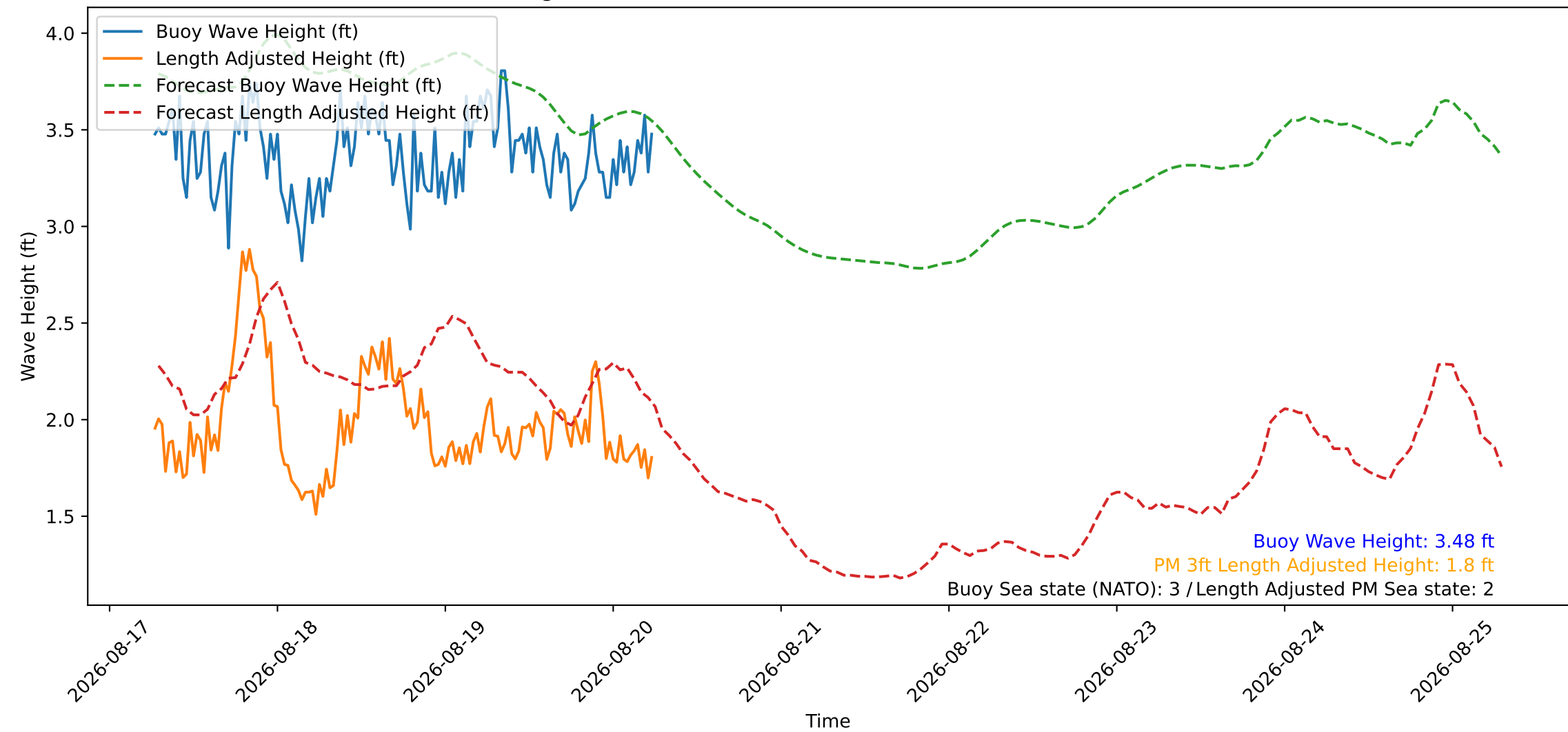
Wave Heights over Time for Oceanside Harbor at 2026-08-20 06:30:26
